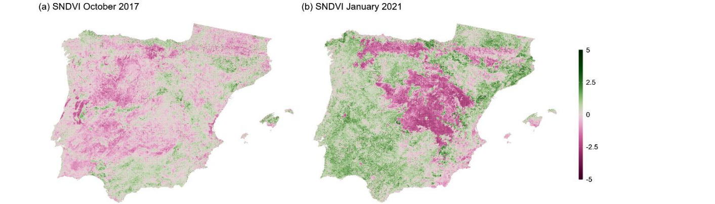
450 Figure 11. SNDVI from significant climatic events. Panel (a) shows the impact of the severe drought and wildfires on the Iberian Peninsula in October 2017, with notable vegetation stress indicated by standard deviation values below -3. Panel (b) presents SNDVI from the storm Filomena in January 2021, highlighting areas with unprecedented snowfall.
