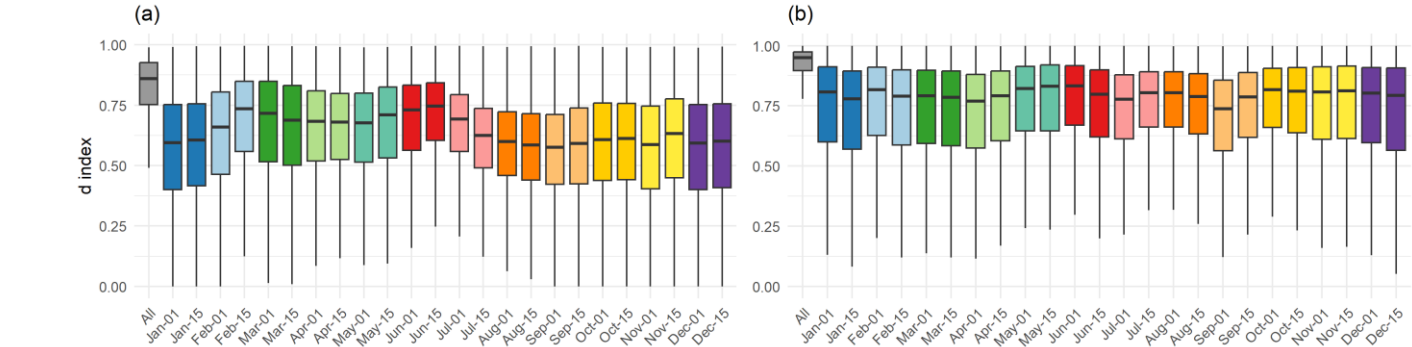
355 Figure 5. Distribution of Willmott’s d index values. Panel (a) shows the d index for harmonized AVHRR and MODIS NDVI data over the entire overlapping period, with median values ranging from 0.57 to 0.75, exhibiting seasonal variability. Panel (b) displays the d index for integrated AVHRR-MODIS and VIIRS NDVI data, with median values from 0.74 to 0.83, peaking in late spring and early summer.
