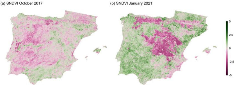
460 Figure 11. SNDVI from significant climatic events. Panel (a) shows the impact of the severe drought and wildfires on the Iberian Peninsula in October 2017, with notable vegetation stress indicated by standard deviation values below -3. Panel (b) presents SNDVI from the storm Filomena in January 2021, highlighting areas with unprecedented snowfall.
