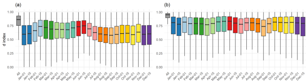
Figure 5. Distribution of Willmott's d index values. Panel (a) shows the d index for harmonized AVHRR and MODIS NDVI data over the entire overlapping period, with median values ranging from 0.57 to 0.75, exhibiting seasonal variability. Panel (b) displays the d index for integrated AVHRR-MODIS and VIIRS NDVI data, with median values from 0.74 to 0.83, peaking in late spring and early summer.
