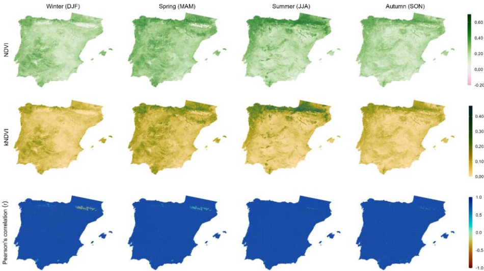
390 Figure 7. Spatial distribution of seasonal NDVI and kNDVI average for the period 1981 to 2024 and Pearson's correlation coefficient ( r ) between seasonal NDVI and kNDVI data.
