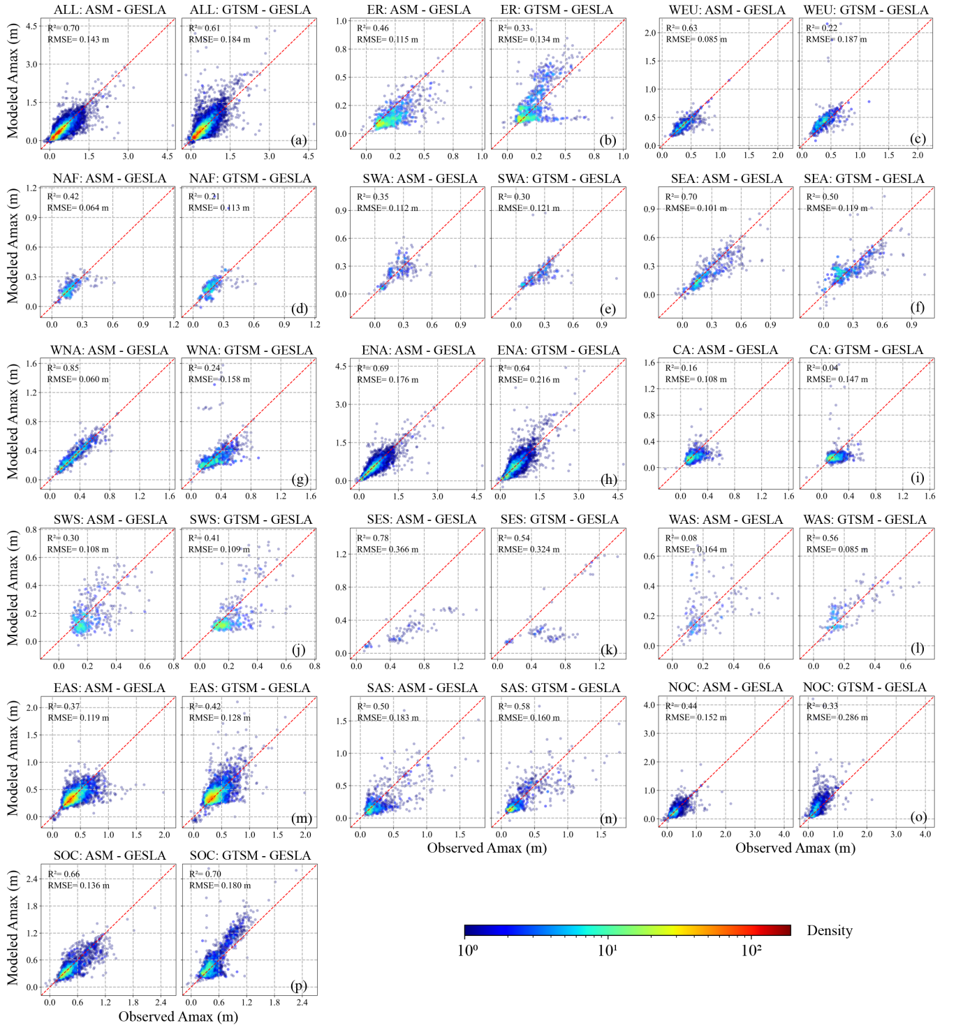
Figure 6: Scatter density plots of ASM and GTSM annual maxima (Amax) compared with tide gauge observations in different regions. The data for tide gauges were combined. The red dotted line indicates the perfect fit line.
