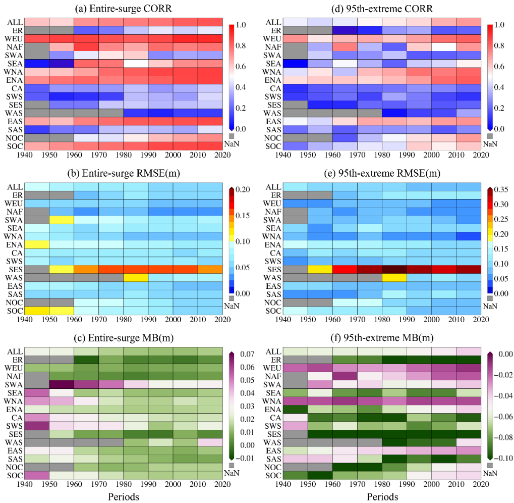
Figure 4: Temporal variations of the ASM model's precision at tide gauges from 1940 to 2020. (a-c) Entire surge evaluation statistics for different regions every 10 years; (d-f) 95th extreme evaluation statistics for different regions every 10 years
