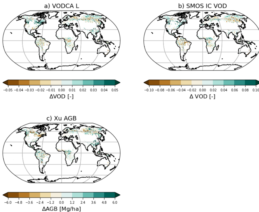
Figure 18. Difference between the years 2019 and 2011 for a) VODCA L and b) SMOS-IC VOD and c) Xu AGB (method of Araza et al. (2023) for reducing the inter-annual variability of the original time-series). The analysis is limited to forested areas.
