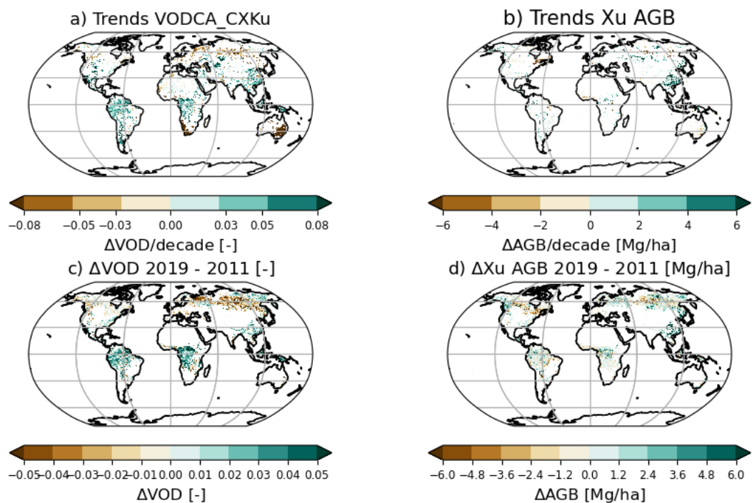
Figure A28. a) Theil-Sen trends for VODCA CXKu for 2011 - 2020. b) Theil-Sen trends for Xu AGB for the same period. Difference between the years 2019 - 2011 for c) VODCA CXKu and d) Xu AGB (method of Araza et al. (2023)).
