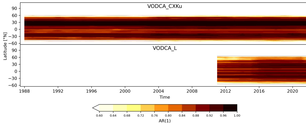
Figure 8. Hovmöller diagrams showing the yearly AC(1) per latitude for VODCA CXKu and VODCA L.
