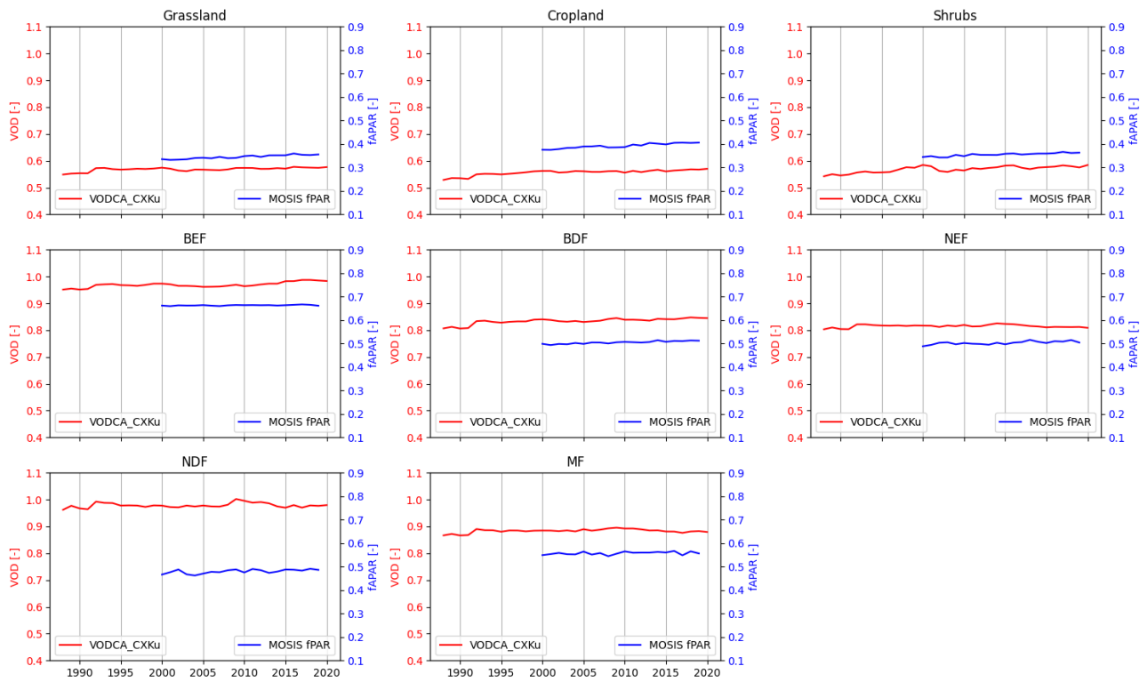
Figure A7. Yearly time-series per landcover class for VODCA CXKu and MODIS fAPAR. ESA CCI LC was used.
