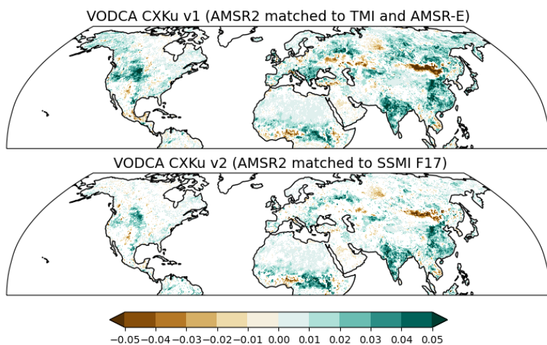
Figure 11. Trends (1987 - 2021) for VODCA CXKu v1 computed with the Moesinger et al. (2020) satellite constellation and CDF-matching framework, by merging AMSR2 to TMI below 35°N latitude and AMSR-E further north (top); and for VODCA CXKu v2 computed with the method from this paper, by matching AMSR2 to SSMI F17 (bottom). The same colorbar as in Fig. 10 (b) and (c) was used.
