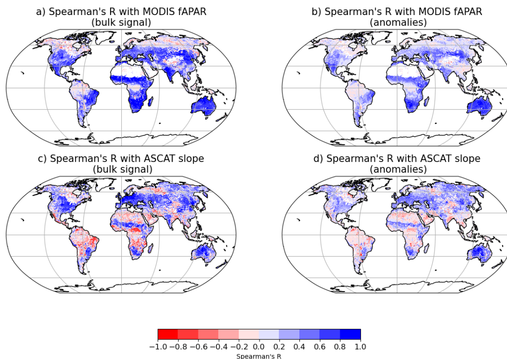
Figure 12. Spearman's R between 8-daily VODCA CXXu and MODIS fAPAR over the period 2000 - 2021 on the bulk signal (a) and anomalies (b). Spearman's R between 8-daily VODCA CXXu and ASCAT slope over the period 2007 - 2021 on the bulk signal (c) and anomalies (d).
