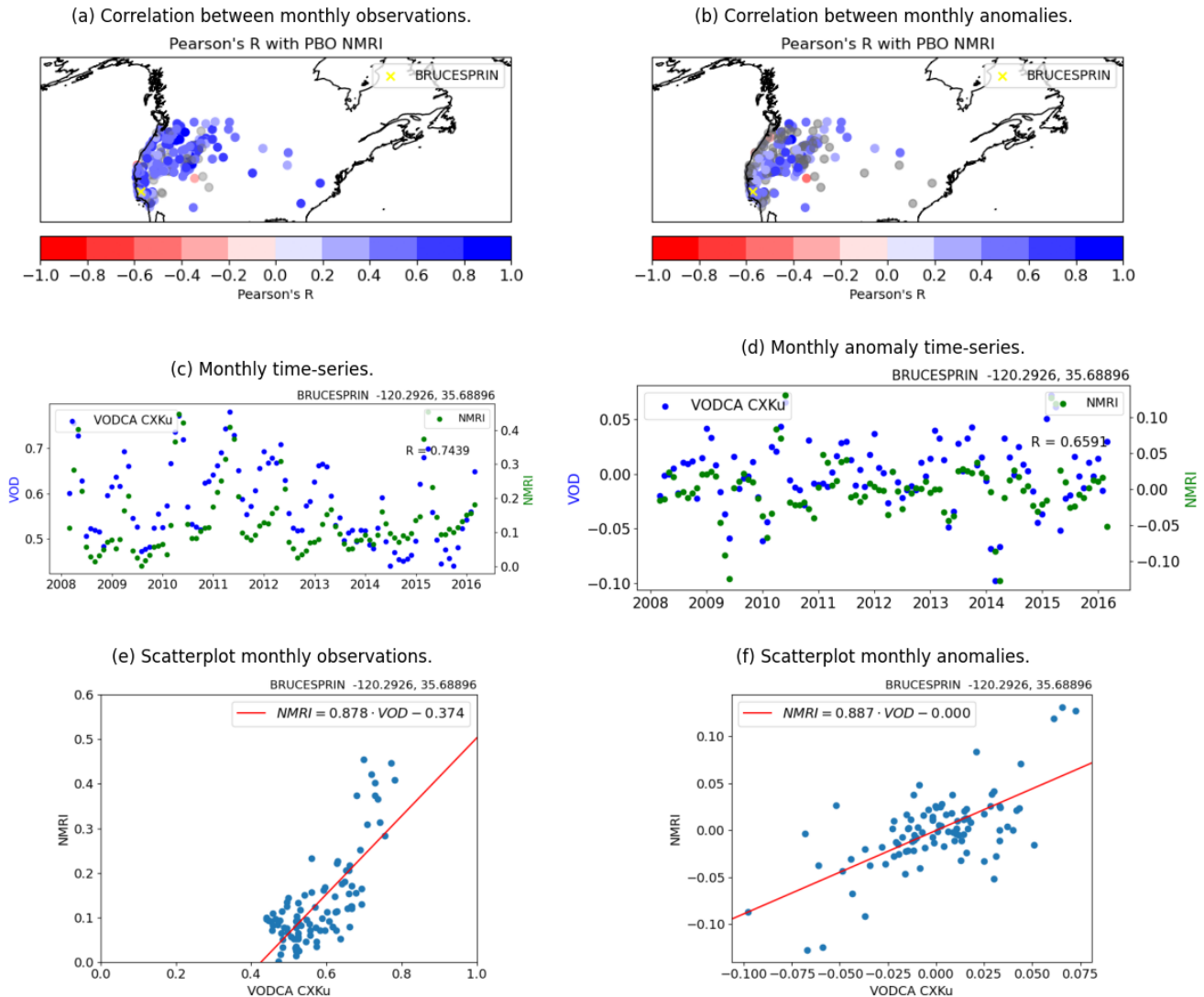
Figure 14. Pearson’s R between monthly VODCA CXKu and NMRI for the PBO stations over the bulk signal (a) and anomalies (b). The stations with non-significant correlations are shown in grey. time series over the bulk signal (c) and anomalies (d) of VODCA CXKu (blue) and PBO NMRI (green), as well as scatterplot over the bulk signal (e) and over anomalies (f) for a station with good agreement between datasets (BRUCESPRIN, lon -120.29, lat 35.68, indicated with a cross in the correlation maps).
