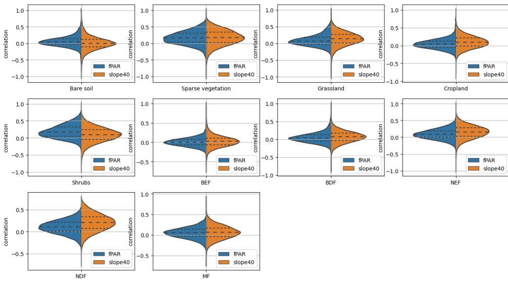
Figure A23. Violin plots showing the distribution of Spearman's R between monthly VODCA L and MODIS fPAR (blue) and VODCA L and ASCAT slope (orange) over anomalies, per landcover.
