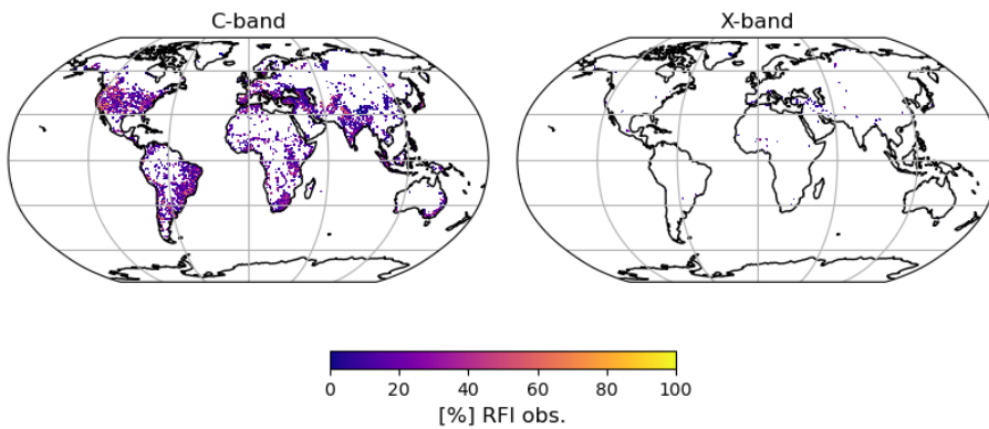
Figure A25. Percentage of observations affected by RFI in AMSR2 (2012 - 2021) C- and X-band. The internal flag provided with the LPRM data was used.
