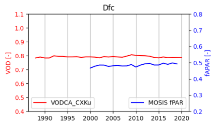
Figure A9. Yearly time-series for the Dfc climate, corresponding to boreal forest, for VODCA CXKu and MODIS fPAR.
