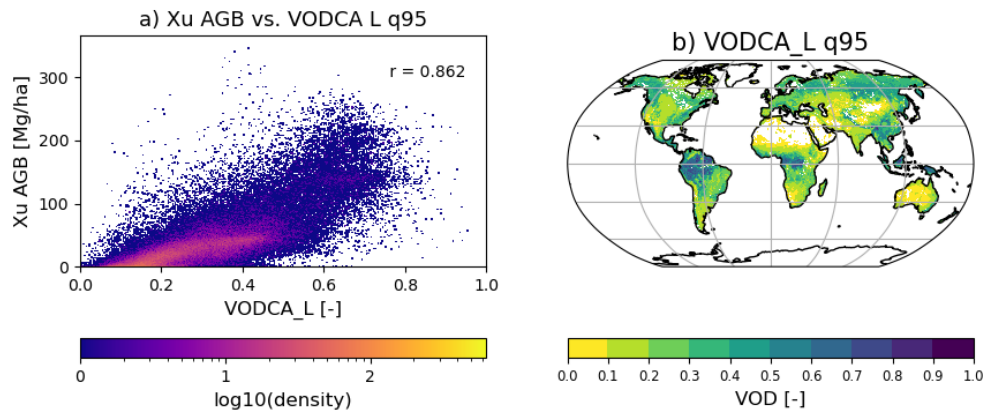
Figure 17. a) Temporal-spatial relationship between VODCA L q95 and Xu AGB over all overlapping years. The scatterplot is colored by the density of observations. Spearman's r is shown in the upper right side. (b) Median of VODCA L q95 of each year in 2010 - 2019.
