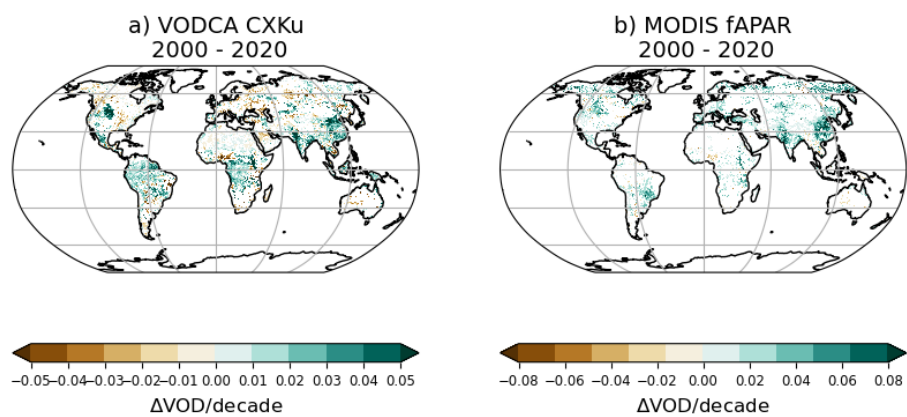
Figure A18. Trends for the overlapping period (February 2000 - August 2020) for a) VODCA CXKu and b) fAPAR.
