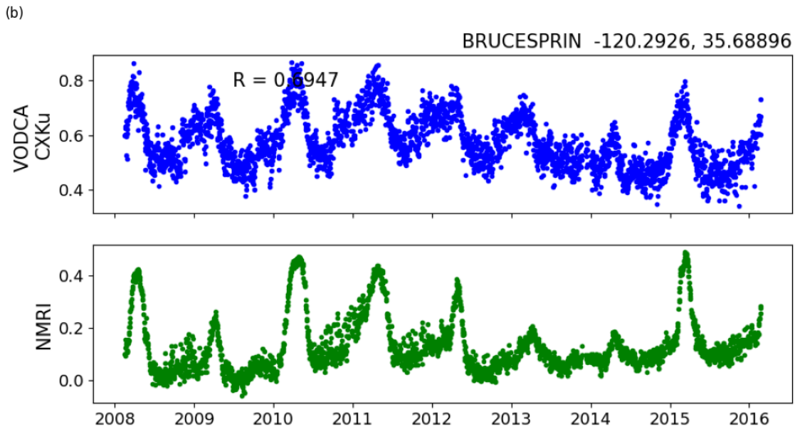
Figure A26. (a) Pearson's R between daily VODCA CXKu and NMRI for each PBO station. Only sites with significant correlation are shown. (b) time series of VODCA CXKu (blue) and PBO NMRI (green) for a station with above average agreement between datasets.
