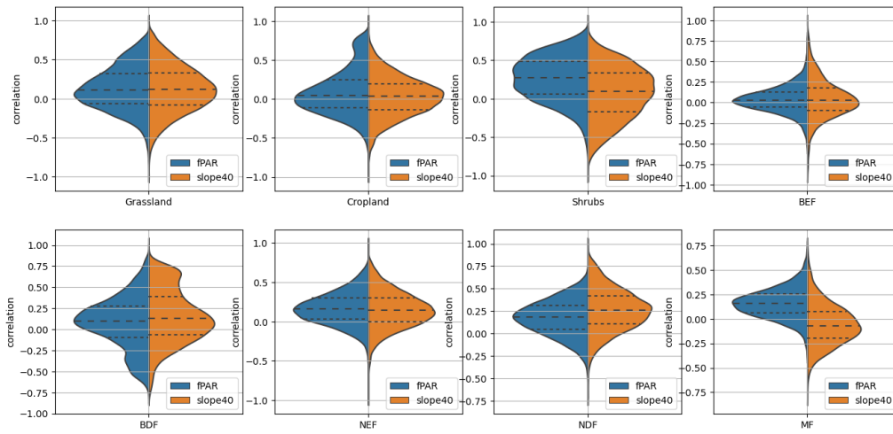
Figure A22. Violin plots showing the distribution of Spearman's R between monthly VODCA L and MODIS fPAR (blue) and VODCA L and ASCAT slope (orange) on the bulk signal, per landcover.
