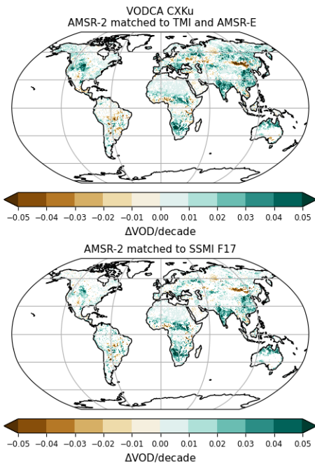
Figure A19. Trends (1987 - 2021) for VODCA CXXKu computed with the Moesinger et al. (2020) satellite constellation and CDF-matching framework, by merging AMSR2 to TMI below 35°N latitude and AMSR-E above; and for VODCA CXXKu computed with the method from this paper, by matching AMSR2 to SSMI F17
