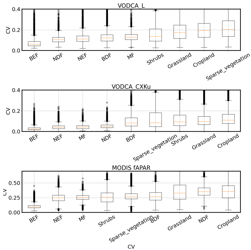
Figure A16. Coefficient of variation per LC for VODCA L, VODCA CXKu and fAPAR. ESA CCI LC was used.
