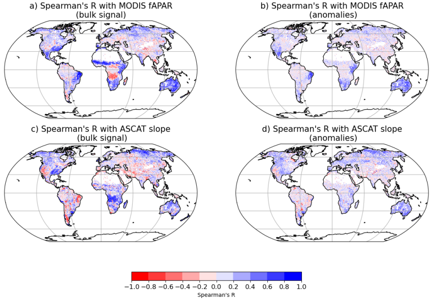
Figure A21. Spearman's R between monthly VODCA L and MODIS fAPAR over the period 2010 - 2021 on the bulk signal (a) and anomalies (b). Spearman's R between monthly VODCA L and ASCAT slope over the period 2010 - 2021 on the bulk signal (c) and anomalies (d).
