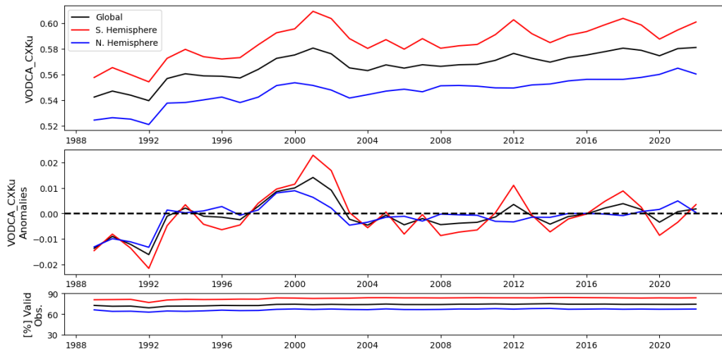
Figure 5. Global and hemisphere time-series of yearly VODCA CXXKu showing the bulk signal (upper part), detrended anomalies (middle part) and percentage of valid observations (lower part).
