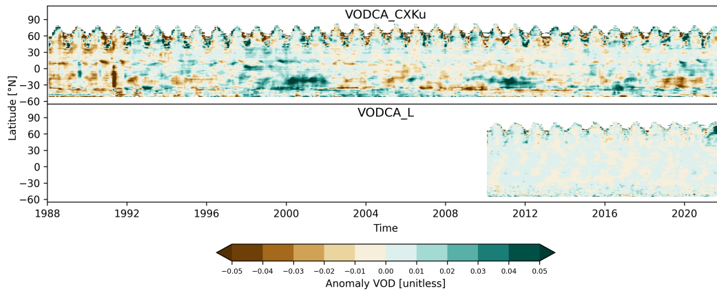
Figure A5. Hovmöller diagrams showing anomalies of the monthly means per latitude for VODCA CXXKu and VODCA L. Anomalies have been computed as deviations from the climatology of the periods 1990 - 2020 (VODCA CXXKu) and 2010 - 2021 (VODCA L).
