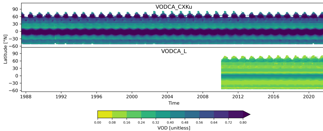
Figure 7. Hovmöller diagrams showing the monthly mean VOD per latitude for VODCA CXKu and VODCA L.
