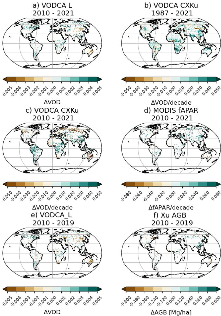
Figure 10. Trends over the entire product period calculated with the Theil-Sen regressor for VODCA L (a) and VODCA CXKu (b). Trends for the overlapping period 2010 - 2021 for VODCA CXKu (c) and MODIS fAPAR (d). Trends for the overlapping period 2010 - 2019 for VODCA L (e) and Xu AGB (f). Trends are considered not significant and masked when the upper and lower confidence intervals have conflicting signs.
