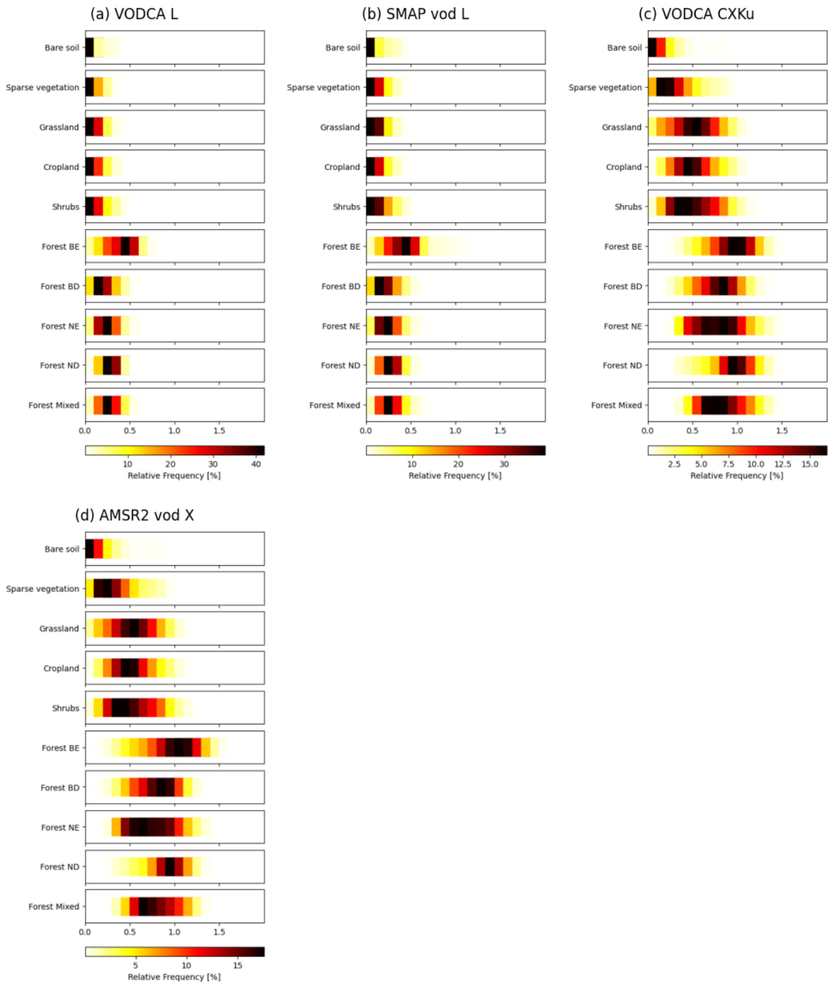
Figure A15. Values ranges per LC class for VODCA L (a), SMAP vod L (b), VODCA CXKu (c) and AMSR2 vod X (d). Bins are colored by the relative frequency in percent of the respective values. ESA CCI LC was used.
