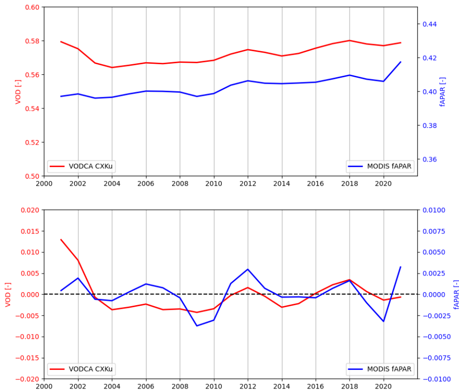
Figure A6. Yearly global time-series of VODCA CXXKu and fAPAR for the bulk signal (upper graphic) and for anomalies (lower graphic).
