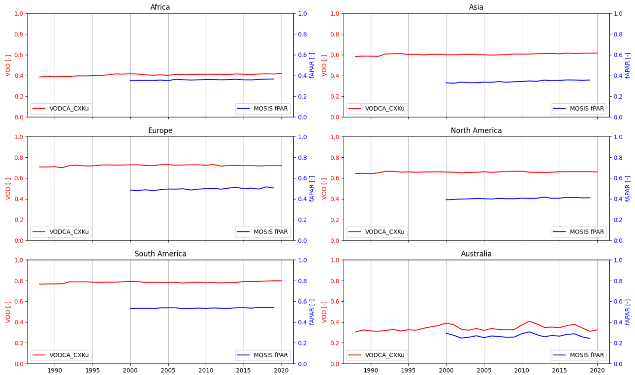
Figure A11. Yearly time-series per continent for VODCA CXKu and MODIS fPAR.
