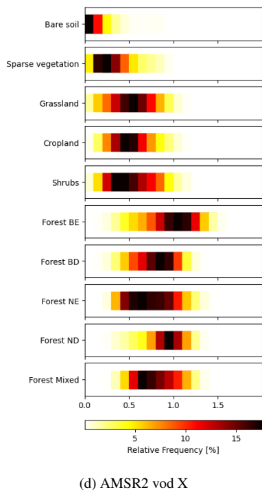
Figure A16. Values ranges per LC class for VODCA L (a), SMAP vod L (b), VODCA CXKu (c) and AMSR2 vod X (d). Bins are colored by the relative frequency in percent of the respective values. ESA CCI LC was used.
