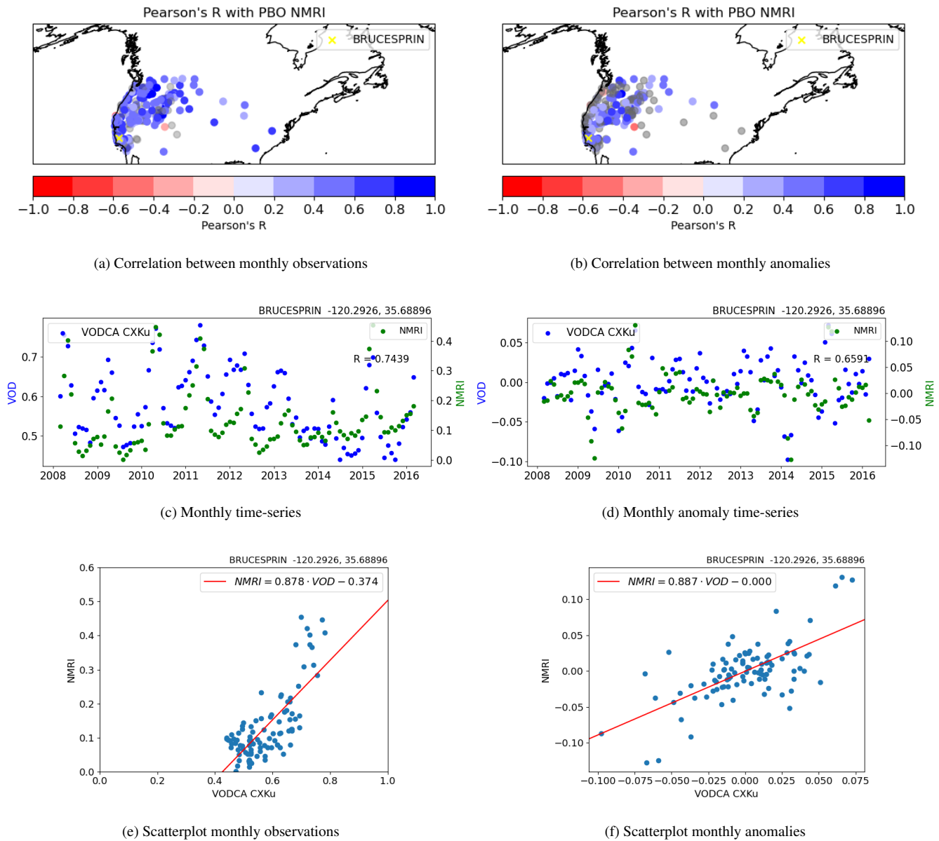
Figure 14. Pearson's R between monthly VODCA CXKu and NMRI for the PBO stations over the bulk signal (a) and anomalies (b). The stations with non-significant correlations are shown in grey. time series over the bulk signal (c) and anomalies (d) of VODCA CXKu (blue) and PBO NMRI (green), as well as scatterplot over the bulk signal (e) and over anomalies (f) for a station with good agreement between datasets (BRUCESPRIN, lon -120.29, lat 35.68, indicated with a cross in the correlation maps).
