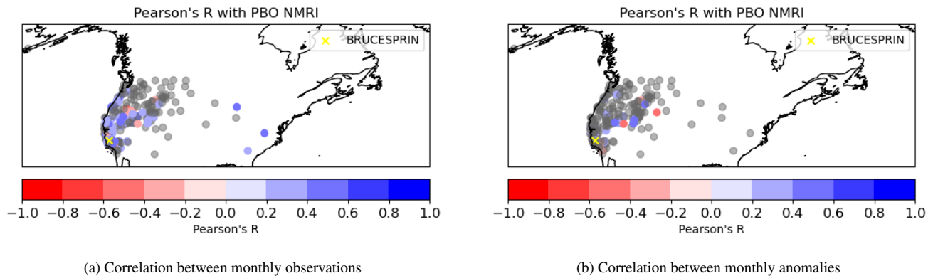
Figure 15. Pearson's R between monthly VODCA L and NMRI for the PBO stations over the bulk signal (a) and anomalies (b). The stations with non-significant correlation are shown in grey.
