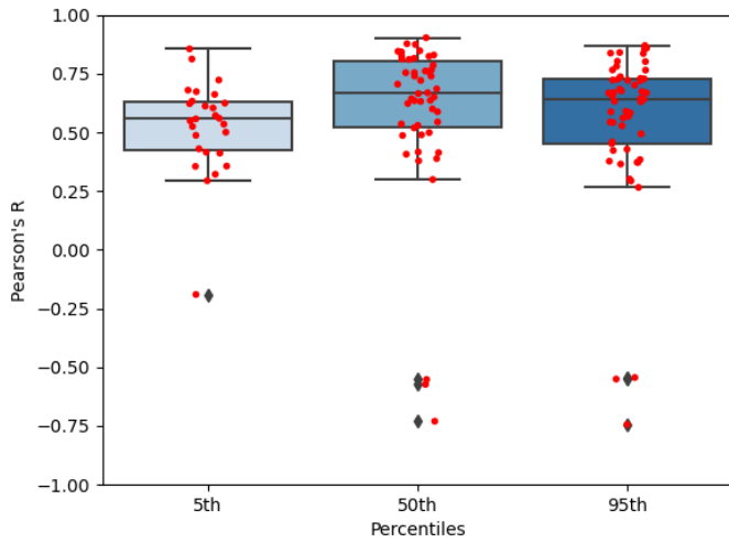
Figure A25. Agreement between VODCA CXKu (SD) and sapflow (SD) for the monthly 5th, 50th and 95th percentiles. Red points represent the correlation for each station.
