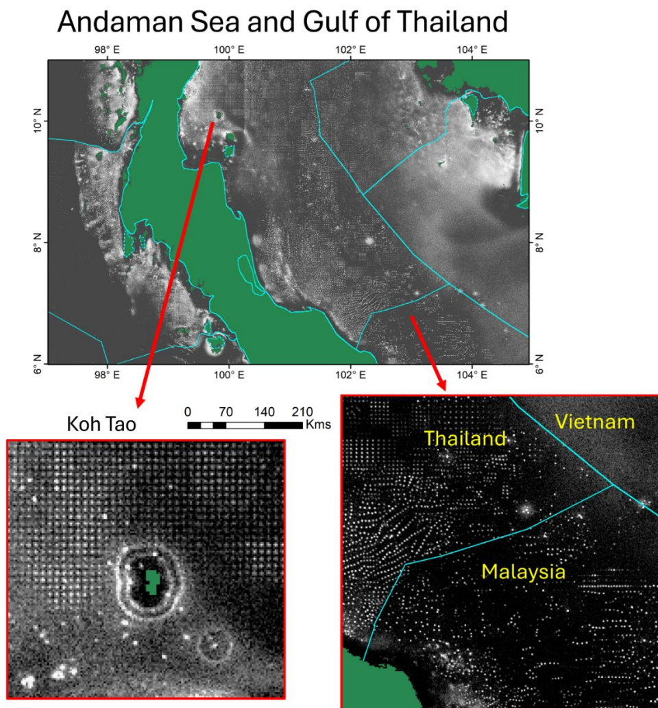
315 Figure 7. VBD percent detection frequency for portions of the Andaman Sea and Gulf of Thailand. Insets show the grid pattern common across much of Thailand’s offshore fisheries. The center grid cells have 20 to 50 times more detections than the adjacent cells. In Thailand, many grids align to the cardinal directions, and the spacing between grid centers
