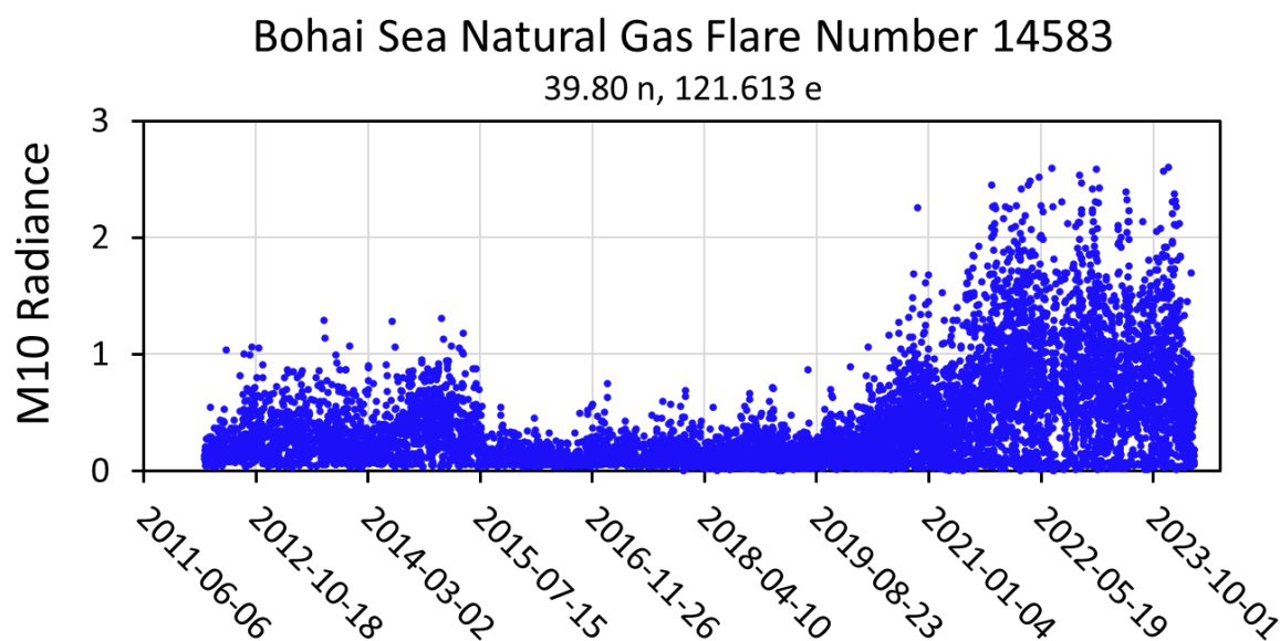
Figure 17. Nightly shortwave infrared (band M10) radiance for the Bohai Sea natural gas flare from the VIIRS Nightfire product line. Because the DNB radiances closely track the M10 radiance levels, we conclude that the DNB radiance is dominated by the flare's radiant emissions and not the electric lighting at the site.
