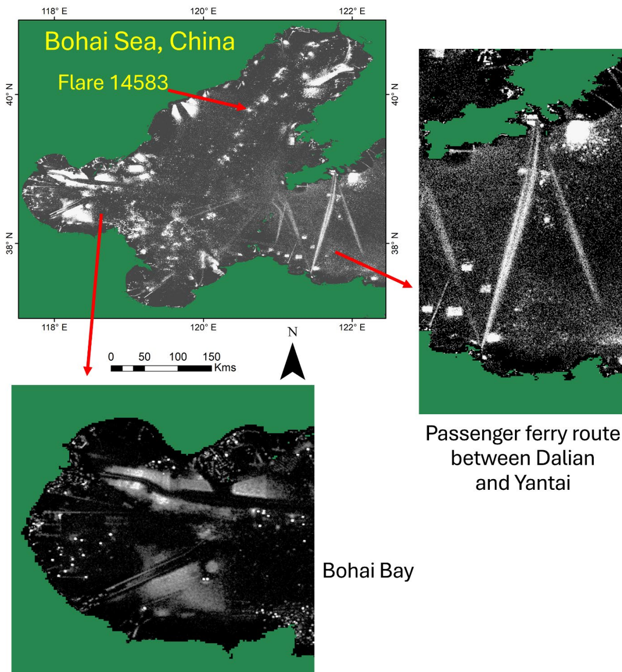
370 Figure 11. Multiyear VBD percent frequency of detection in the Bohai Sea of China. The area has multiple anchorages, platforms, and transit corridors.
