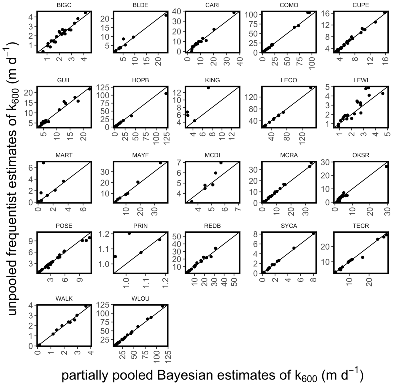
390 Figure 7. Comparison of partially pooled Bayesian and unpoled frequentist estimates of k_{600} . Black 1:1 lines overlay the points for reference.
