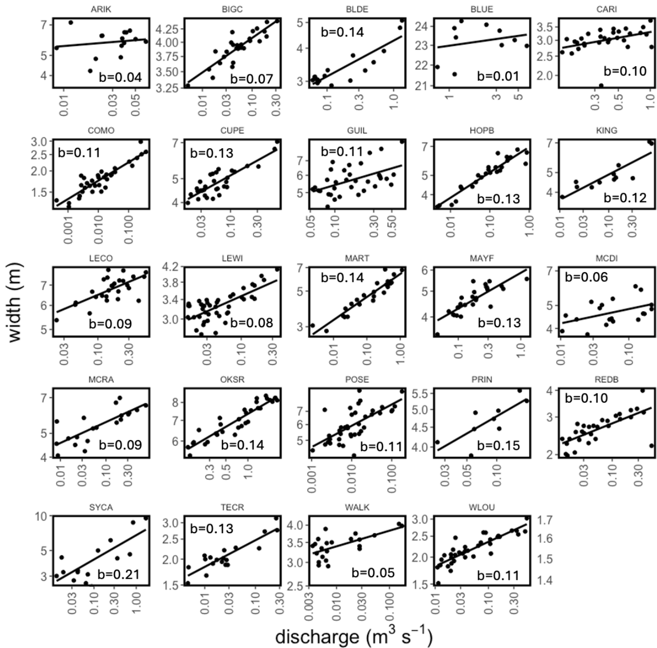
Figure 4. At-a-station hydraulic geometries for relationship between Q and w . The exponent b of the power law relationship \bar{w} = \alpha Q^b is the linear slope of the relationship in log-log space and is denoted on each subplot.
