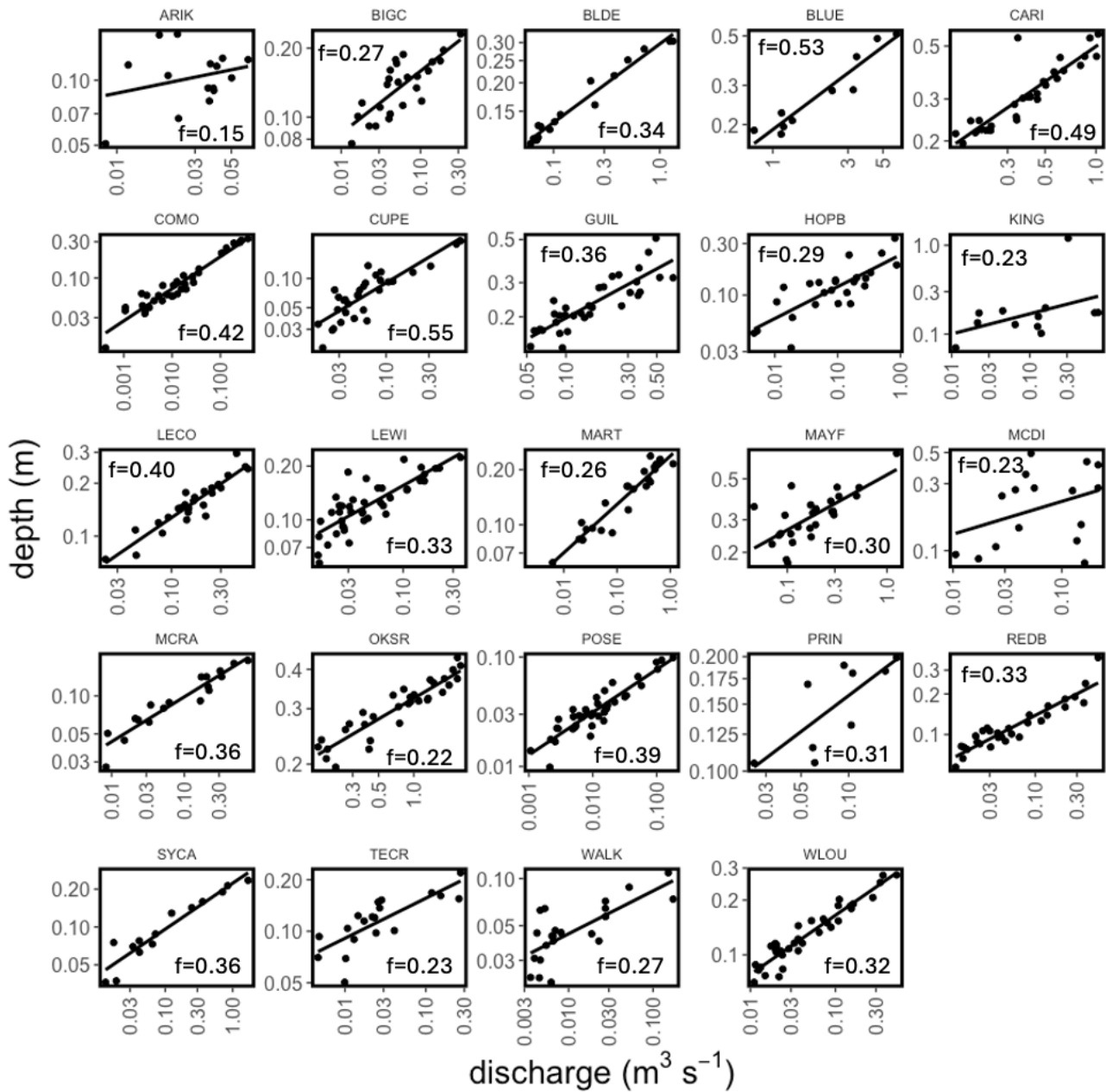
335 Figure 5. At-a-station hydraulic geometries for relationship between Q and \bar{z} . The exponent f of the power law relationship \bar{z} = cQ^f is the linear slope of the relationship in log-log space and is denoted on each subplot.
