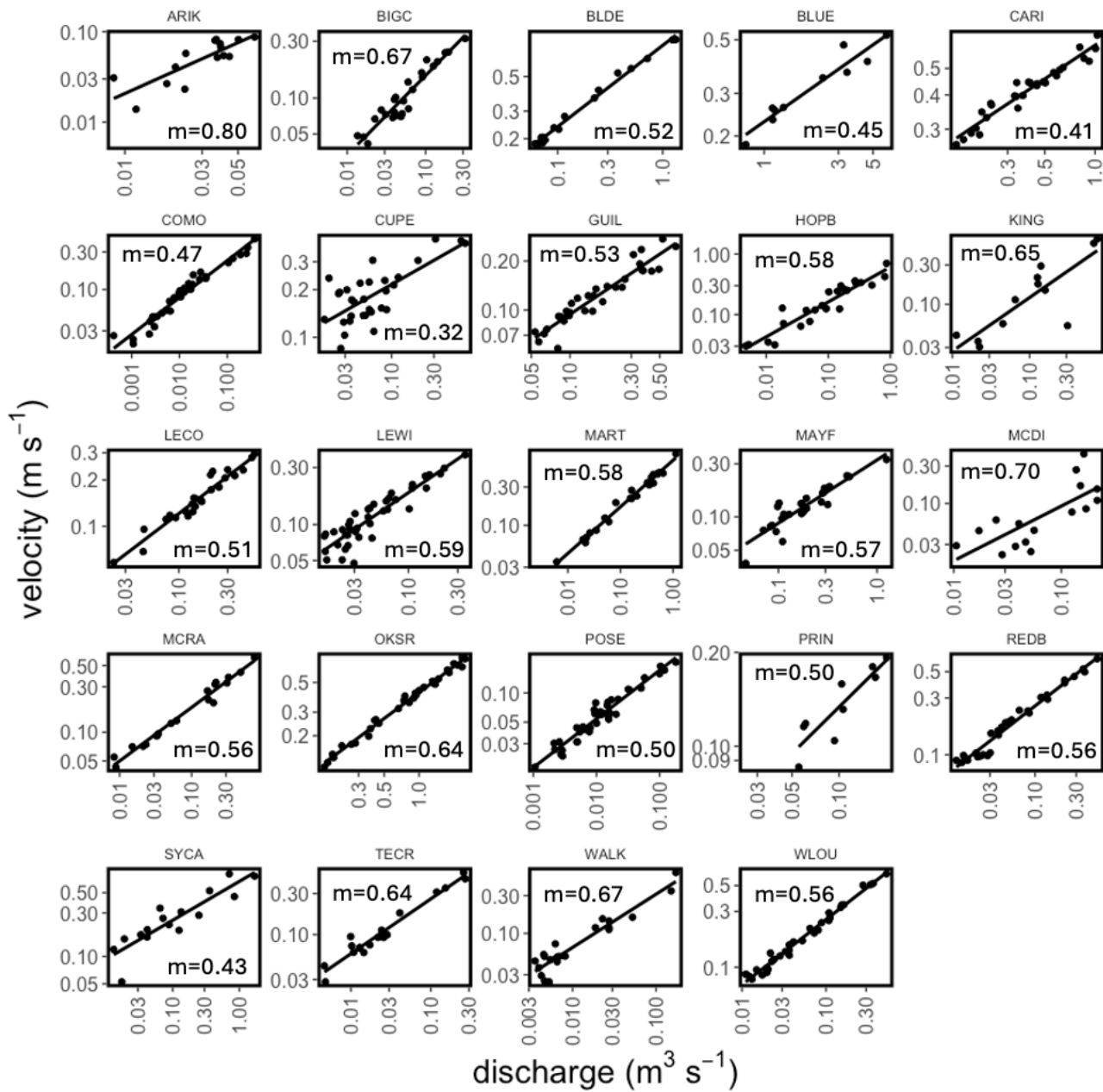
340 Figure 6. At-a-station hydraulic geometries for relationship between Q and v . The exponent of the power law relationship v = kQ^m is the linear slope of the relationship in log-log space and is denoted on each subplot.
