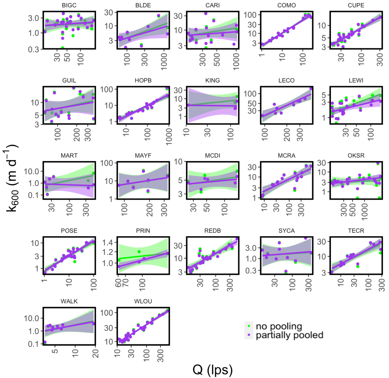
395 Figure 8. Relationship between Q and partially pooled Bayesian and unpooled frequentist estimates of k_{600} . The unpooled estimates are shown in green, with a green regression line with 95% confidence intervals, while the partially pooled estimates are shown in purple with a purple regression line with 95% confidence intervals.
