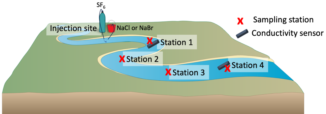
120 Figure 2. Diagram of a model study reach for NEON tracer-gas experiments. Each ~500-m study reach comprises an injection site and four downstream sampling stations (Stations 1 – 4). At the upstream injection site, SF 6 is diffused into the water column with an air stone and NaCl or NaBr is dripped into the stream. After plateau concentrations are reached at the downstream end of the study reach, injection rates are maintained and field quintuplicate samples for SF 6 and NaCl or NaBr concentrations are collected at four downstream stations spaced along the study reach. At the upper and lower stations, conductivity sensors are deployed and 125 used to monitor either 1) when NaCl plateau concentrations are reached (for NaCl continuous injections) or 2) when a NaCl “slug”
