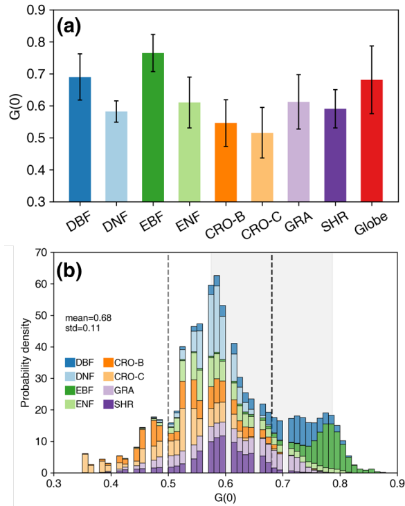
315 Figure 11. Statistics (a) and probability density distributions (b) of the global nadir leaf projection function ( G(0) ) for different plant 316 functional types. The error bars in (a) represent the standard deviation. The black dash line and shade area in (b) indicate the global G(0) 317 mean and standard deviation. The gray dashed line represents the G(0) ( =0.50 ) of spherical leaf angle distribution. The mean, standard 318 deviation, and probability density values are weighted by leaf area index. See Fig. 1 for the acronyms.
