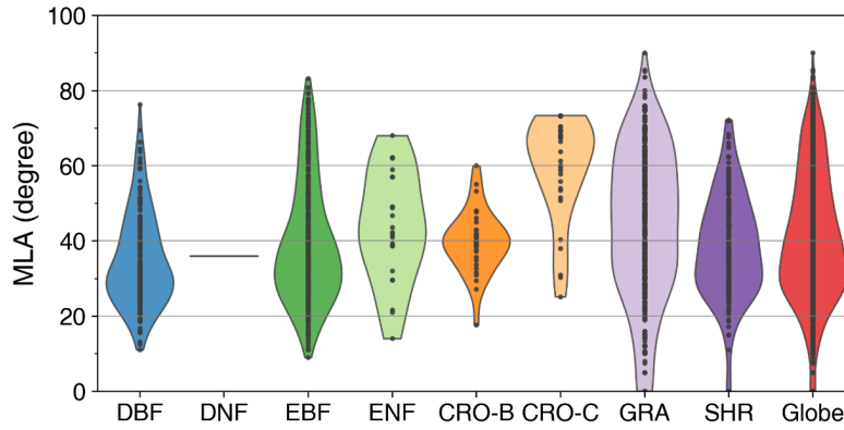
Figure 5. Distribution of global mean LIA (MLA) for different plant function types (see Fig. 1 for acronyms). The last shape shows the global average. Statistics are conducted for each species as represented by points in the figure.
