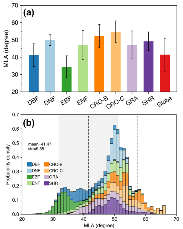
Figure 9. Statistics (a) and probability density distributions (b) of the global mean leaf inclination angle (MLA) for different plant functional types. The error bars in (a) represent the standard deviation. The black dash line and shade area in (b) indicate the global MLA mean and standard deviation. The gray dashed line represents the MLA (=57.30°) of spherical leaf angle distribution. The mean, standard deviation, and probability density values are weighted by leaf area index. See Fig. 1 for the acronyms.
