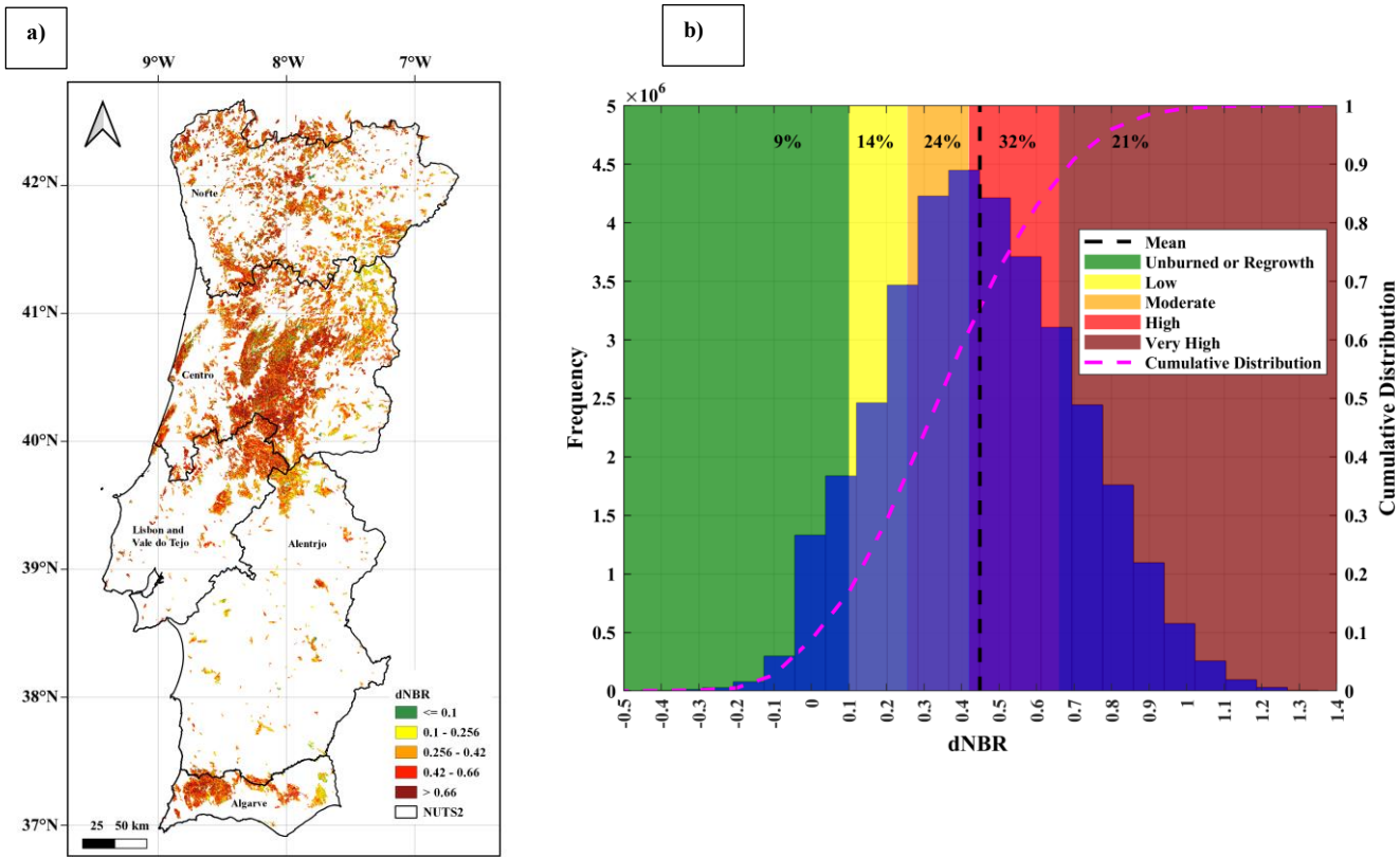
Figure 2. (a) Spatial distribution of the overlaid dNBR pixel value of all the years (1984 to 2022) is presented, with the average pixel value presented in the area where burned more than once. “Nomenclature of Territorial Units for Statistics” (presented as NUTS2) frontiers (Registo Nacional de Dados Geográficos - Direção-Geral do Território (DGT), 2024; Meneses et al., 2018) was applied to demonstrate the extent of the mainland Portugal and its five regions. (b) The histogram shows the distribution and frequency of all annual dNBR pixel counts, with no averaging. On the secondary y-axis, the cumulative distribution of the dNBR pixel value is presented. The dNBR classification according to EFFIS (European Commission, 2018; Llorens et al., 2021) combined with percentage of pixel counts within these classes are also shown (panel (b)).
