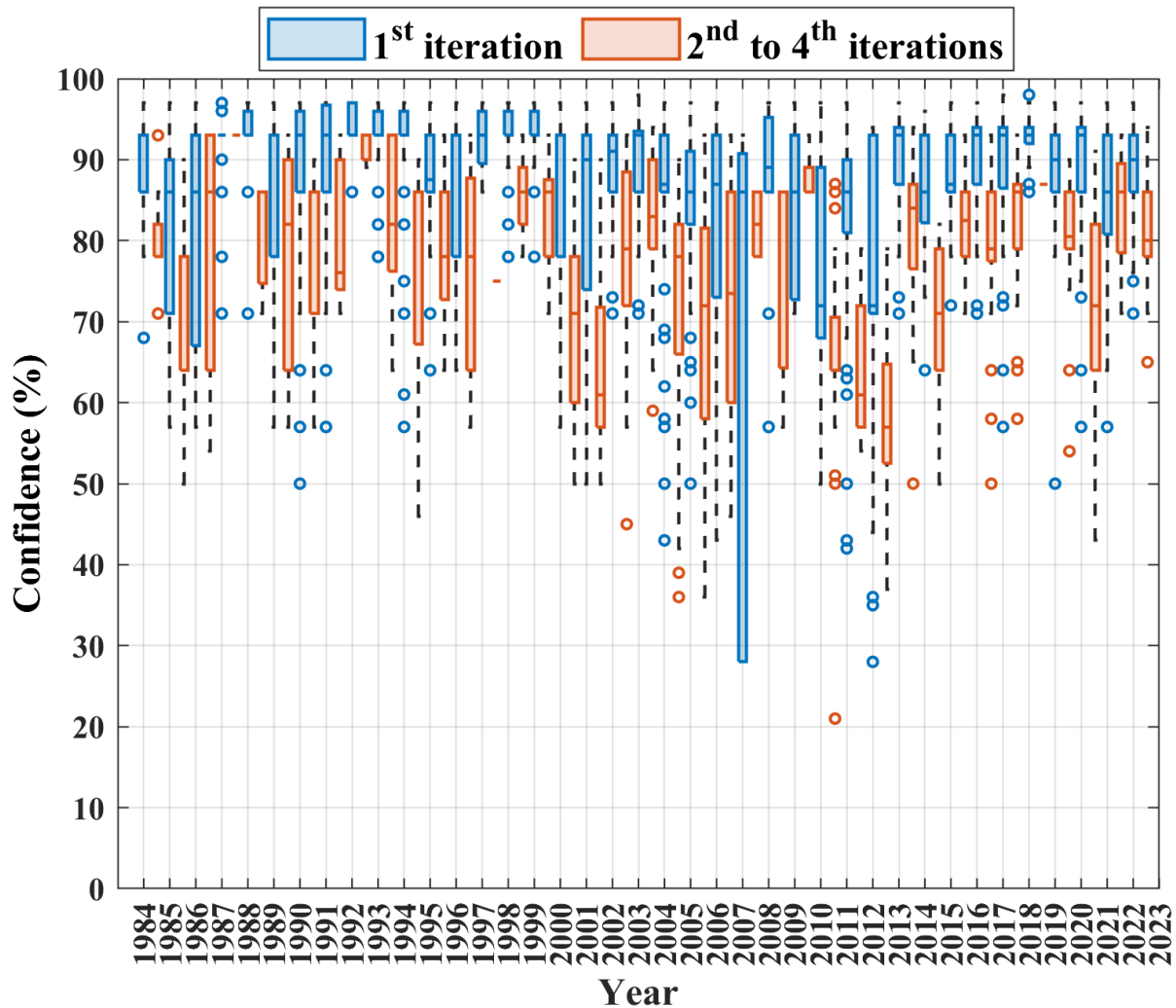
Figure 5. Fire-by-fire confidence variability over the years obtained through the first iteration or second to fourth iterations. The median (50 th percentile) is shown as the central line within the boxes. The first quartile (25 th percentile or Q1) forms the bottom of the box, while the third quartile (75 th percentile or Q3) forms the top. The interquartile range (IQR), calculated as difference between the third and first quartiles ( Q3 - Q1 ), is represented as the height of the boxes. The upper whisker extends to the largest data point ( \leq Q3 + IQR \cdot 1.5 ), while the lower whisker extends to the smallest data point ( \geq Q1 - IQR \cdot 1.5 ). The outliers are shown as circular points.
