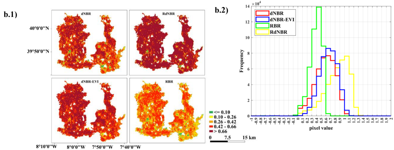
Figure 6. Burn severity estimates via dNBR, dNBR-EVI, RBR, and RdNBR for two large fires (area \geq 10 k ha) as examples are presented in panels (a.1 and b.1). The thresholds applied are according EFFIS classification for dNBR (European Commission, 2018; Llorens et al., 2021). However, to facilitate the comparison of different severity indices, the same color classification was applied on all the indices. In the second panel, the histograms represent the distribution of different burn severity estimates via different indices.
