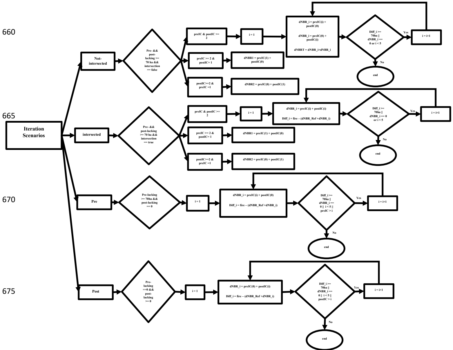
Figure A3. Flowchart represents the iteration scenarios. PreIC and PostIC stand for the pre- and post-fire image collections in GEE and their size or the number of images within each IC is shown (e.g., PreIC ≤ 3 meaning the number of images within this IC is less or equal to 3). All the ICs are sorted from images with the highest SUITABILITY to the lowest and the first image, shown as e.g., PostIC(0), is the first image within the sorted post-fire IC with the highest SUITABILITY.
