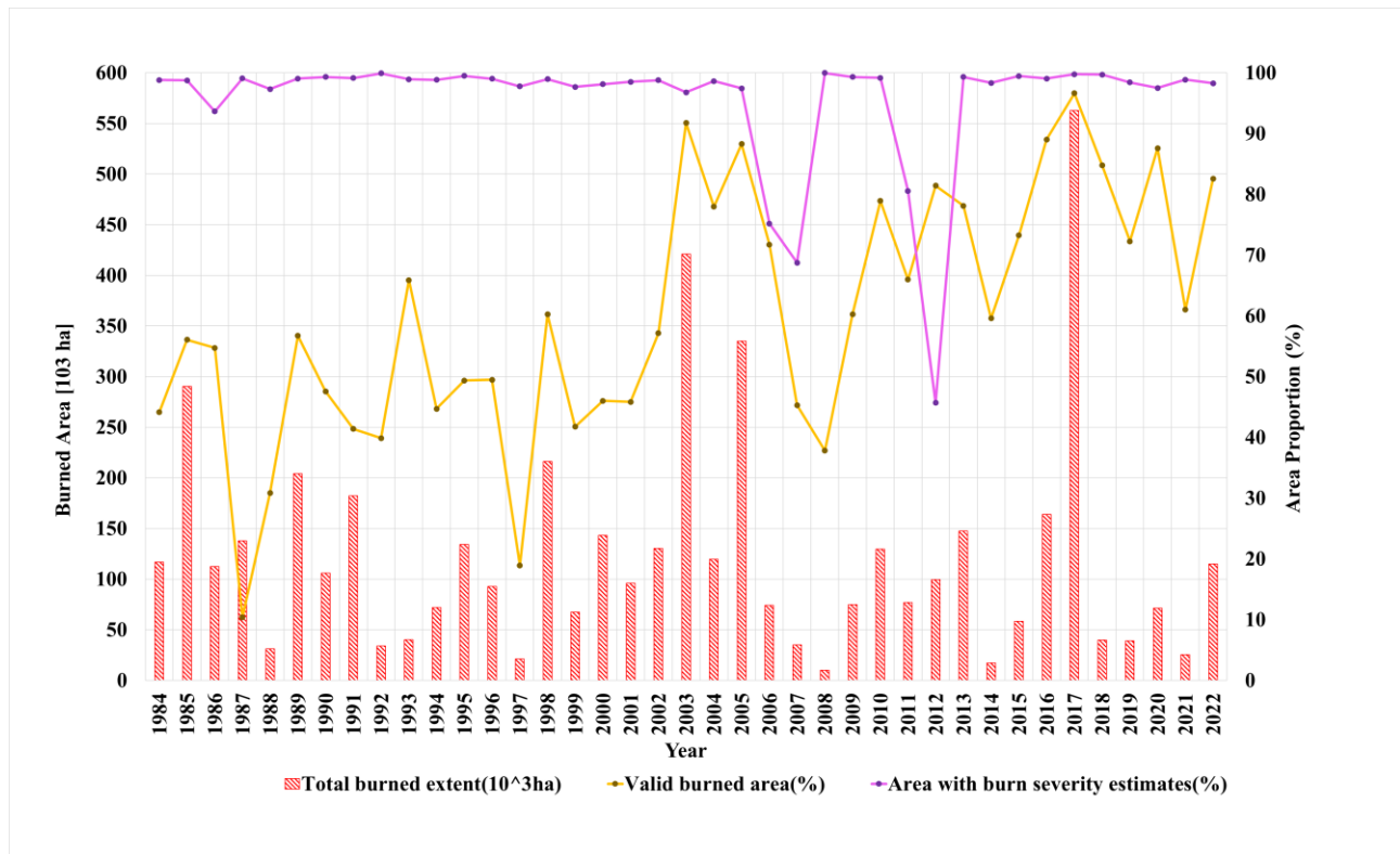
345 Figure 3. Timeline of total burned extents of fires 1984 to 2022. On left-y axis, annual burned area in unit of 10^3 ha and on secondary y-axis the percentages of valid burned area and area with burn severity estimates are shown.
