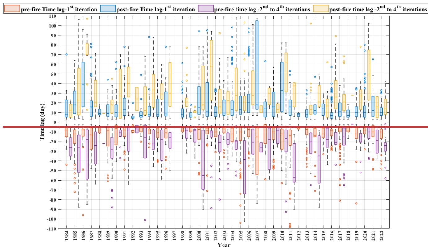
Figure B1. The annual variability of pre- and post-fire time lags in units units of days are presented, both from the first and second to fourth iterations. Negative values represent pre- fire time lags and positive ones show post-fire time lags. No data is presented for 1997 (no valid fire data).
