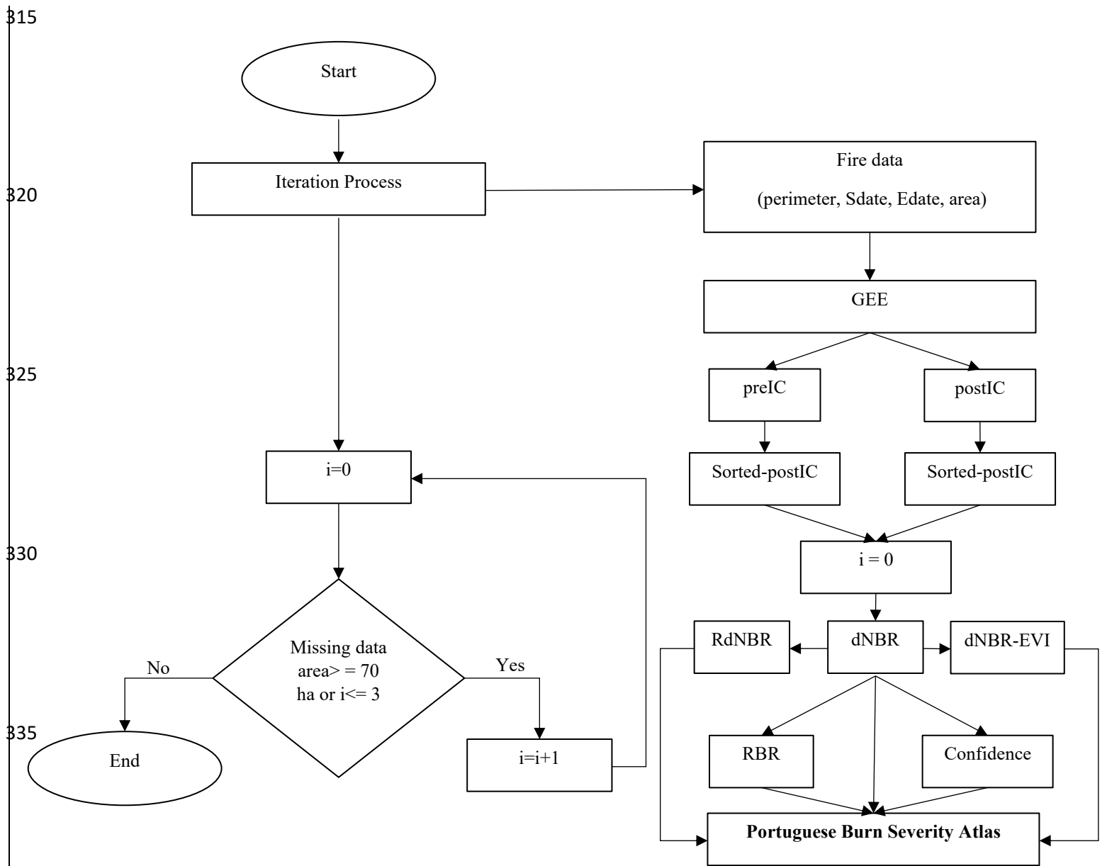
Figure 1. Flowchart demonstrat demonstrates ing the iteration process used for the calculation of burn severity indices and to have estimates for the largest proportion of the fire area as possible. PreIC and postIC are our abbreviated versions of pre-fire ImageCollection and post-fire ImageCollection, respectively. Sorted-pre and -postICs were sorted based on SUITABILITY of images from highest to lowest.
