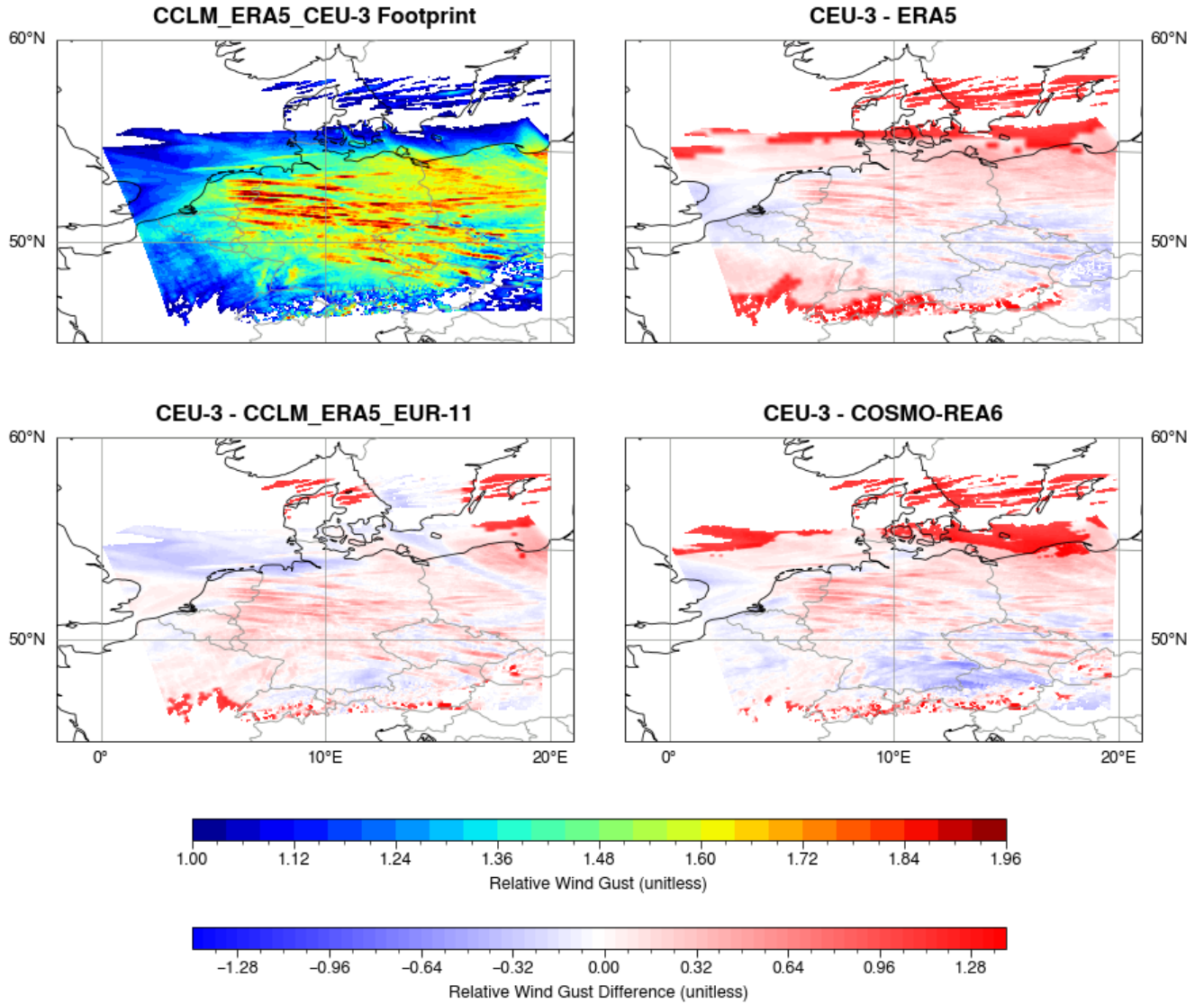
Figure 10. Storm footprint for windstorm KYRILL (Jan 2007) derived from the CCLM_ERA5_CEU-3 data set and shown in Fig. 2, displayed in the top left panel. The three remaining panels display the difference between the CCLM_ERA5_CEU-3 footprint and the footprints derived from ERA5, COSMO-REA6, and CCLM_ERA5_EUR-11 after regridding to the CCLM_ERA5_CEU-3 resolution, in clockwise order. All panels are plotted at the CCLM_ERA5_CEU-3 horizontal resolution. KYRILL is the strongest storm in our database.
