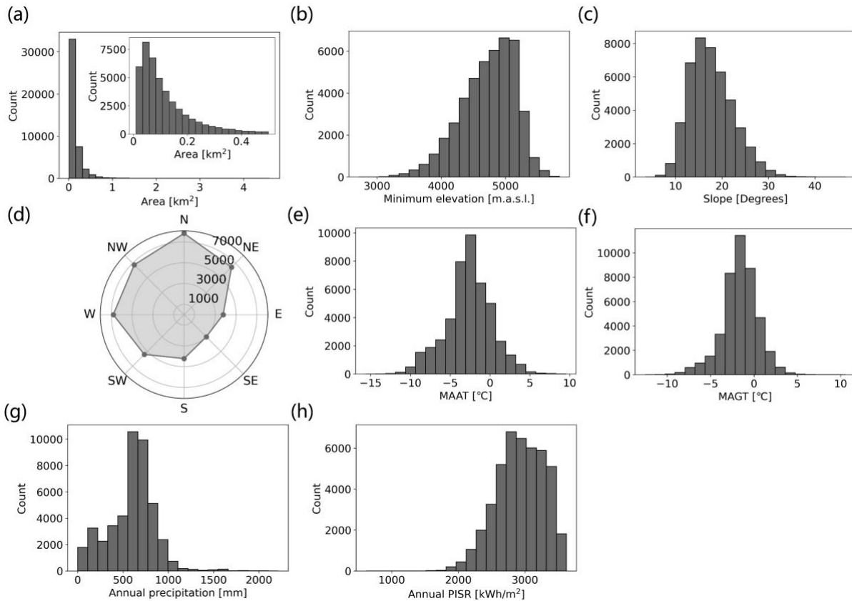
375 Figure 6. Statistical summaries of the geomorphic and current climatic features of rock glaciers in the study region. (a) The areal histogram of all the rock glaciers on the Tibetan Plateau. The inset shows the areas smaller than 0.5 \text{ km}^2 . (b)-(h) are histograms of the minimum elevations, slopes, aspects of the rock glaciers with the radial axis representing the counts, Mean Annual Air Temperature (MAAT), Mean Annual Ground Temperature (MAGT), annual precipitation, and annual Potential Incoming Solar Radiation (PISR), respectively.
