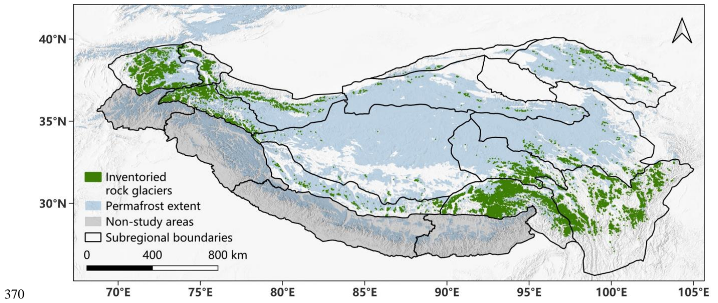
Figure 5. Rock glacier inventory on the Tibetan Plateau (TPRoGI). The permafrost in Hengduan Shan is overlapped by the rock glaciers thus not visible on the map. The permafrost extent map is from Obu et al. (2018).
