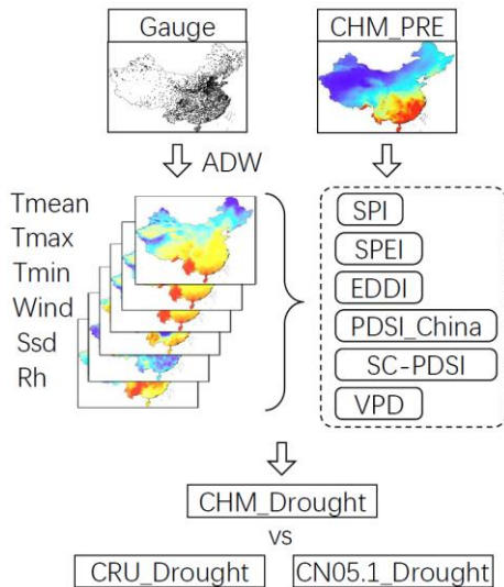
165 Figure 2: Flowchart of the drought index construction system. The meteorological variables include maximum temperature (Tmax), minimum temperature (Tmin), average temperature (Tmean), average wind speed (Wind), sunshine duration (Ssd), and average relative
