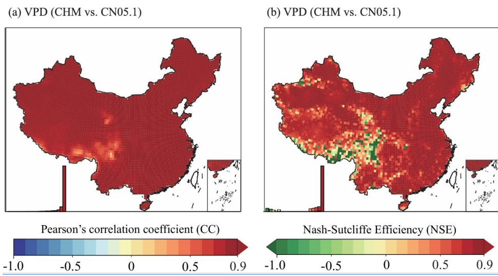
430 Figure 8: Spatial distributions of correlation (a) and NSE (b) of VPD based on CHM and CN05.1 data
