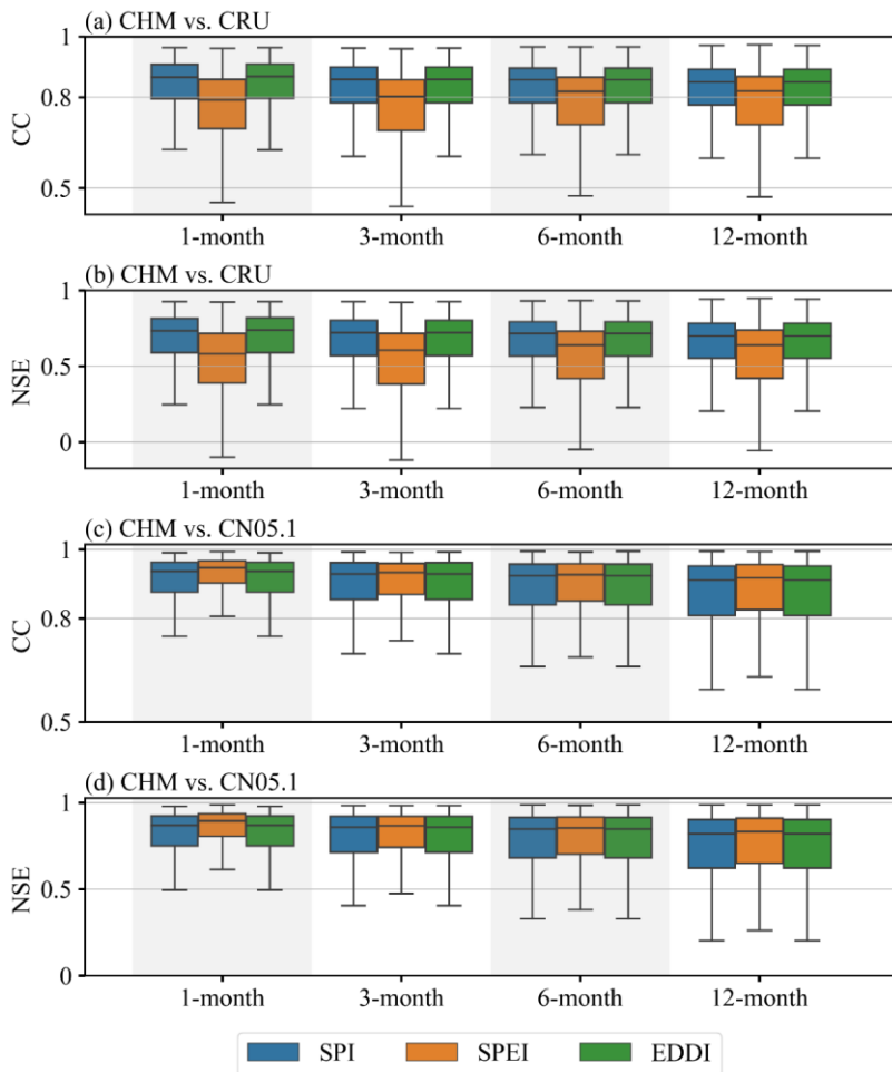
385 | Figure 6: Box plots of the CC and NSE of three drought indices (SPI, SPEI, EDDI) calculated based on CHM and either (a, b) CRU or (c, d) CN05.1 at different month scales (1-, 3-, 6-, and 12-month). The middle line within each box indicates the median, the upper and the lower edges mark the 25th and 75th percentiles, and the whiskers show the 2.5th and 97.5th percentiles.
