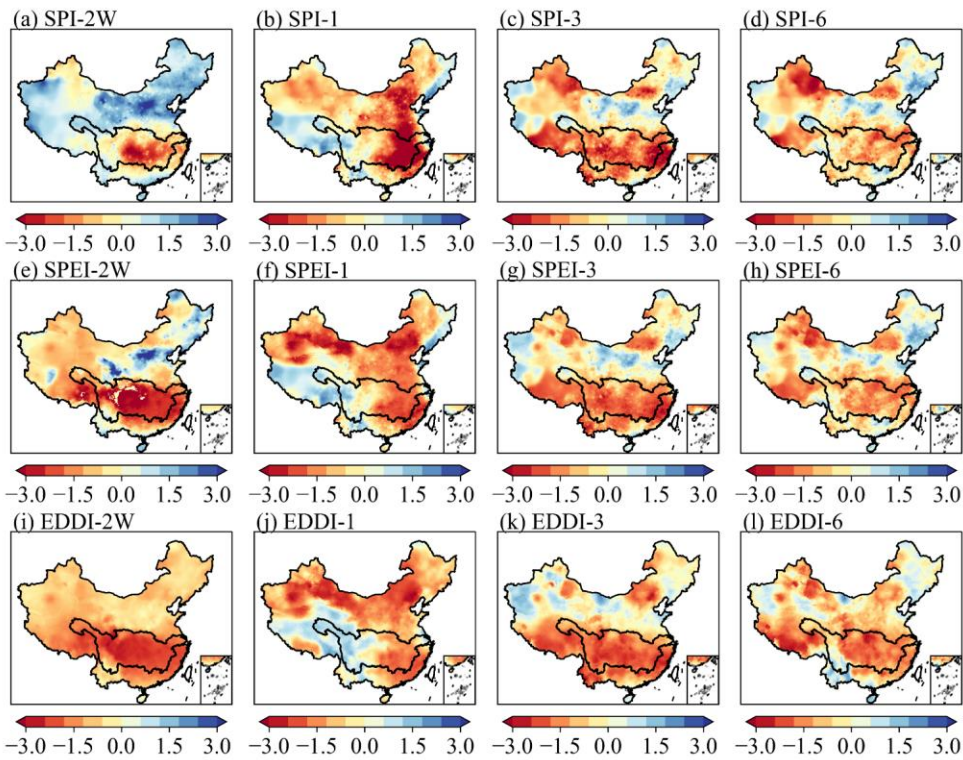
335 Figure 4: Spatial distribution of three drought indices (SPI, SPEI, and EDDI) in the Yangtze River Basin, China, across multiple timescales (2-week, 1-month, 3-month, and 6-month), using August 2022 as an example. (a–d) SPI-2W indicates the 2-week scale SPI, SPI-1 indicates the 1-month scale SPI, SPI-3 indicates the 3-month scale SPI, and SPI-6 indicates the 6-month scale SPI. The scales of SPEI and EDDI follow the same naming pattern.
