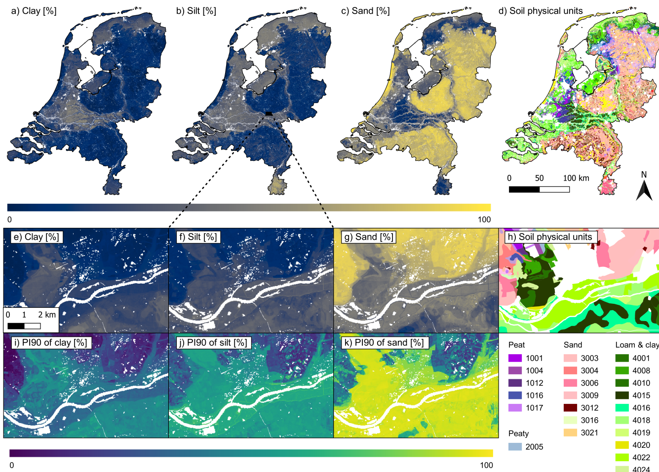
Figure 4. Mean predicted clay [%] (a & e), silt [%] (b & f) and sand [%] content (c & g) at 60 - 100 cm depth and associated prediction uncertainty (PI90 = 90 th prediction interval) and the soil physical units map of the Netherlands (BOFEK, Heinen et al., 2022, d & h) in comparison. The soil physical unit codes can be found in Heinen et al. (2022); here grouped into the main categories (1xxx = peat, 2xxx = peaty, 3xxx = sand, 4xxx = loam/clay and 5xxx = loess). The zoom-in area around Wageningen was chosen since this area contains all main soil physical categories except loess.
