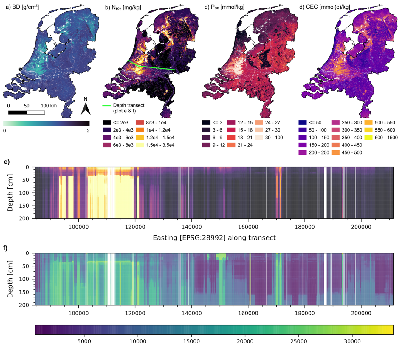
Figure 5. Median predicted BD [ g/cm^3 ] (a), N_{tot} [mg/kg] (b), P_{ox} [mmol/kg] (c), and CEC [mmol(c)/kg] (d) at 0 - 5 cm depth; and median predicted N_{tot} (e) and PI90 (90 th prediction interval) as a measure of the associated prediction uncertainty (f) along the depth transect shown in b.
