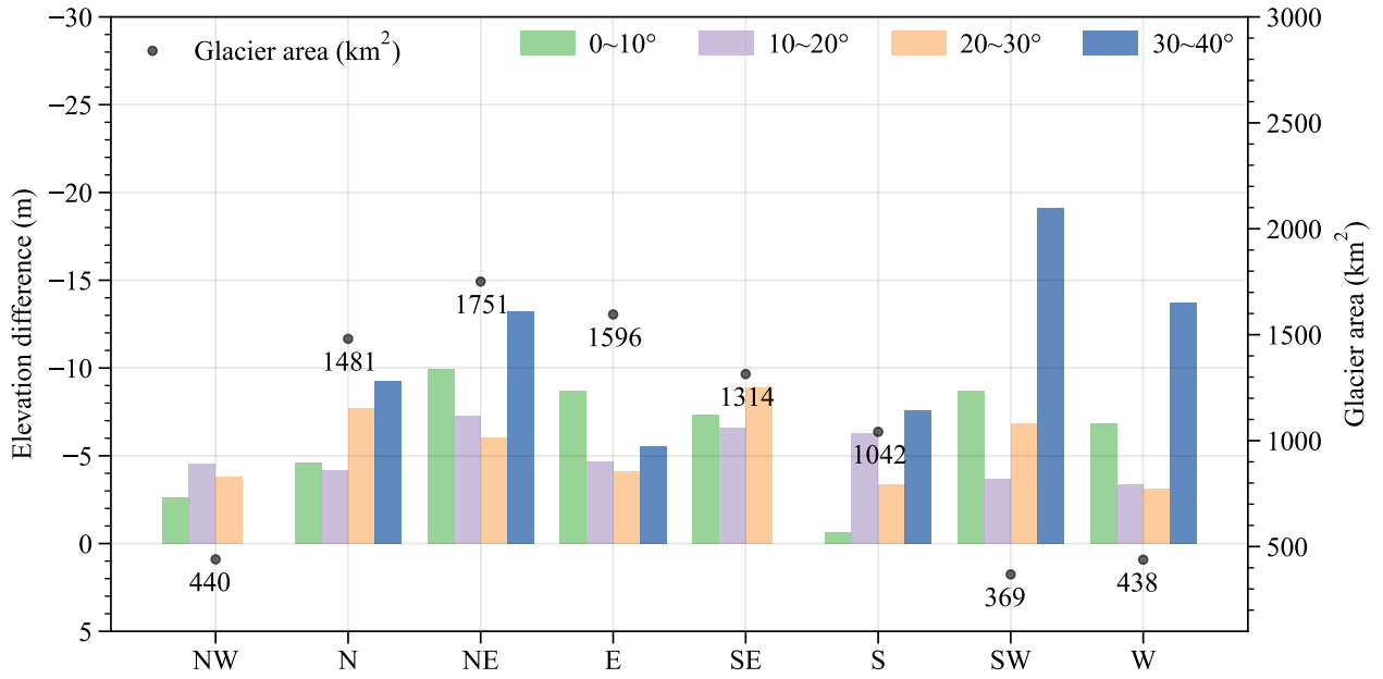
Figure 4. Elevation difference of large glaciers ( > 10 \text{ km}^2 ) by aspect and slope.
