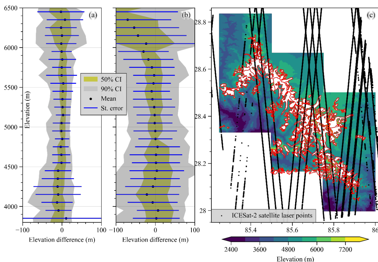
Figure A1. Comparison of Topo DEM (a) and ATL06 (b) elevation differences along altitude (Off-glacier region, Xixiabangma Mountains). Tracks of ATL06 are presented in (c). Elevation zones with fewer than 200 laser spots of ATL06 were excluded from the statistical analysis.
