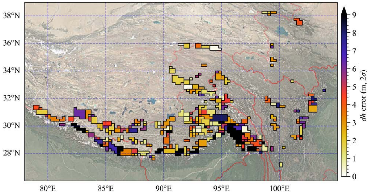
Figure 3. Spatial distribution of glacier surface elevation change error ( 2\sigma ) from 1970s to 2000. The polygons represent group. The base map depicted in the image utilizes Google Terrain Map, accessed through QGIS for visualization.
