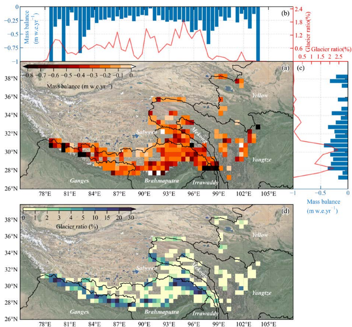
Figure 5 0.5° gridded product over the ETPR. (a) Characteristics of glacier mass balance. (d) Glacier ratio. Statistics of mass balance along longitude and latitude are presented in (b) and (c), respectively. The glacier ratio accounts for the glacier area divided by grid area. The base map depicted in the image utilizes Google Terrain Map, accessed through QGIS for visualization.
