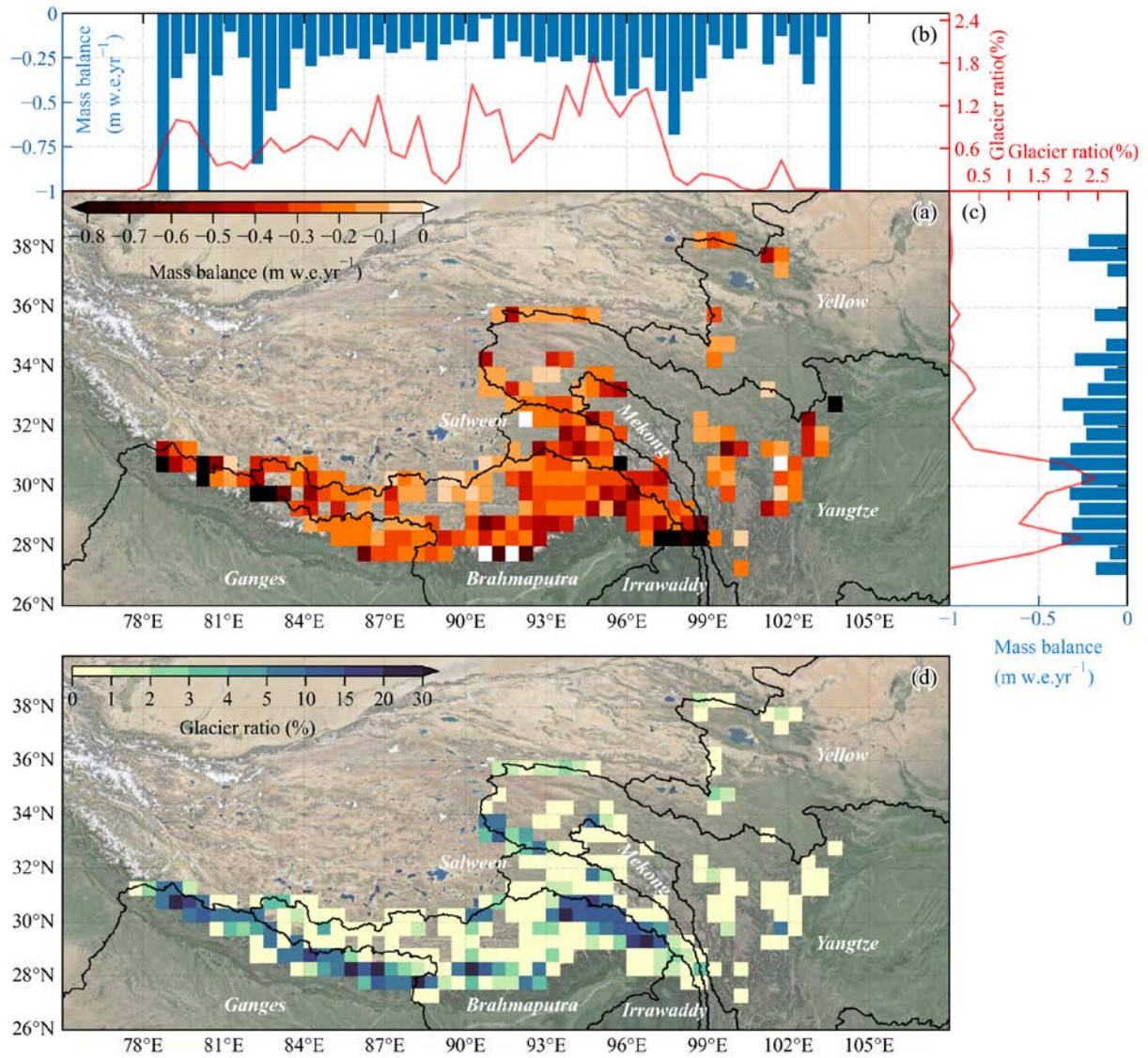
Figure 5 0.5° gridded product over the ETPR. (a) Characteristics of glacier mass balance. (d) Glacier ratio. Statistics of mass balance along longitude and latitude are presented in (b) and (c), respectively. The glacier ratio accounts for the glacier area divided by grid area. The base map depicted in the image utilizes Google Terrain Map, accessed through QGIS for visualization.
