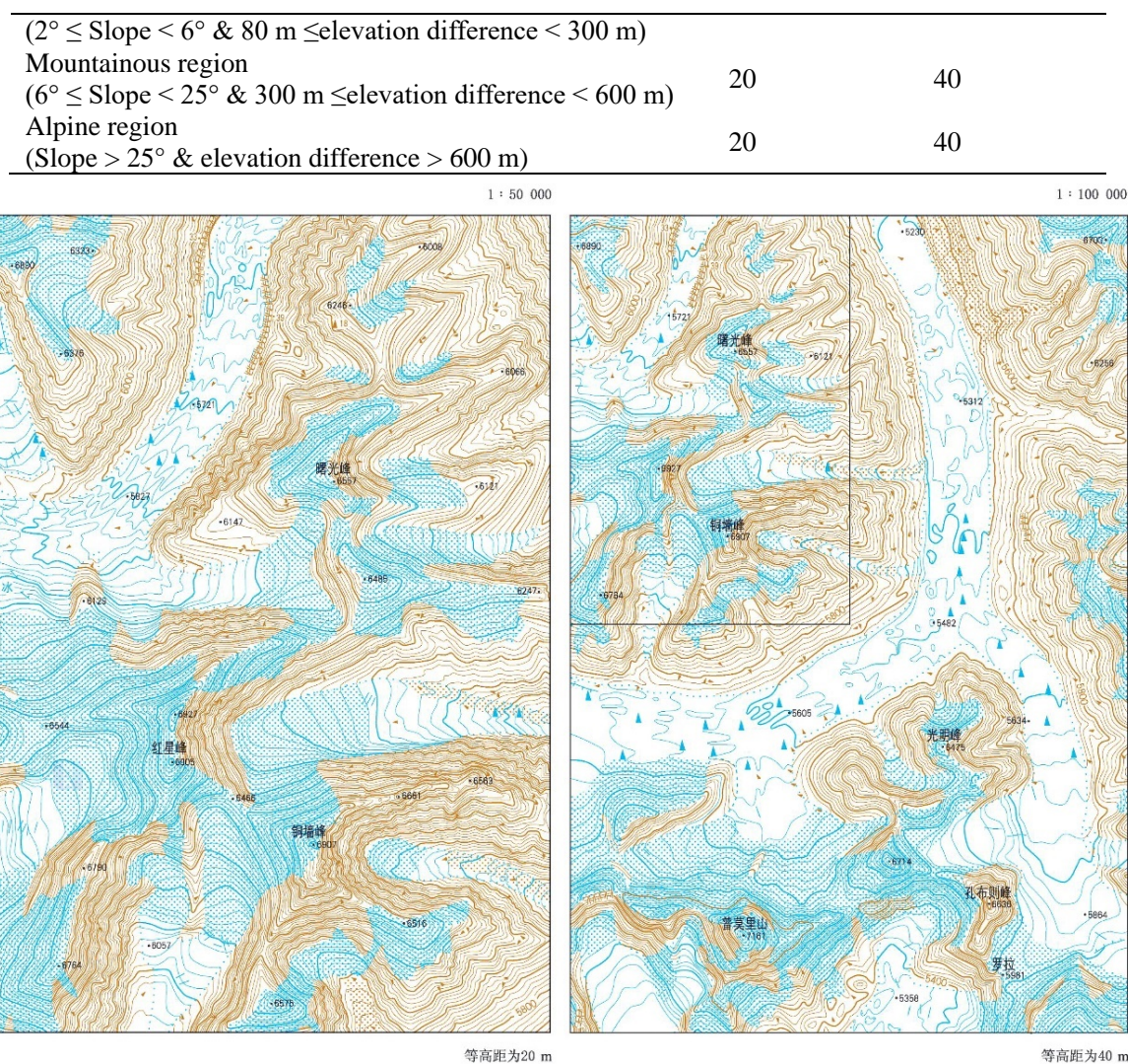
Figure A2. A sample of topographical maps in glacierized region (originate from the NPSC, GB/T 12343.1-2008).
