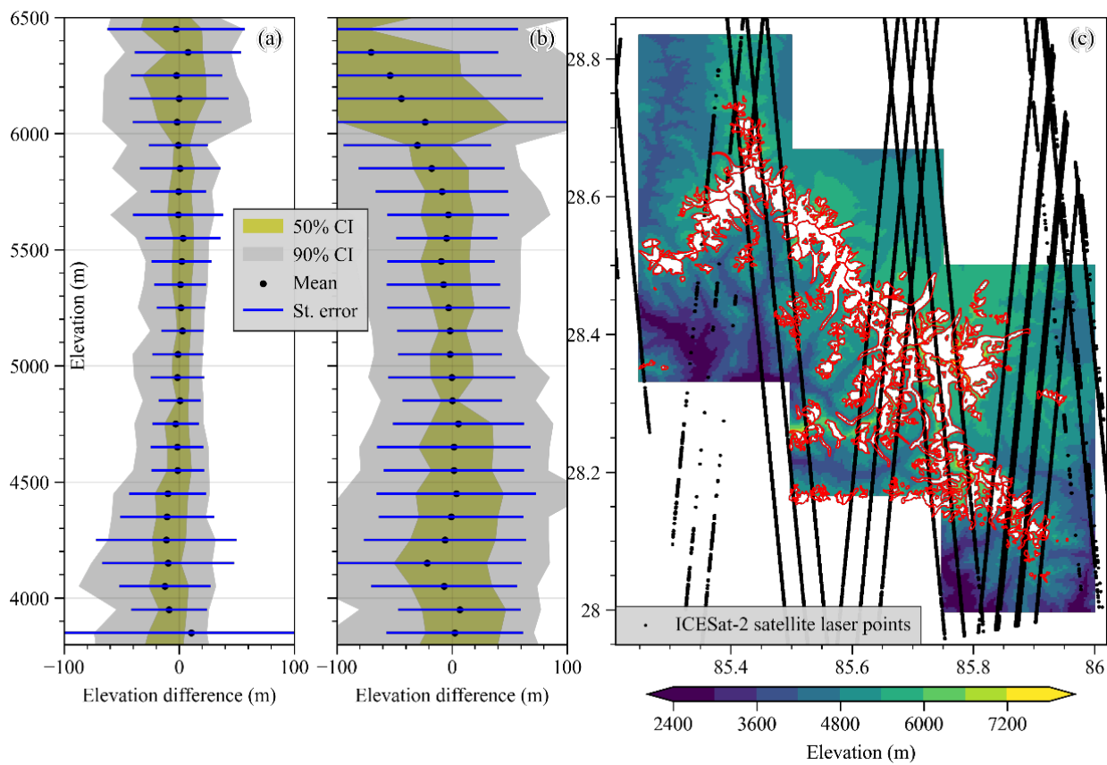
Figure A1. Comparison of Topo DEM (a) and ATL06 (b) elevation differences along altitude (Off-glacier region, Xixiabangma Mountains). Tracks of ATL06 are presented in (c). Elevation zones with less-fewer than 200 laser spots of ATL06 were excluded from the statistical analysis.
