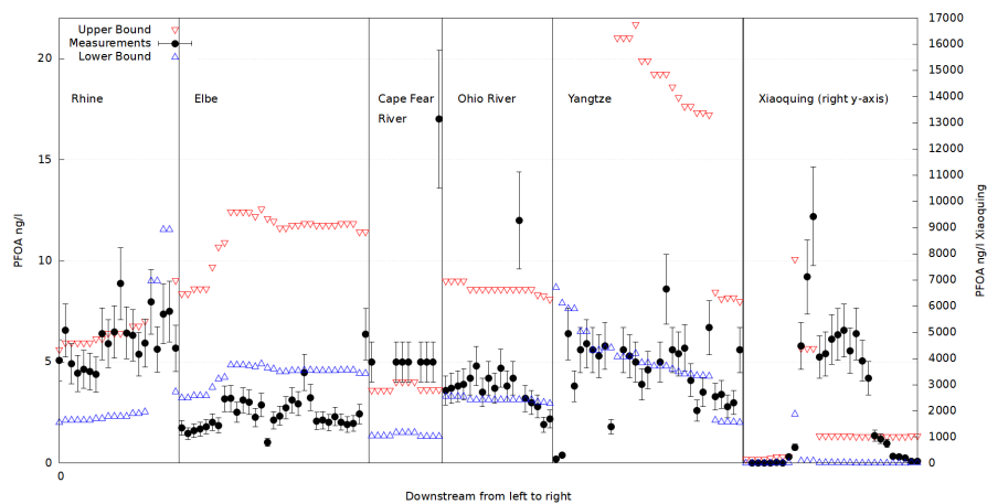
Figure 7. Overview of several river concentration measurements by Sun et al.(Sun et al., 2016), Pétré et al. (Pétré et al., 2022), Heydebreck et al. (Heydebreck et al., 2015) and Jin et al. (Jin et al., 2009) in comparison with the upper and lower bound estimation by POPE. The rightmost values are closest to the sea.
