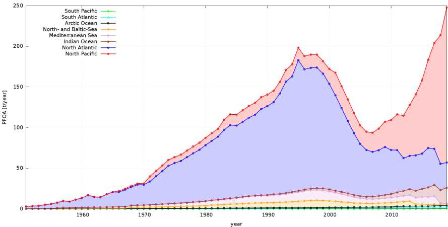
Figure 10. Total PFOA emissions to oceans in the upper bound scenario
