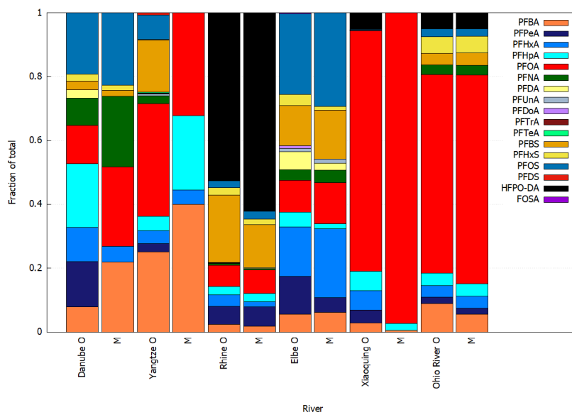
Figure 9. Relative fraction of all PFAS considered by POPE and the respective studies for a selection of rivers in the sections with measurements available . O indicates an observation, M designates the corresponding modelled -modeled result. The order of substances in the legends corresponds to the inverse vertical order of fractions.
