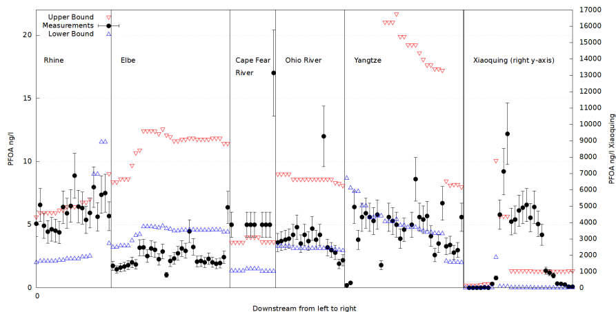
Figure 7. Overview of several river concentration measurements by Sun et al.(Sun et al., 2016), Pétré et al. (Pétré et al., 2022), Heydebreck et al. (Heydebreck et al., 2015) and Jin et al. (Jin et al., 2009) in comparison with the upper and lower bound estimation by POPE. The rightmost values are closest to the sea.
