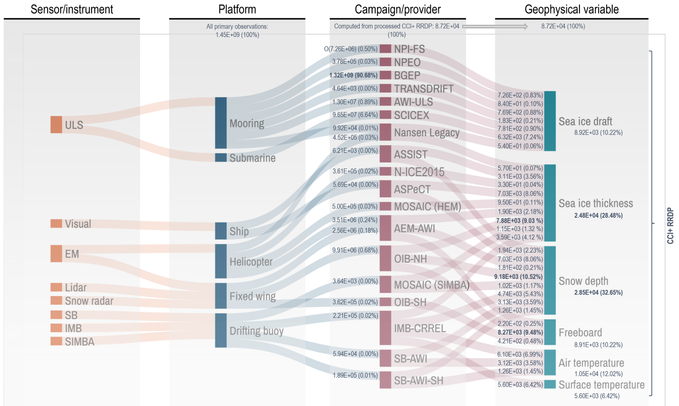
Figure 2. Sankey diagram providing an overview of the data sources used in the CCI SIT RRD and how they are acquired, by whom/when and what has been observed. The diagram is shown by four categories; sensor or measurement type, platform, campaigns (Table 2), derived geophysical variable, and their dependencies. We note that the data volume included in the CCI SIT RRD is represented here by numbers (in scientific notation) and percentages, and it is dependent on the processing level. Platform data volume denotes raw data, while campaign/geophysical variables refer to processed data. Note that the highest contributing data sources (at different processing levels) are highlighted in bold, defined as the the three highest contributing (in %) unless there is a large gap to the lesser contributors. In particular, the platform/mooring contributes more than 80% of the data, which primarily reflects the large time series, high sampling frequency, and temporal coverage of the buoys. In contrast, campaign (OIB-NH, ASPeCt, or SCICEX) primarily reflect spatial coverage, since these numbers refer to the processed CCI SIT RRD. In total, SIT and SD account for approximately 60% of the CCI SIT RRD. The notation O(number) denotes an approximation.
