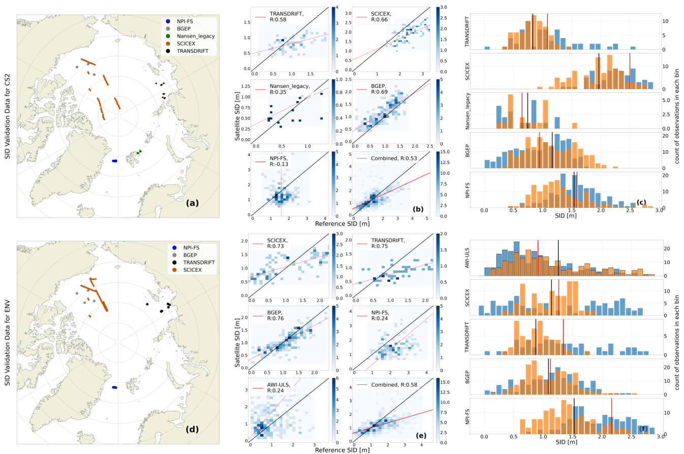
Figure 8. SID satellite and reference observation measurements comparison for CryoSat-2 (a-c) and Envisat (d-f). Maps of overlap data are shown for NH in (a,d), associated scatterplots with uncertainty weighted linear fits and associated correlation coefficients in the legend in (b,e) and histograms in (c,f). In the histograms the reference observations measurements and satellite CDRs are marked with blue and orange, respectively, with associated average as black and red vertical lines. A black outline around the histogram bins are added to data from the SH
