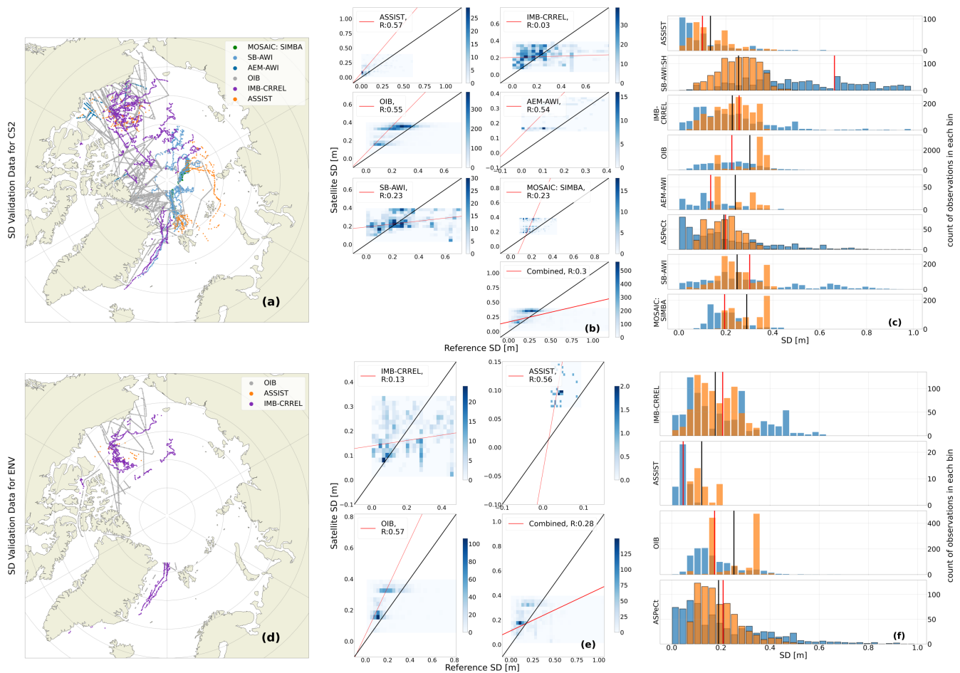
Figure 9. SD satellite and reference observation-measurements comparison for CryoSat-2 (a-c) and Envisat (d-f). Maps of overlap data are shown for NH in (a,d), associated scatterplots-scatter density plots with uncertainty weighted linear fits and associated correlation coefficients in the legend in (b,e) and histograms in (c,f). In the histograms the reference observations-measurements and satellite CDRs are marked with blue and orange, respectively, with associated average as black and red vertical lines. A black outline around the histogram bins are added to data from the SH
