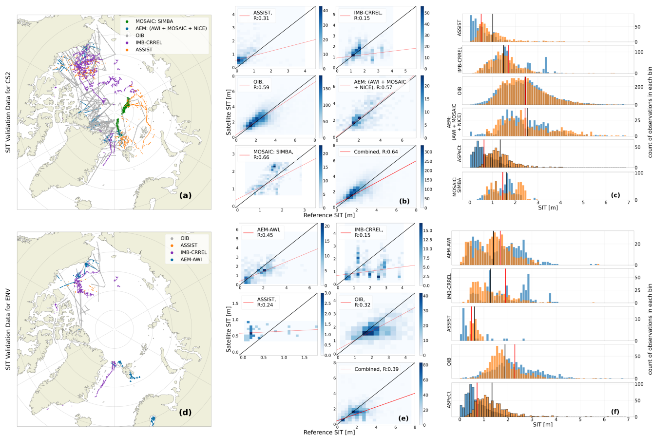
Figure 7. SIT satellite and reference observation-measurements comparison for CryoSat-2 (a-c) and Envisat (d-f). Maps of overlap data are shown for NH in (a,d), associated scatterplots with uncertainty weighted linear fits and associated correlation coefficients in the legend in (b,e) and histograms in (c,f). In the histograms the reference observations-measurements and satellite CDRs are marked with blue and orange, respectively, with associated average as black and red vertical lines. A black outline around the histogram bins are added to data from the SH
