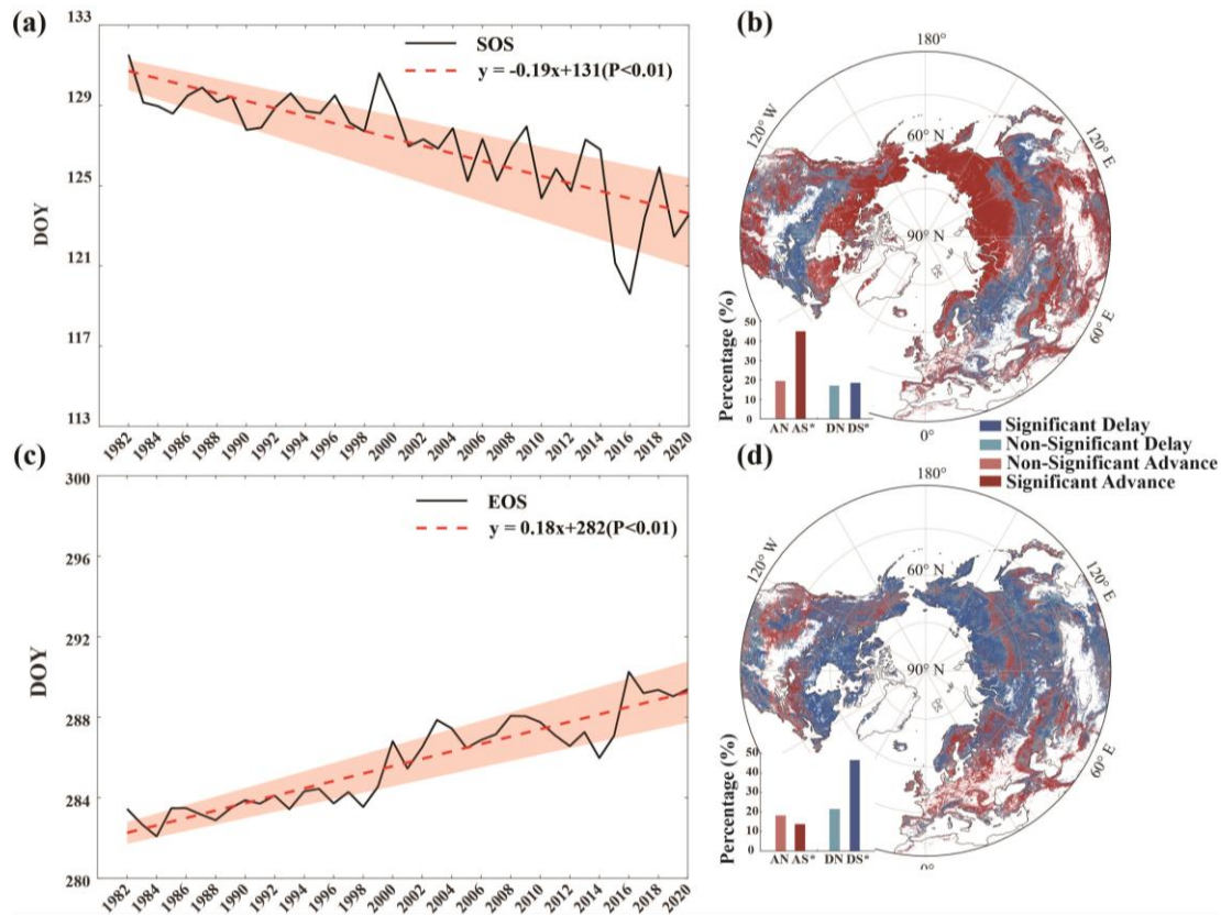
365 Figure 6: Temporal and spatial trends of the SOS and the EOS over the period 1982–2020 based on the merged dataset obtained using the REA method. (a) Temporal trend of the SOS over the period 1982–2020, (b) Spatial trend of the SOS over the period 1982–2020, (c) Temporal trend of the EOS over the period 1982–2020, (d) Spatial trend of the EOS over the period 1982–2020. The shaded area in (a) and (c) indicates uncertainty at one standard deviation, red lines in (a) and (c) are the fitting lines of average SOS/EOS dates for each year, and black lines are the average SOS/EOS date for each year. Significant delay (DS), non-significant delay (DN), significant advance (AS), non-significant advance (AN). 370
