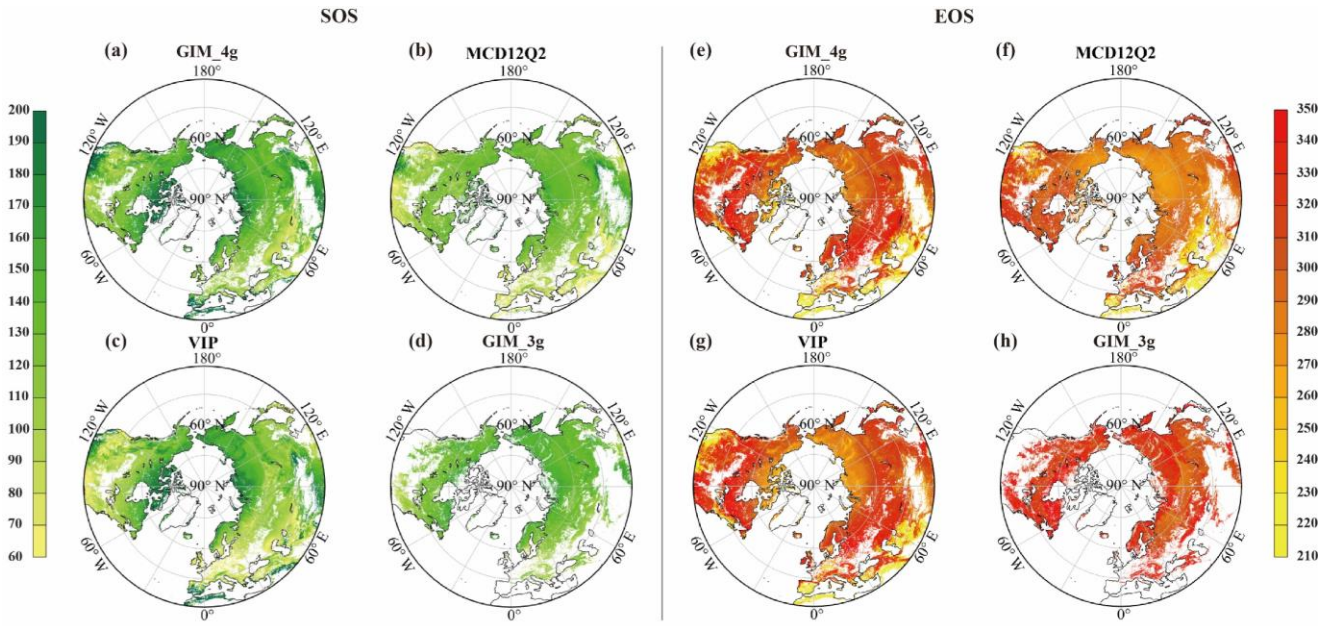
250 Figure 1: Spatial distribution of multiyear mean SOS and EOS dates from each phenology dataset: (a–d) multiyear mean SOS dates and (e–h) multiyear mean EOS dates derived from the GIM_4g, MCD12Q2, VIP, and GIM_3g datasets, respectively.
