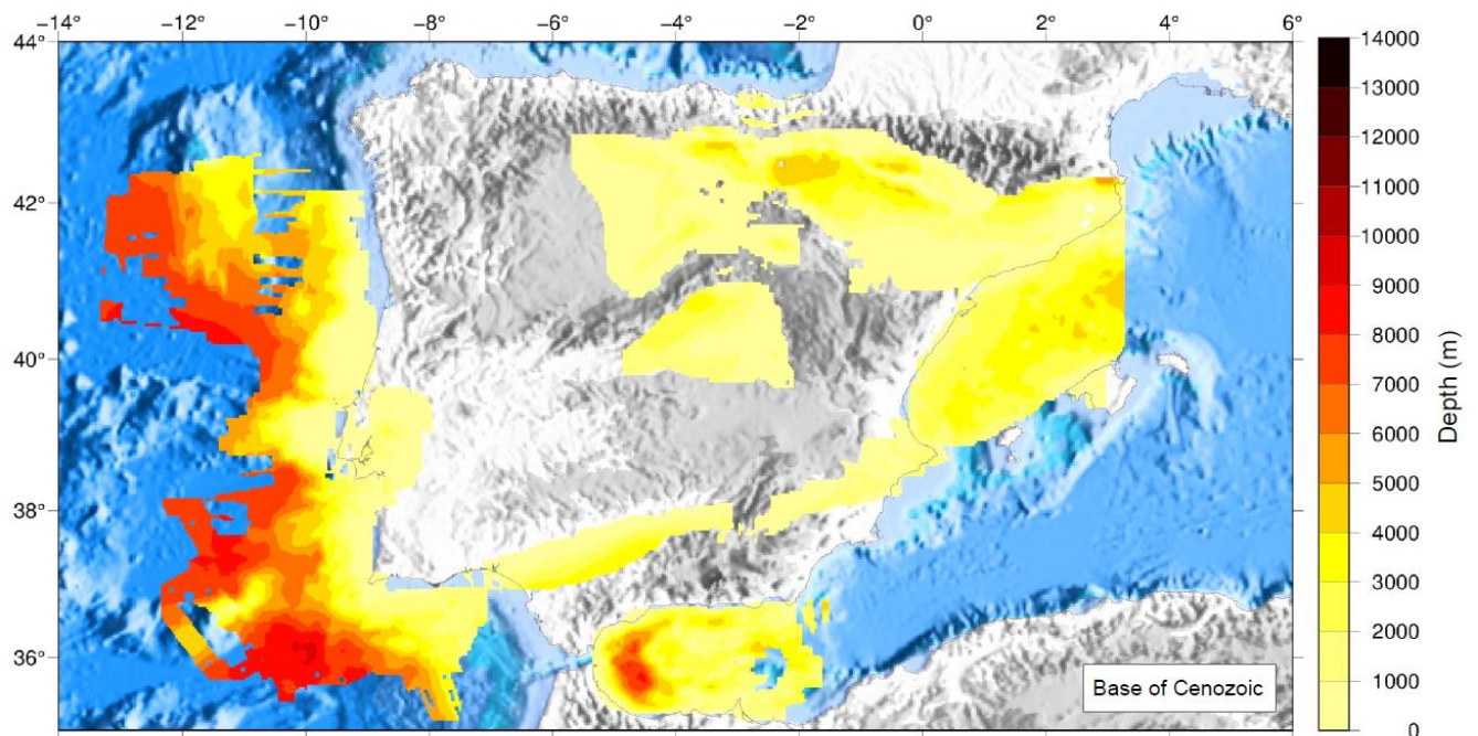
Figure 6 Offshore and onshore depth to the Base of Cenozoic. Main references from which data have 510 been gathered are shown in Table S1. Additional references can also be found throughout the text. Data from the Western Mediterranean have been taken from (Belluci et al., 2021, and references therein).
