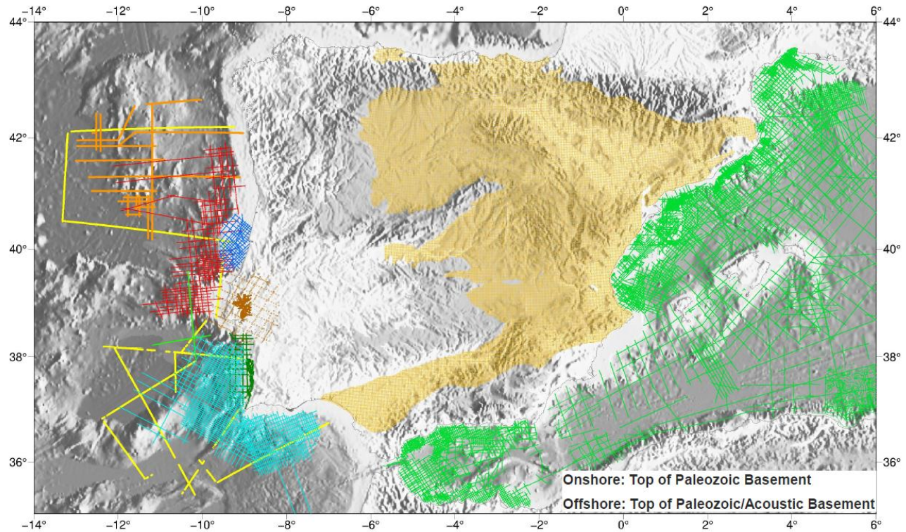
Figure 3 Offshore: Location of seismic profiles used for interpreting and gathering data for the Top of Paleozoic, or Acoustic Basement for most of the Western Mediterranean region. Exceptions are the Valencia Trough and the Alboran Basin (see Fig. 1 for location), where the Acoustic Basement corresponds to the Base of Cenozoic or the so-called Oligocene unconformity. Onshore: location of x,y,z
