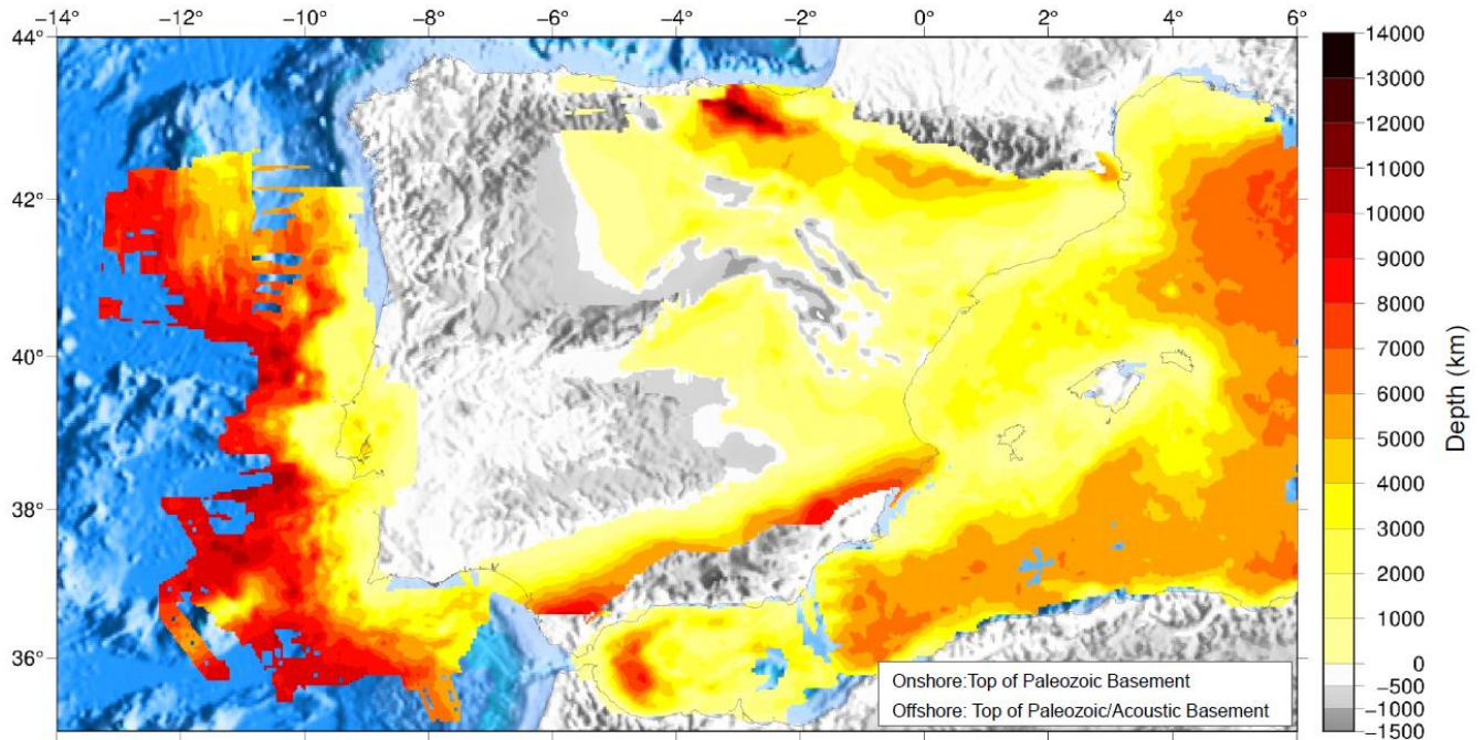
Figure 5 Offshore: Depth to the Top of Paleozoic, or Acoustic Basement for the majority of the Western Mediterranean region. Exceptions are the Valencia Trough and the Alboran Basin (see Fig. 1 for location), where the top of the basement corresponds to the Base of Cenozoic or the so-called Oligocene unconformity. Onshore: Depth to the Top of the Paleozoic Basement interpreted as the Paleozoic-cover sequence boundary or Hercynian discordance (Garcia-Lobón et al., 2020 and references therein).
