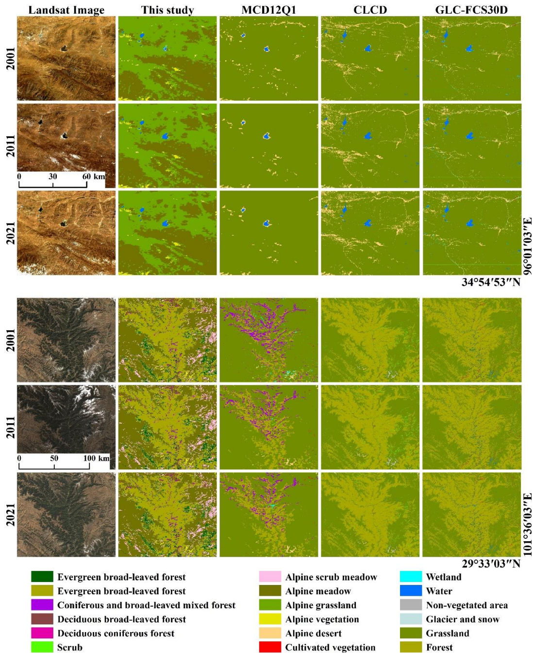
505 Figure 14. Comparison with the annual vegetation maps, MCD12Q1, CLCD, and GLC-FCS30D. (a): Region dominated by AM and AG. (b): Region dominated by EBF and AM
