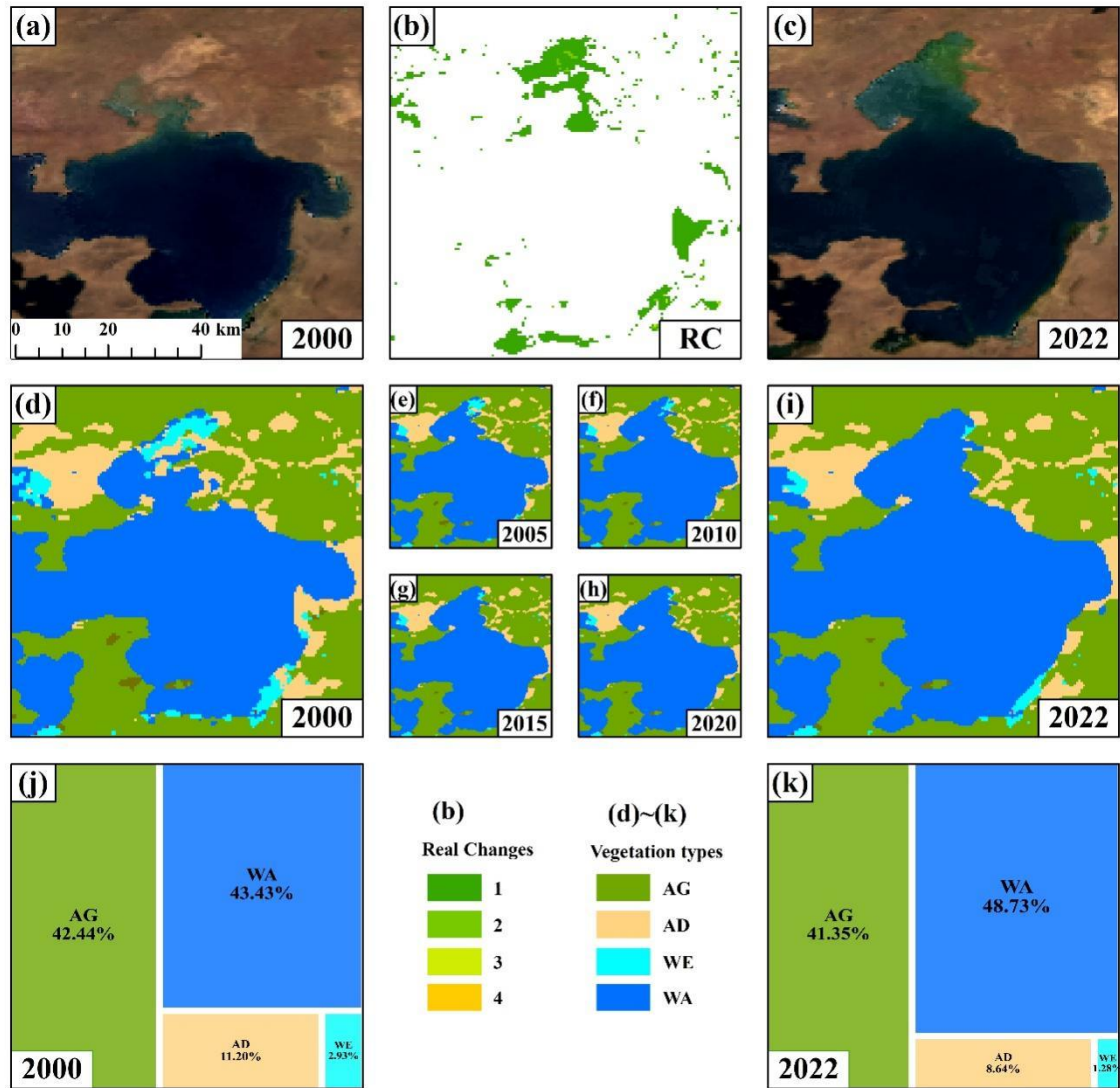
370 Figure 7. Annual vegetation cover changes in Area 1 [88.6985E, 31.5002N]. (a, c): Remote sensing images from 2000 and 2022, respectively. (b): Distribution and frequency of RC. (d-i): Annual vegetation maps for 2000, 2005, 2010, 2015, 2020, and 2022. (j, k): Area proportions of major vegetation types in 2000 and 2022, respectively.
