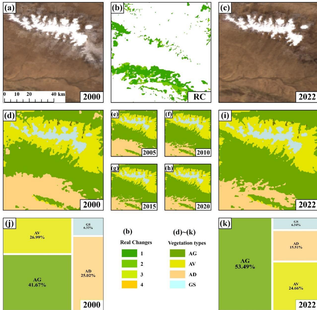
380 Figure 8. Annual vegetation cover changes in Area 2 [95.8644E, 37.6311N]. (a, c): Remote sensing images from 2000 and 2022, respectively. (b): Distribution and frequency of RC. (d-i): Annual vegetation maps for 2000, 2005, 2010, 2015, 2020, and 2022. (j, k): Area proportions of major vegetation types in 2000 and 2022, respectively.
