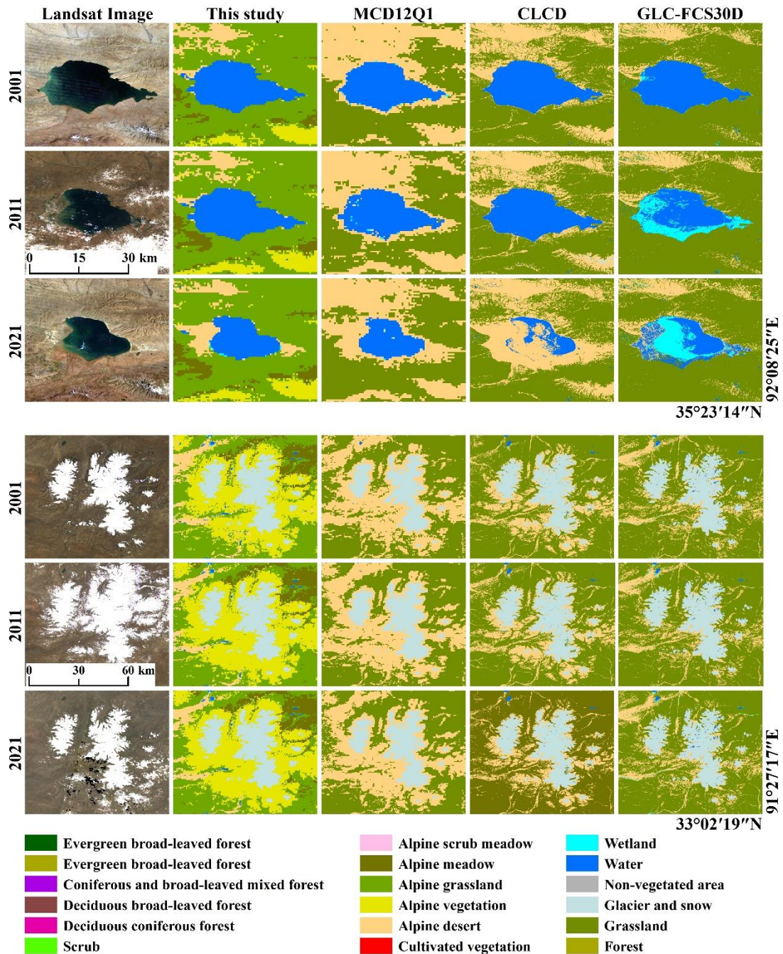
Figure 13. Comparison with the annual vegetation maps, MCD12Q1, CLCD, and GLC-FCS300. (a): Region dominated by WA and AG. (b): Region dominated by GA and AM.
