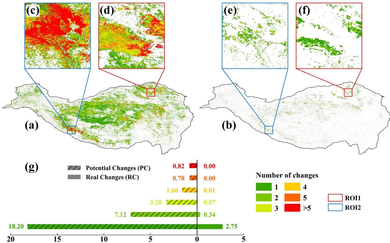
355 Figure 5. Overview of potential change (PC) and real change areas (RC) on the QTP from 2000 to 2022. (a-b) Distribution of PC and RC on the QTP; (c-f) PC and RC areas in ROI1 and ROI2; (g) Area statistics of PC and RC on the QTP.
