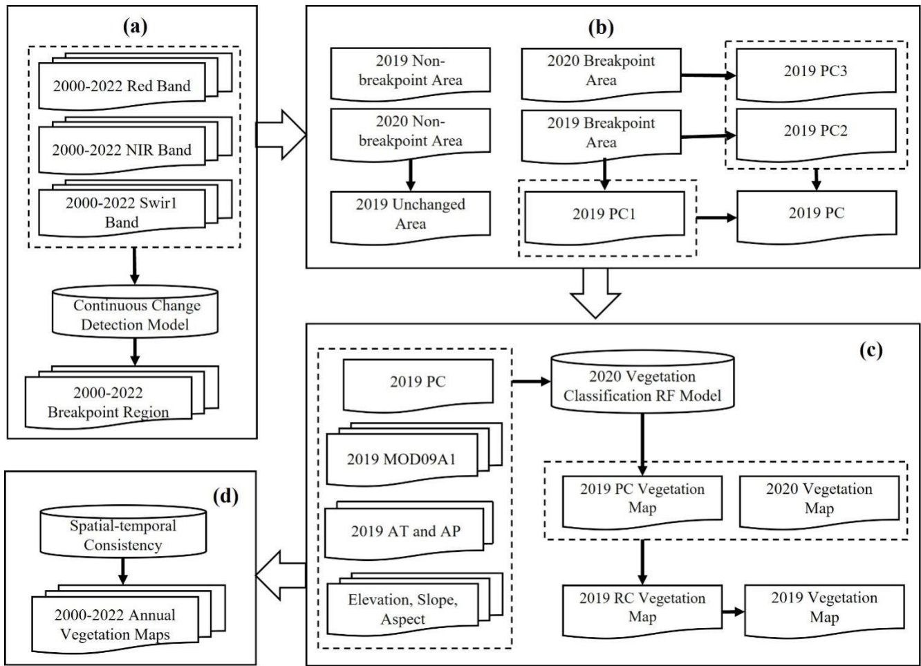
240 Figure 2. Vegetation mapping technology route at 500 m resolution on the QTP from 2000 to 2022 (dynamically updating the 2019 vegetation map with the 2020 vegetation map as a reference).
