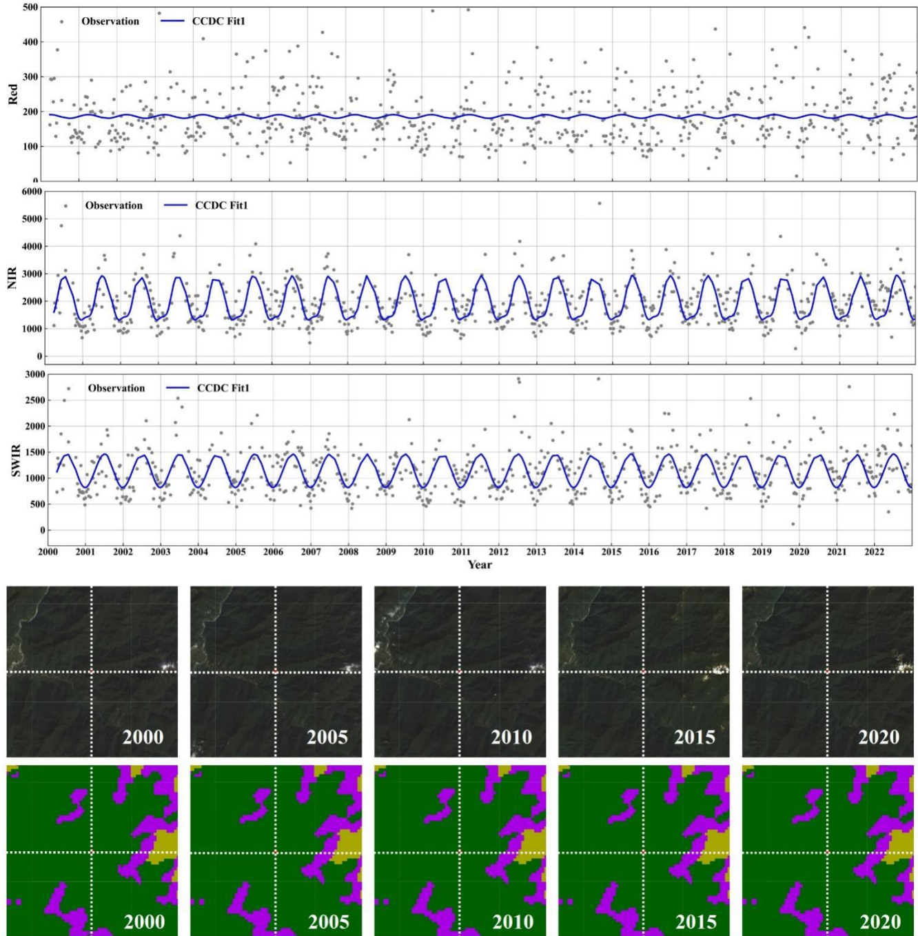
440 Figure 11. Validation of vegetation mapping: consistency of no change detection in forest sample [95.2794E, 28.7617N] by CCD, Landsat, and annual vegetation maps.
