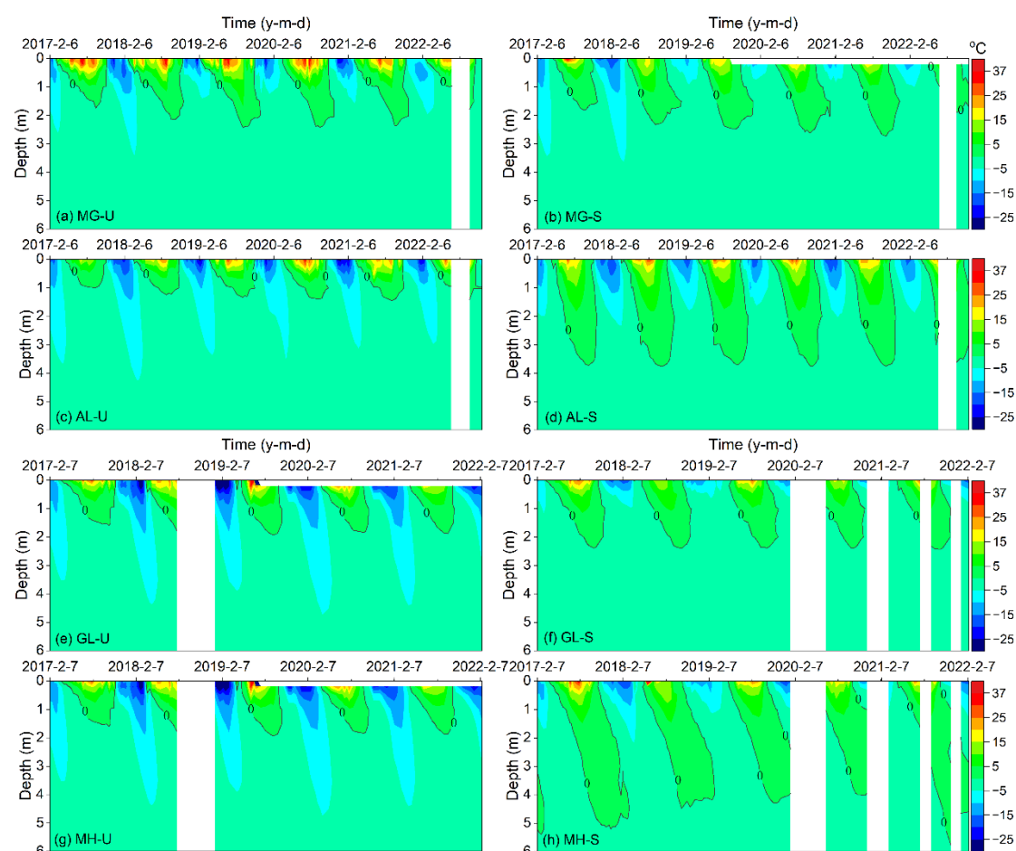
Figure 7. Variability of ground temperatures isotherms at eight sites in Mangui (MG), Alongshan (AL), Gulian (GL), and Mo'he (MH) on the western flank of the northern Da Xing'anling Mountains in Northeast China during 2017-2022.
