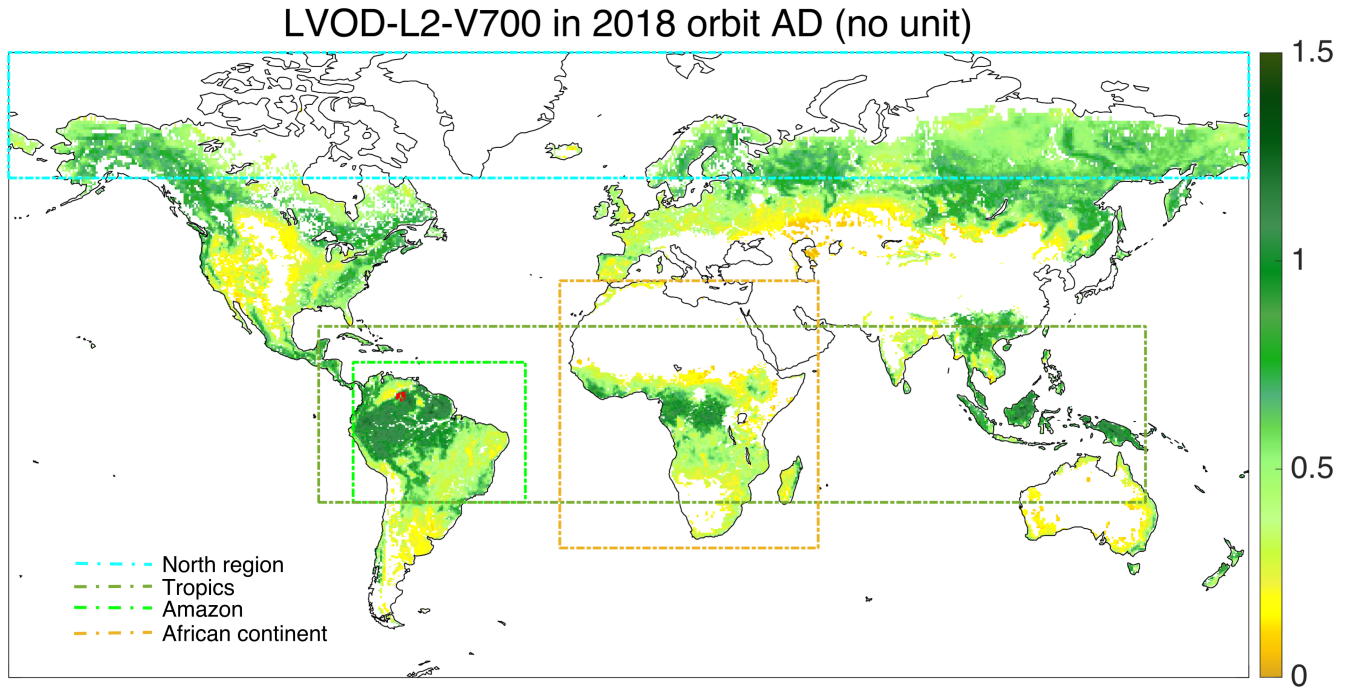
Figure 1. L-VOD from SMOS L2 v700 products averaged over 2018. Ascending and descending orbits are mixed. Values where RFI contamination is higher than 20 % or where the Chi2\_P is lower than 5 % or where the air temperature is below 0 °C, are filtered out. Pixels with an AGB reference value equals to 0 are also filtered out and outliers are discarded. The colored rectangles show the extent of the different regions (see Sect. 3.3.1 for more details about the regions) considered in the study
