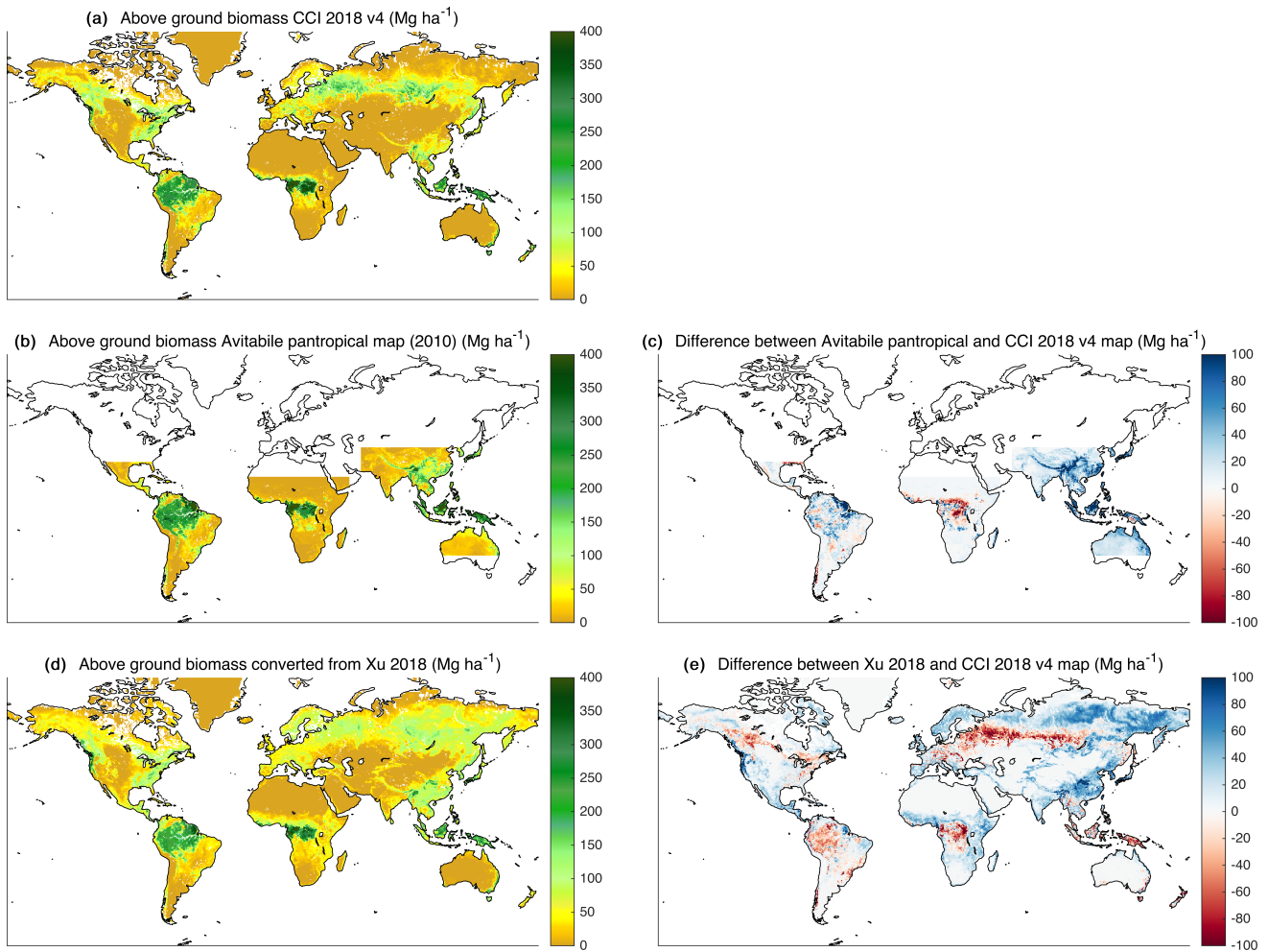
Figure 2. Reference maps used in this study and the spatial differences between them. (a) Above ground biomass from Santoro and Cartus (2023) CCI 2018 v4 (Santoro and Cartus, 2023), (b) Above ground biomass from Avitabile et al. (2016), (c) Above ground biomass difference between Avitabile et al. (2016) minus Santoro and Cartus (2023) CCI 2018 v4, (d) Above and below ground biomass (BGB) in 2018 from converted from Xu et al. (2021a), (e) Biomass difference between Xu et al. (2021a) minus Santoro and Cartus (2023) CCI 2018 v4. All units are in \text{Mg ha}^{-1} and all maps are resampled to the EASE 2 grid at 25 km
