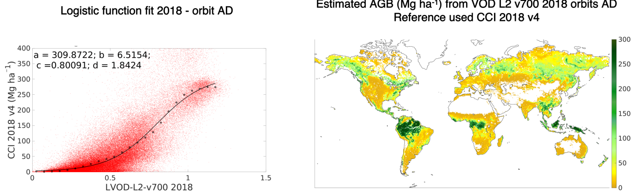
Figure 5. The left panel shows the parameter values and the mean logistic fit between the CCI 2018 AGB v4 map version 4 and the VOD from SMOS L2 products filtered and averaged over 2018. The right panel is the estimated AGB in Mg ha -1 by applying the logistic function with the estimated a , b , c and d parameters to the 2018 averaged VOD
