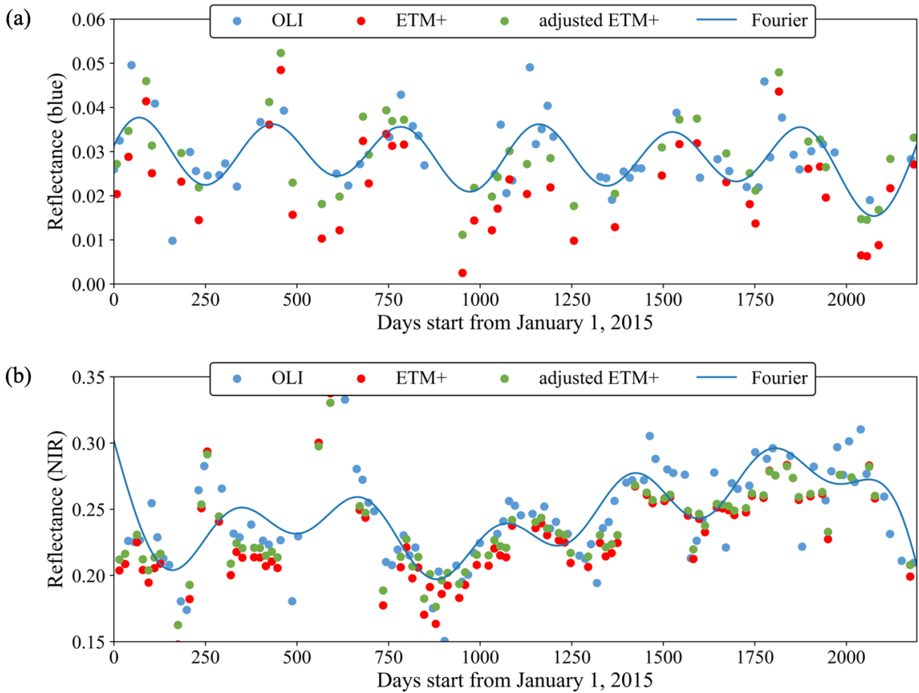
505 Figure 15: Time series of original and calibrated surface reflectance: (a) located at 23.2923° N, 68.7947° E; (b) located at 23.2923° N, 68.7947° E. The blue lines are the estimated curves of the OLI observations based on the Fourier approach (Dash et al., 2010; Shang and Zhu, 2019).
