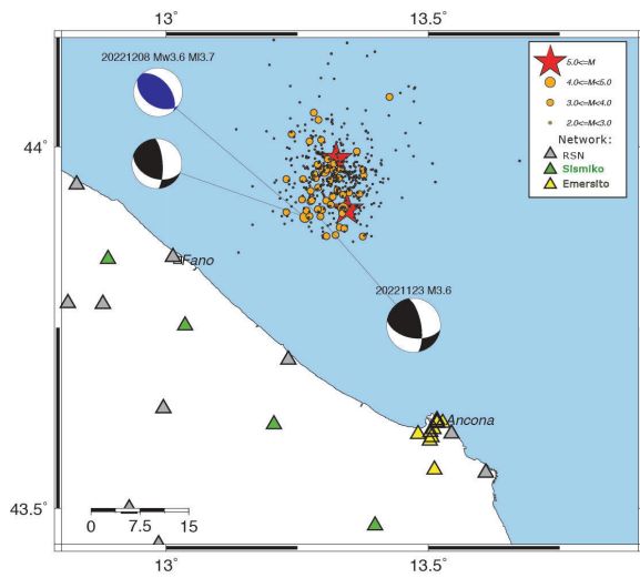
Figure 13. Left: Fault-Plane fit (FPFIT) focal solutions (black) for the earthquakes reported in Table 3. For the second event (id #33589291) the available Time Domain Moment Tensor (TDMT) is also shown in (blue); circles are M \geq 2.0 earthquakes of the seismic sequence (see the insert for the different sizes and the correspondence with difference magnitude), and red stars are M \geq 5.0 earthquakes.
