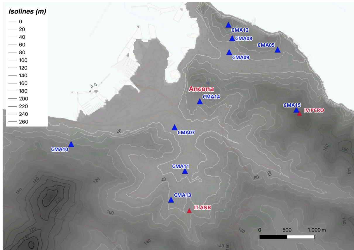
Figure 6. Topography map with isoline of the Ancona area. The blue triangles are most of the stations of the 6N EMERSITO Network, the orange triangles are the two permanent stations of RAN (IT.ANB) and RSN (IV.PCRO). Tarquini S., Isola I., Favalli M., Battistini A. (2007). © TINITALY, a digital elevation model of Italy with a 10 meters cell size (Version 1.0) [Data set]. Istituto Nazionale di Geofisica e Vulcanologia (INGV). https://doi.org/10.13127/tinitaly/1.0
