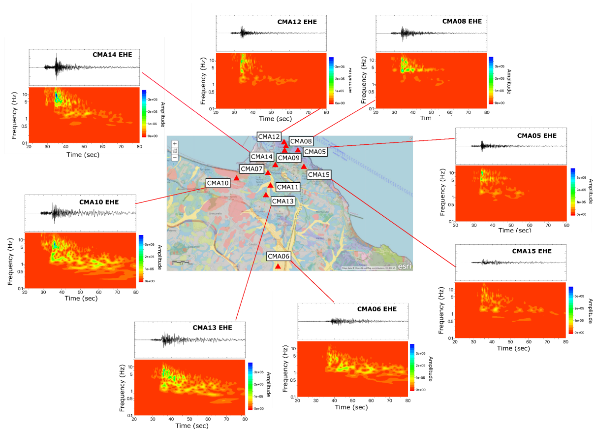
Figure 11. Time series and spectrograms of the M_w 3.9 earthquake (EHE components) occurred the 8th of December, 2022 at 07:08:18 UTC for some stations of the 6N network.
