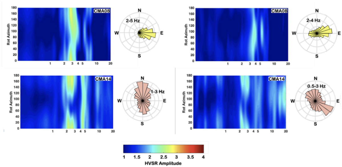
Figure 15. Directional amplification at two exemplificative stations: CMA08 (top) and CMA14 (bottom), by using seismic events (left-hand side) and ambient noise recordings (right-hand side). Rotated HVSR and HVNSR are graphed as contour plots, where the color scale is related to the amplitude level, the x-axis represents frequency, the y-axis the rotation angle ( 0^\circ and 180^\circ corresponding to N-S direction, 90^\circ to EW direction). The time-domain polarization analysis is summarized by means of circular histogram diagrams representing the polarization angle in the horizontal plane, obtained from filtered signals in the frequency band indicated in the rose diagram.
