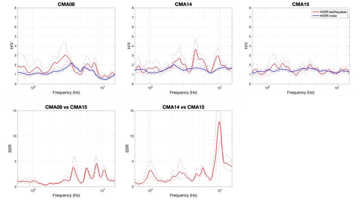
Figure 14. Top: HVNSR (blue lines) and HVSR (red lines) from HVNEA for CMA08, CMA14 and CMA15 stations. Bottom: SSR for CMA08 and CMA14 stations (red lines). For all plots, the solid lines are the averages, the dotted lines the average minus and plus one standard deviation.
