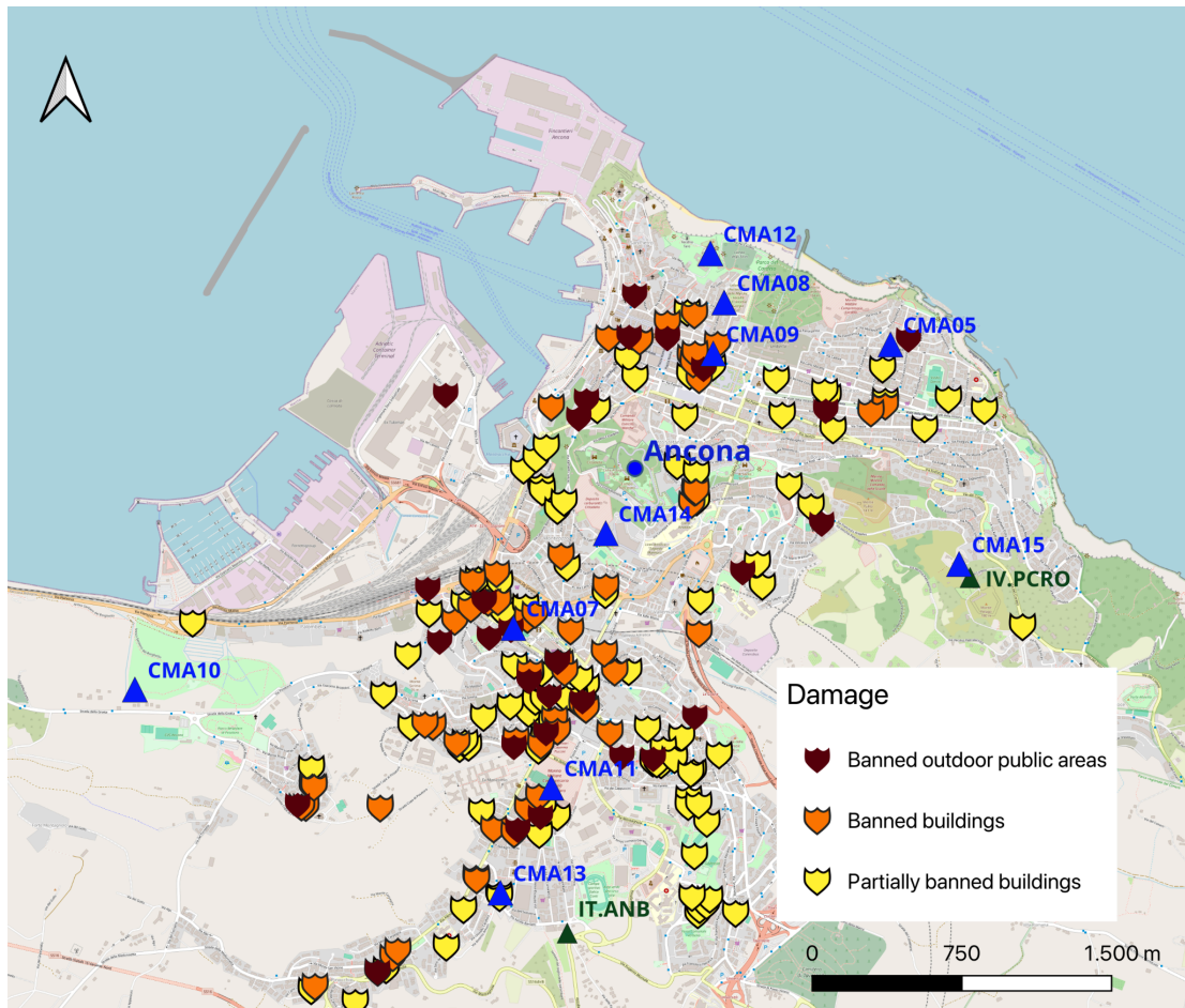
Figure 2. Map of Ancona municipality with the indication of damage as reported by the Fire Brigades. The blue triangles are most of the stations of the temporary network 6N installed by the EMERSITO working group. The green triangle are the two permanent stations installed at Ancona, IT.ANB and IV.PCRO, respectively.
