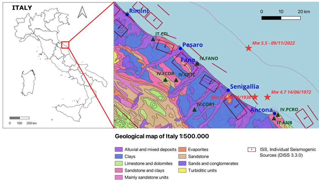
Figure 1. Left: Map of Italy, the red square indicates the Costa Marchigiana-Pesarese. Right: zoom of the study area with the geological map (1:500.000 scale) and the individual seismogenetic sources, showing: a) the epicenter of the M_w 5.5 of 09/11/2022 event, and the epicenters of the two strongest earthquakes occurred in the previous century that affected Ancona significantly (red stars); b) the main cities in the Adriatic coast (blue dots); c) the accelerometric stations (green triangles) of RAN and RSN seismic networks closest to the M_w 5.5 event. The individual seismogenetic sources are taken from DISS Working Group (2021).
