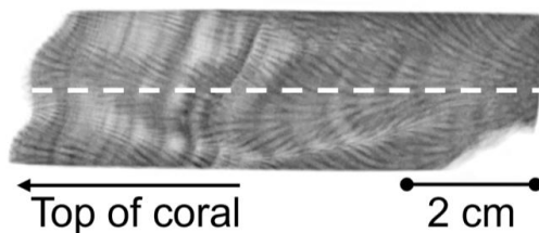
Figure C6. X-radiograph (positive) of alternate slice of OTI 1-3 (AR24OTI02) coral. Dashed white line indicates the estimated track analysed by LA-ICP-MS for the record included in AR24OTI02. X-radiographs by PRP Diagnostic Imaging Wollongong.
