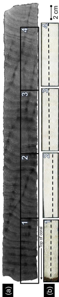
Figure C1. PET12 (EL19OTI01) (a) X-radiograph (negative) of PET12 (EL19OTI01) coral. Black boxes indicate the 4 pieces analysed and are labelled with the piece number (1–4 in the top of the box). (b) Photos of PET12 pieces 1–4 and dashed black lines indicate the track analysed by LA-ICP-MS for each section of the record included in EL19OTI01. X-radiograph and photos supplied 595 by J. Mallela.
