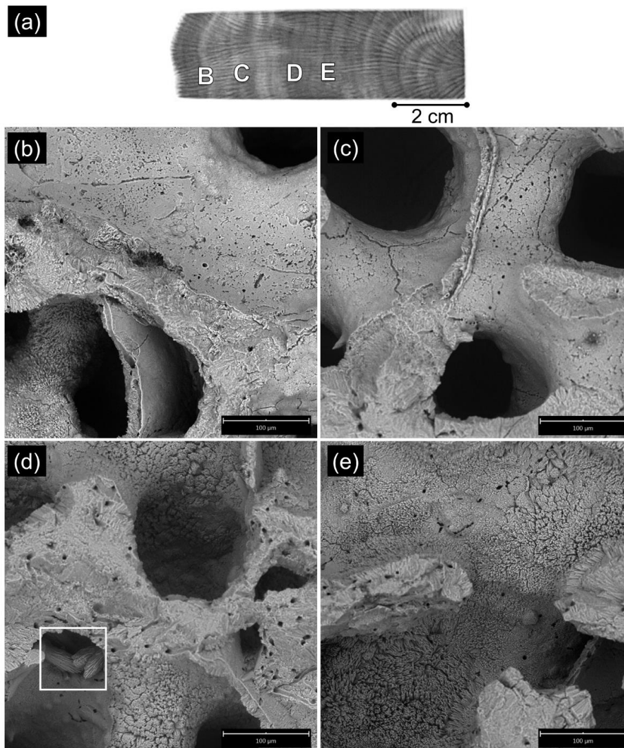
770 Figure C9. OTI 3-1 (AR24OTI03) SEM images. (a) Approximate locations of SEM images labelled B–E on coral X-ray. (b) to (e) Select SEM images from OTI 3-1; (b) Secondary aragonite needles (0–10 \mu\text{m} ) in lower left of image and possible low Mg-calcite cement on coral surface in upper right of image. Evidence of micro-borers, (c) No secondary aragonite. Evidence of micro-borers and possible minor dissolution of coral surface, (d) 100% cover with secondary aragonite needles (0–15 \mu\text{m} ) with evidence of micro-borers. High Mg-calcite splays occur in pore space; marked by white box, (e) 100% cover with secondary aragonite needles (~5–15 \mu\text{m} ) with evidence of micro-borers. Scale bar indicates 100 \mu\text{m} (b–e).
