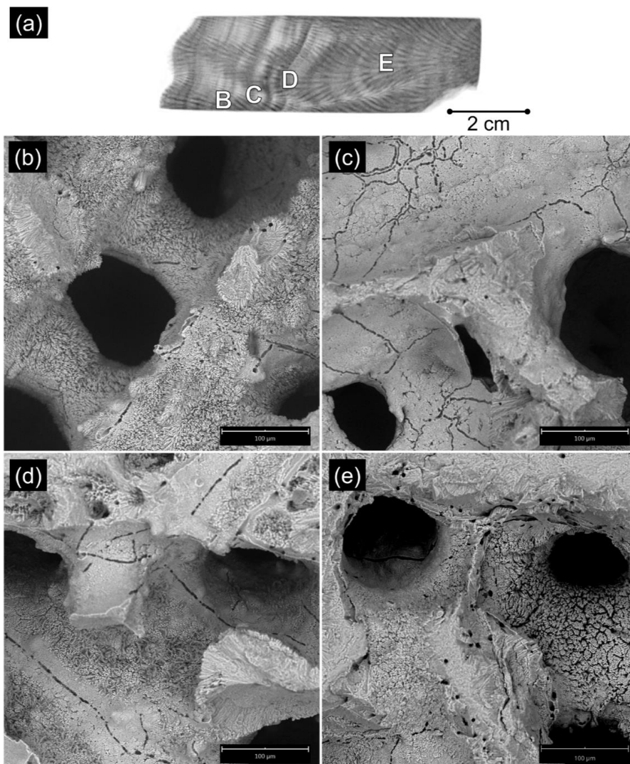
Figure C8. OTI 1-3 (AR24OTI02) SEM images. (a) Approximate locations of SEM images labelled B–E on coral X-radiograph. (b) to (e) Select SEM images from OTI 1-3; (b) low-level diagenetic alteration with 100% cover of secondary aragonite needles of 5–15 µm and micro-borer tracks, (c) No secondary aragonite needles, with evidence of dissolution and micro-borers tracks, (d) Evidence of micro-borer tracks and possibly dissolution. Secondary aragonite needles and calcite crystals (0–10 µm), (e) 90% surface covered by secondary aragonite needles, left side of coral needles are \leq 5 µm and right side of coral needles are ~5–15 µm. Evidence of micro-borers visible. Scale bar indicates 100 µm (b–e).
