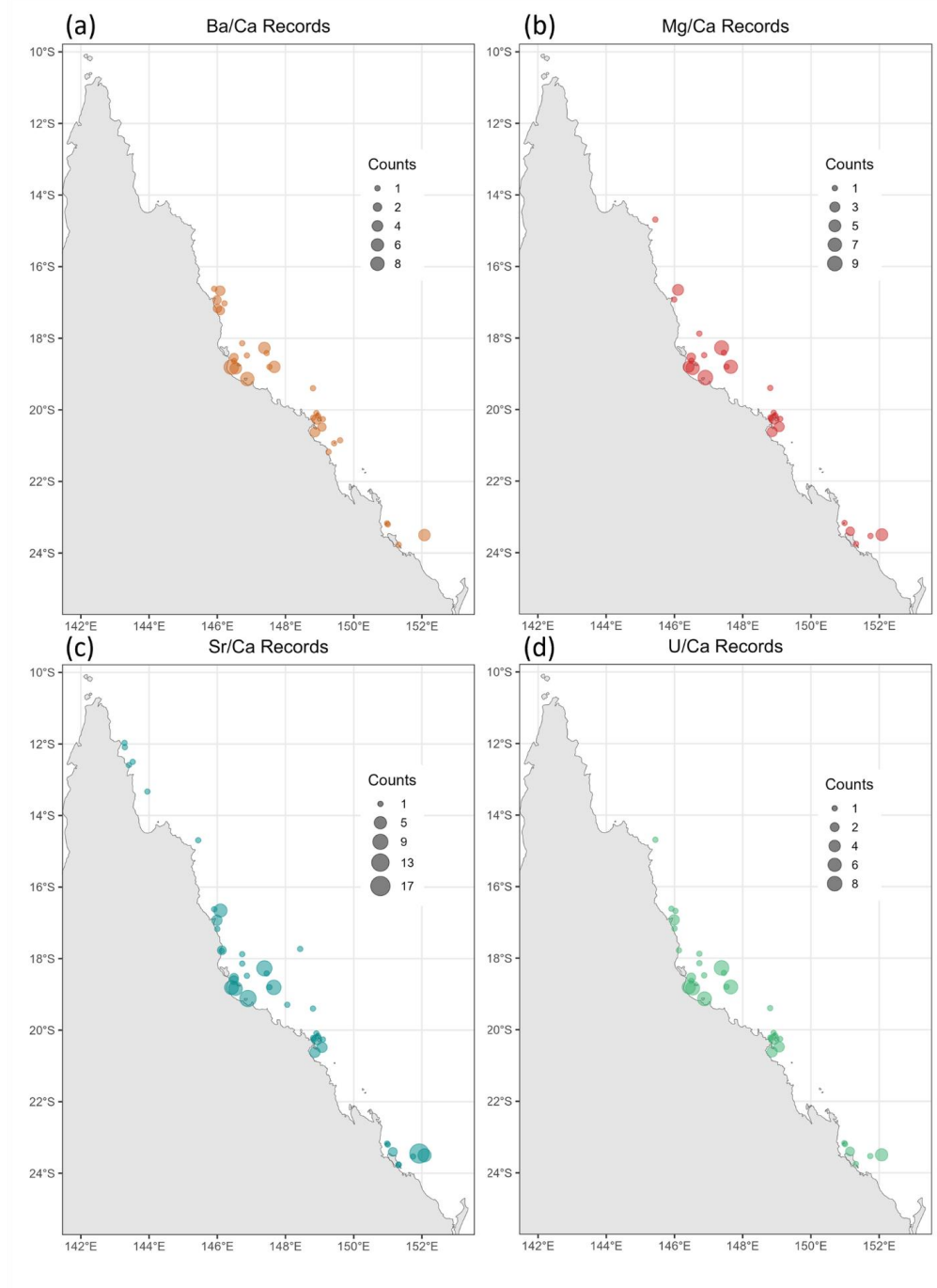
Figure 4. Location map of GBRCD records for common major trace element ratios; (a) Ba/Ca, (b) Mg/Ca, (c) Sr/Ca and (d) U/Ca. The size of the point indicates the number of records, and is specific to each map.
