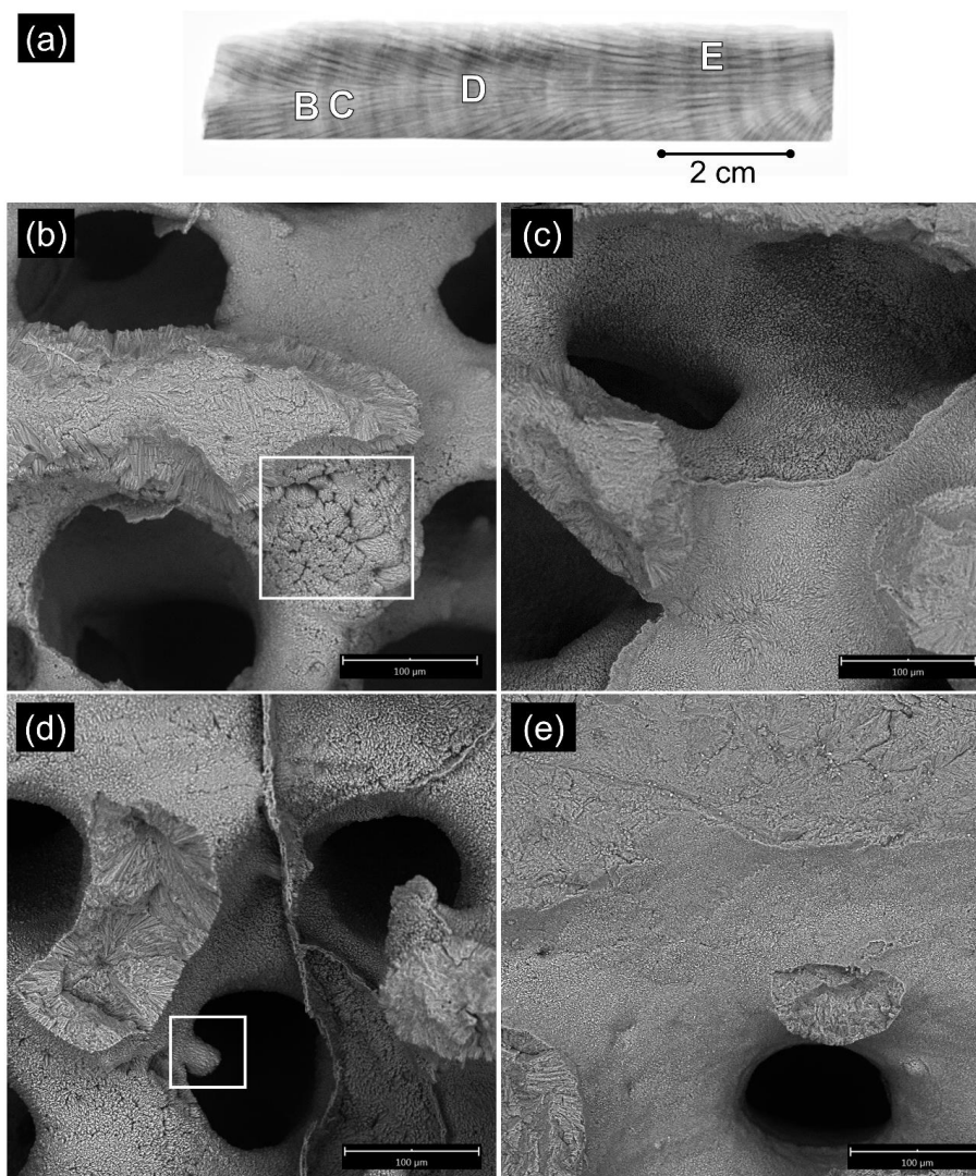
795 Figure C11. OTI4_6C (OTI-4-19; AR24OTI04) SEM images. (a) Approximate locations of SEM images labelled B–E on coral X-ray. (b) to (e) Select SEM images from OTI4_6C (AR24OTI04); (b) 100% cover of secondary aragonite needles generally <10 μm, but section with uneven surface (marked by white box) indicates ~10–20 μm crystals, (c) 100% cover of secondary aragonite needles of <10 μm, (d) 100% cover of secondary aragonite needles of 5–10 μm. Includes secondary aragonite covering likely fungal growth or part of borer tube that occurred when coral was alive (marked by white box), (e) 80% cover of trace (<5 μm) crystals of secondary aragonite. Scale bar indicates 100 μm (b–e).
