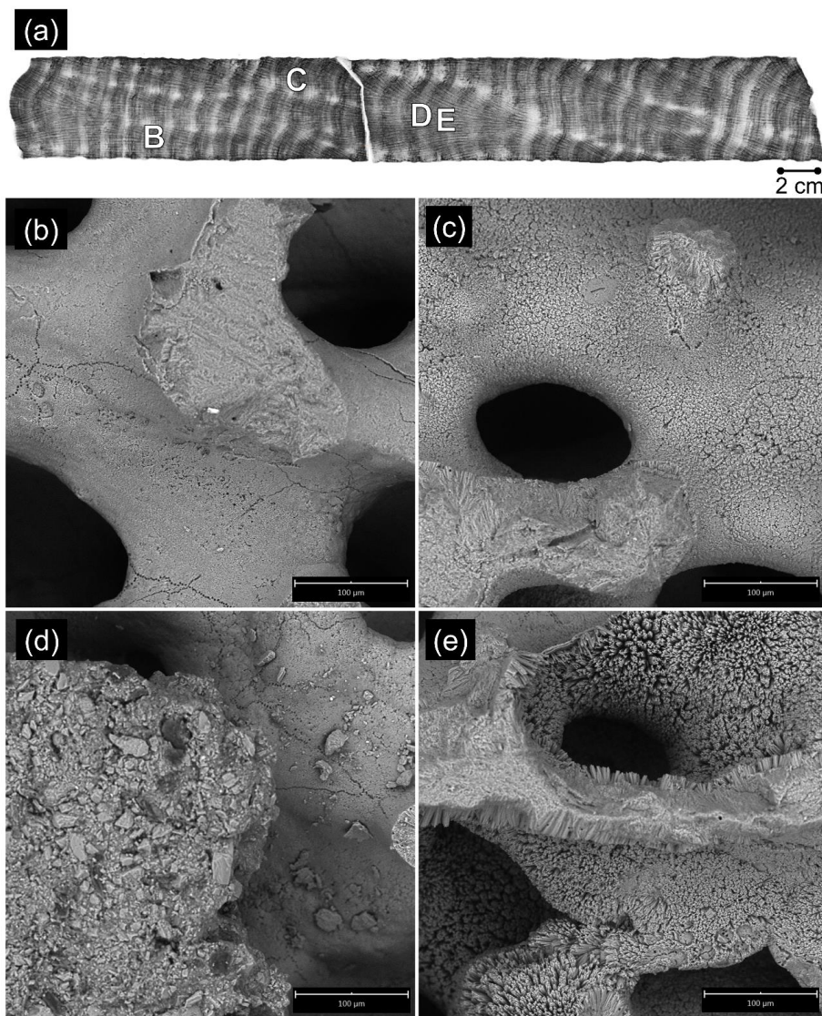
600 605 Figure C2. PET12 (EL180TI01) SEM images from alternate slice of PET12 coral. (a) Approximate locations of SEM images labelled B–E on coral X-radiograph. X-radiograph by PRP Diagnostic Imaging Wollongong. (b) to (e) Select SEM images from PET12 (EL190TI01); (b) No secondary aragonite. Evidence of micro-borers, (c) Low-level diagenetic alteration with 100% cover of secondary aragonite needles \leq 5 \mu\text{m} and evidence of micro-borers, (d) Bioclastic cement plug above relatively pristine coral surface with cement chip (e) 90% cover of secondary aragonite needles of 5–20 \mu\text{m} . Scale bar indicates 100 \mu\text{m} (b–e).
