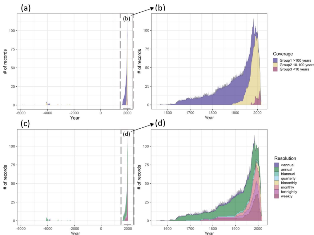
Figure 3. Temporal coverage of records in the GBRCDB colour coded by (a) record coverage Group 1–3 as per Table 6 (1 – records >100 years; 2 – records >10 – <100 years; 3 – records <10 years), (b) subset of (a) showing only records since 1550 CE, (c) nominal resolution as per Table 11 (see figure legend) (records with “_uneven” nominal resolution were combined with even resolution records), and (d) subset of (c) showing only records since 1550 CE. The ‘spikiness’ visible in (b) Group 1 & (d) >annual resolution records is due to the combination of biennial and quinquennial resolution records.
