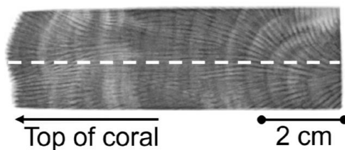
Figure C7. X-radiograph (positive) of alternate slice of OTI 3-1 (AR24OTI03) coral. Dashed white line indicates the estimated track analysed by LA-ICP-MS for the record included in AR24OTI03. X-radiographs by PRP Diagnostic Imaging Wollongong.
