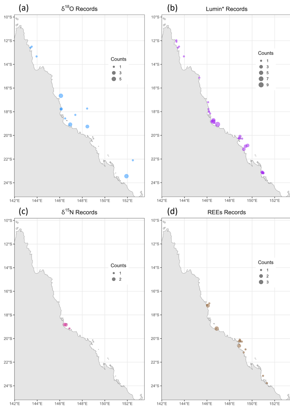
465 Figure 5. Location map of GBRC D records for (a) \delta^{18}\text{O} , (b) luminescence (Lumin), (c) \delta^{15}\text{N} and (d) Rare Earth Elements (REEs). The size of the point indicates the number of records, and is specific to each map. Note that Lumin* includes all the methods included in the GBRC D for measuring luminescence.
