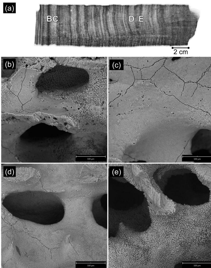
730 Figure C5. GUT12 (AR24OTI01) SEM images (a) Approximate locations of SEM images labelled B–E on coral X-radiograph. (b) to (e) Select SEM images from GUT12; (b) Secondary aragonite needles <5\ \mu\text{m} patchy cover of coral surface (~50%), (c) No secondary aragonite needles. Evidence of micro-borers, (d) low-level diagenetic alteration with 100% cover of secondary aragonite needles <5\ \mu\text{m} , (e) low-level diagenetic alteration with 100% cover of secondary aragonite needles of 5–15 \mu\text{m} . Scale bar indicates 100 \mu\text{m} (b–e).
