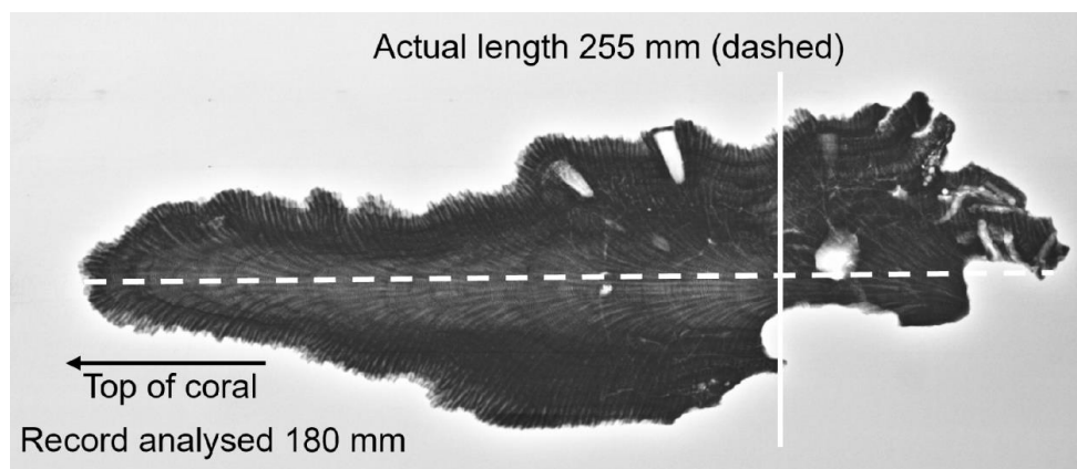
Figure C3. X-radiograph (positive) of Dip-04 (AR24DIP01) coral. White dashed line indicates the track analysed with white solid line the end of record section. X-radiograph supplied by T. Razak.
