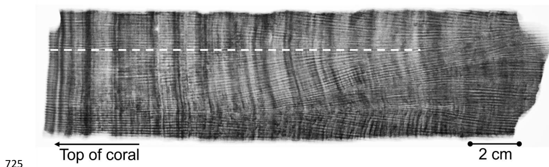
Figure C4. X-radiograph (positive) of GUT12 (AR24OTI01) coral. Dashed white line indicates the track analysed by ICP-AES for the record included in AR24OTI01. X-radiographs by PRP Diagnostic Imaging Wollongong.
