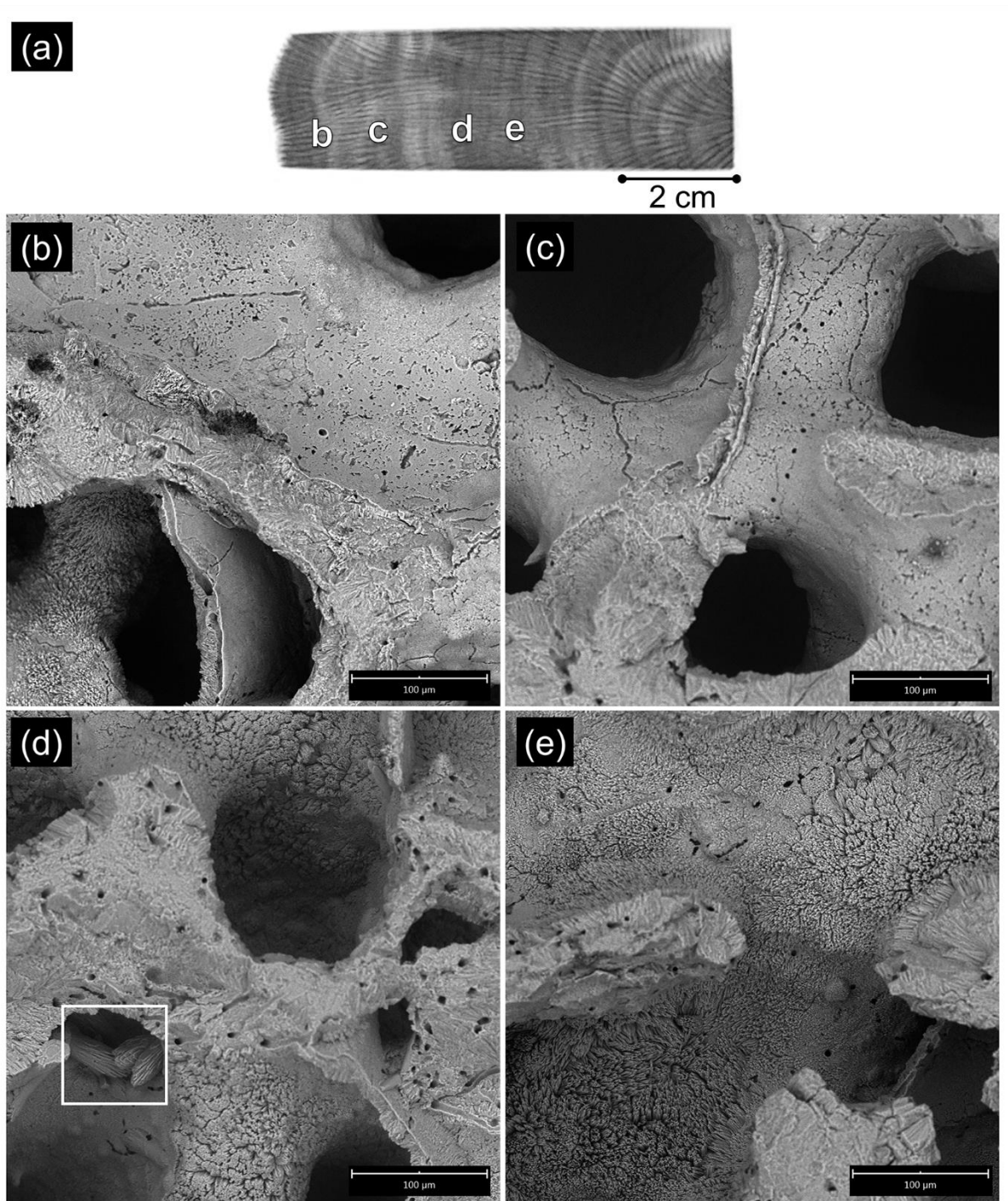
Figure C9. OTI 3-1 (AR24OTI03) SEM images. (a) Approximate locations of SEM images labelled b–e on coral X-ray. (b) to (e) Select SEM images from OTI 3-1; (b) Secondary aragonite needles (0–10 \mu\text{m} ) in lower left of image and possible low Mg-calcite cement on coral surface in upper right of image. Evidence of micro-borers, (c) No secondary aragonite. Evidence of micro-borers and possible minor dissolution of coral surface, (d) 100% cover with secondary aragonite needles (0–15 \mu\text{m} ) with evidence of micro-borers. High Mg-calcite splays occur in pore space (marked by white box), (e) 100% cover with secondary aragonite needles (~5–15 \mu\text{m} ) with evidence of micro-borers. Scale bar indicates 100 \mu\text{m} (b–e).
