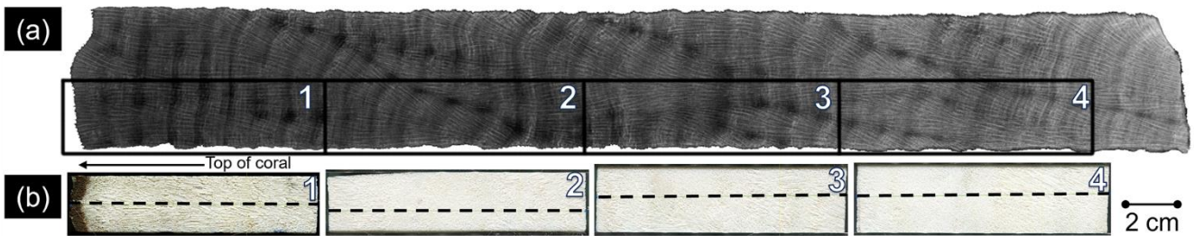
625 Figure C1. PET12 (EL190TI01) (a) X-radiograph (negative) of PET12 (EL190TI01) coral. Black boxes indicate the 4 pieces analysed and are labelled with the piece number (1–4 in the top of the box). (b) Photos of PET12 pieces 1–4 and dashed black lines indicate the track analysed by LA-ICP-MS for each section of the record included in EL190TI01. X-radiograph and photos supplied by J. Mallela.
