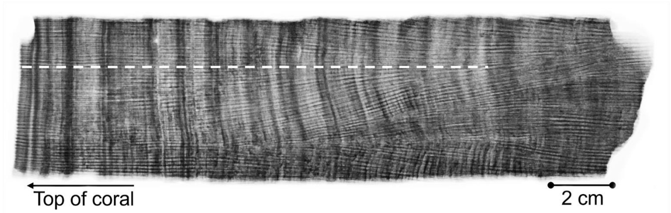
760 Figure C4. X-radiograph (positive) of GUT12 (AR24OTI01) coral. Dashed white line indicates the track analysed by ICP-AES for the record included in AR24OTI01. X-radiographs by PRP Diagnostic Imaging Wollongong.
