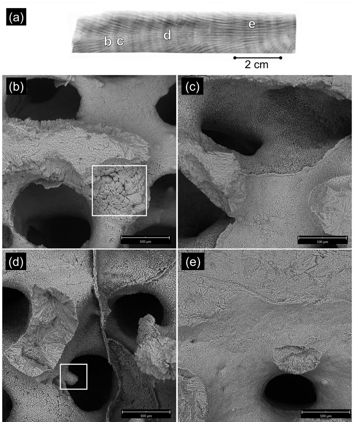
825 Figure C11. OTI4_6C (OTI-4-19; AR24OTI04) SEM images. (a) Approximate locations of SEM images labelled b–e on coral X-ray. (b) to (e) Select SEM images from OTI4_6C (AR24OTI04); (b) 100% cover of secondary aragonite needles generally <10 \mu\text{m} , but section with uneven surface (marked by white box) indicates ~10–20 \mu\text{m} crystals, (c) 100% cover of secondary aragonite needles of <10 \mu\text{m} , (d) 100% cover of secondary aragonite needles of 5–10 \mu\text{m} . Includes secondary aragonite covering likely fungal growth or part of borer tube that occurred when coral was alive (marked by white box), (e) 80% cover of trace (<5 \mu\text{m} ) crystals of secondary 830 aragonite. Scale bar indicates 100 \mu\text{m} (b–e).
