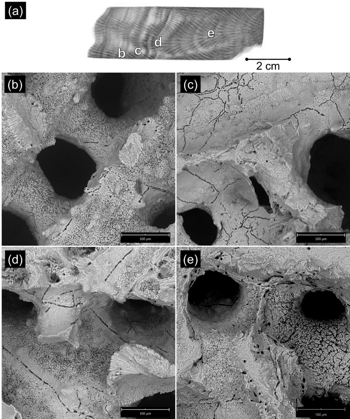
795 Figure C8. OTI 1-3 (AR24OTI02) SEM images. (a) Approximate locations of SEM images labelled b–e on coral X-radiograph. (b) to (e) Select SEM images from OTI 1-3; (b) low-level diagenetic alteration with 100% cover of secondary aragonite needles of 5–15 μm and evidence of micro-borers, (c) No secondary aragonite needles, with evidence of dissolution and micro-borers, (d) Evidence of micro-borers and possibly dissolution. Secondary aragonite needles and calcite crystals (0–10 μm), (e) 90% surface covered by secondary aragonite needles, left side of coral needles are \leq 5 μm and right side of coral needles are \sim 5 –15 μm. Evidence of micro-borers visible. Scale bar indicates 100 μm (b–e).
