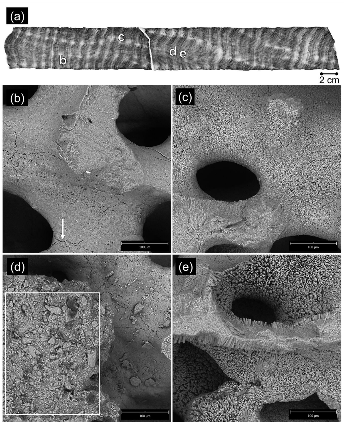
Figure C2. PET12 (EL180TI01) SEM images from alternate slice of PET12 coral. (a) Approximate locations of SEM images labelled b–e on coral X-radiograph. X-radiograph by PRP Diagnostic Imaging Wollongong. (b) to (e) Select SEM images from PET12 (EL190TI01); (b) No secondary aragonite. Evidence of micro-borers (example noted by white arrow), (c) Low-level diagenetic alteration with nearly 100% cover of secondary aragonite needles \leq 5 \mu\text{m} and evidence of micro-borers, (d) Bioclastic cement plug (marked by white box) above relatively pristine coral surface with cement chips and evidence of micro-borers, (e) 90% cover of secondary aragonite needles of 5–20 \mu\text{m} . Scale bar indicates 100 \mu\text{m} (b–e).
