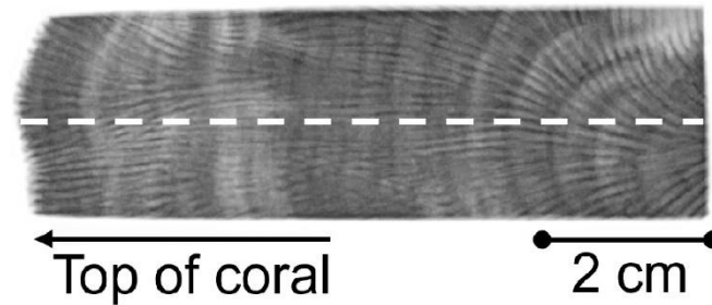
790 Figure C7. X-radiograph (positive) of alternate slice of OTI 3-1 (AR24OTI03) coral. Dashed white line indicates the estimated track analysed by LA-ICP-MS for the record included in AR24OTI03. X-radiographs by PRP Diagnostic Imaging Wollongong.
