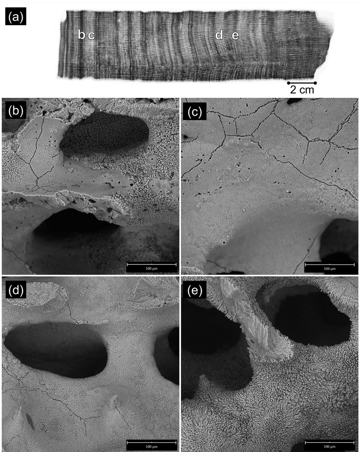
765 Figure C5. GUT12 (AR24OTI01) SEM images (a) Approximate locations of SEM images labelled b–e on coral X-radiograph. (b) to (e) Select SEM images from GUT12; (b) Secondary aragonite needles \leq 5 \mu\text{m} patchy cover of coral surface (~50%) and evidence of micro-borers, (c) No secondary aragonite needles. Evidence of micro-borers, (d) low-level diagenetic alteration with 100% cover of secondary aragonite needles < 5 \mu\text{m} , (e) low-level diagenetic alteration with 100% cover of secondary aragonite needles of 5-15 \mu\text{m} . Scale bar indicates 100 \mu\text{m} (b-e).
