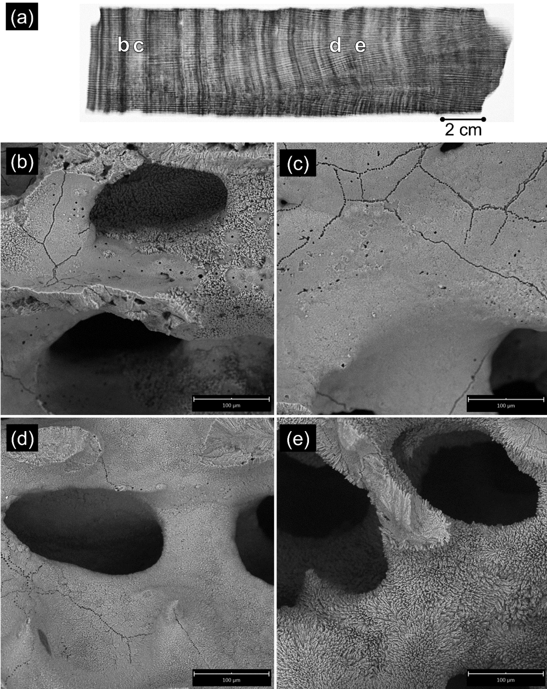
760 Figure C5. GUT12 (AR24OTI01) SEM images (a) Approximate locations of SEM images labelled b–e on coral X-radiograph. (b) to (e) Select SEM images from GUT12; (b) Secondary aragonite needles \leq 5 \mu\text{m} patchy cover of coral surface (~50%) and evidence of micro-borers, (c) No secondary aragonite needles. Evidence of micro-borers, (d) low-level diagenetic alteration with 100% cover of secondary aragonite needles < 5 \mu\text{m} , (e) low-level diagenetic alteration with 100% cover of secondary aragonite needles of 5-15 \mu\text{m} . Scale bar indicates 100 \mu\text{m} (b-e).
