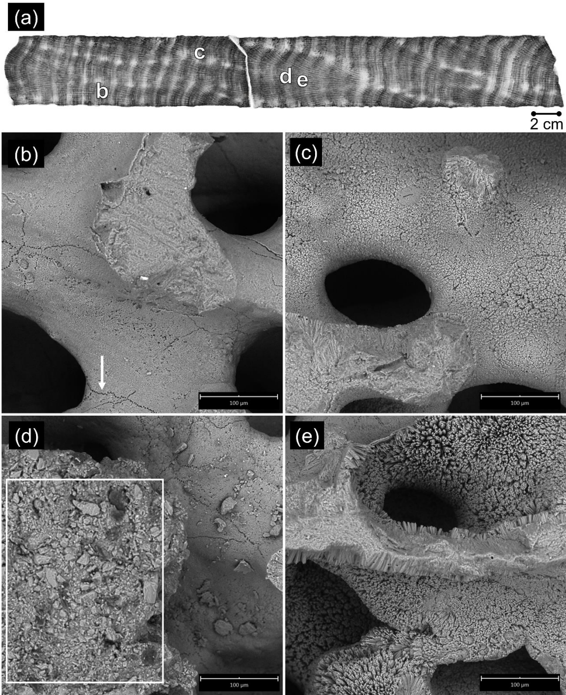
625 Figure C2. PET12 (EL180TI01) SEM images from alternate slice of PET12 coral. (a) Approximate locations of SEM images labelled b–e on coral X-radiograph. X-radiograph by PRP Diagnostic Imaging Wollongong. (b) to (e) Select SEM images from PET12 (EL190TI01); (b) No secondary aragonite. Evidence of micro-borers (example noted by white arrow), (c) Low-level diagenetic alteration with nearly 100% cover of secondary aragonite needles \leq 5 \mu\text{m} and evidence of micro-borers, (d) Bioclastic cement plug (marked by white box) above relatively pristine coral surface with cement chips and evidence of micro-borers, (e) 90% cover of 630 secondary aragonite needles of 5–20 \mu\text{m} . Scale bar indicates 100 \mu\text{m} (b–e).
