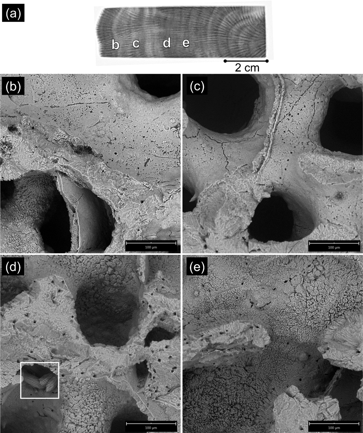
800 Figure C9. OTI 3-1 (AR24OTI03) SEM images. (a) Approximate locations of SEM images labelled b–e on coral X-ray. (b) to (e) Select SEM images from OTI 3-1; (b) Secondary aragonite needles (0–10 μm) in lower left of image and possible low Mg-calcite cement on coral surface in upper right of image. Evidence of micro-borers, (c) No secondary aragonite. Evidence of micro-borers and possible minor dissolution of coral surface, (d) 100% cover with secondary aragonite needles (0–15 μm) with evidence of micro-borers. High Mg-calcite splays occur in pore space (marked by white box), (e) 100% cover with secondary aragonite needles (~5–15 μm) with evidence of micro-borers. Scale bar indicates 100 μm (b–e).
