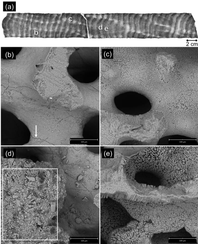
Figure C2. PET12 (EL180TI01) SEM images from alternate slice of PET12 coral. (a) Approximate locations of SEM images labelled b – e on coral X-radiograph. X-radiograph by PRP Diagnostic Imaging Wollongong. (b) to (e) Select SEM images from PET12 (EL190TI01); (b) No secondary aragonite. Evidence of micro-borers (example noted by white arrow), (c) Low-level diagenetic alteration with nearly 100% cover of secondary aragonite needles \leq 5 \mu\text{m} and evidence of micro-borers, (d) Bioclastic cement plug (marked by white box) above relatively pristine coral surface with cement chips and evidence of micro-borers, (e) 90% cover of secondary aragonite needles of 5–20 \mu\text{m} . Scale bar indicates 100 \mu\text{m} (b–e).
