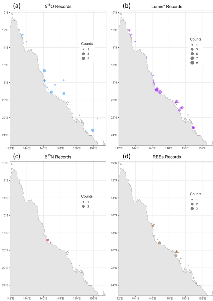
Figure 5. Location map of GBRCD records for (a) \delta^{18}\text{O} , (b) luminescence (Lumin), (c) \delta^{15}\text{N} and (d) Rare Earth Elements (REEs). The size of the point indicates the number of records, and is specific to each map. Note that Lumin* includes all the methods included in the GBRCD for measuring luminescence.
