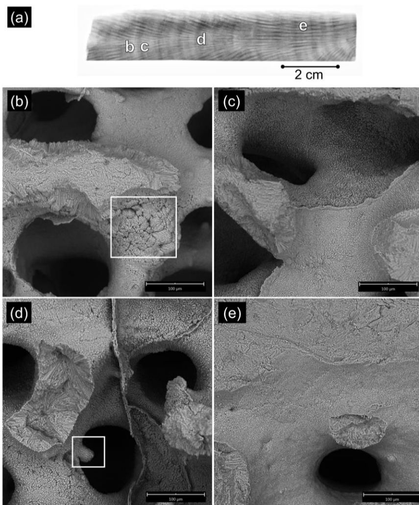
825 Figure C11. OTI4_6C (OTI-4-19; AR24OTI04) SEM images. (a) Approximate locations of SEM images labelled b – e on coral X- ray. (b) to (e) Select SEM images from OTI4_6C (AR24OTI04); (b) 100% cover of secondary aragonite needles generally <10 μm, but section with uneven surface (marked by white box) indicates ~10–20 μm crystals, (c) 100% cover of secondary aragonite needles of <10 μm, (d) 100% cover of secondary aragonite needles of 5–10 μm. Includes secondary aragonite covering likely fungal growth 830 or part of borer tube that occurred when coral was alive (marked by white box), (e) 80% cover of trace (<5 μm) crystals of secondary aragonite. Scale bar indicates 100 μm (b–e).
