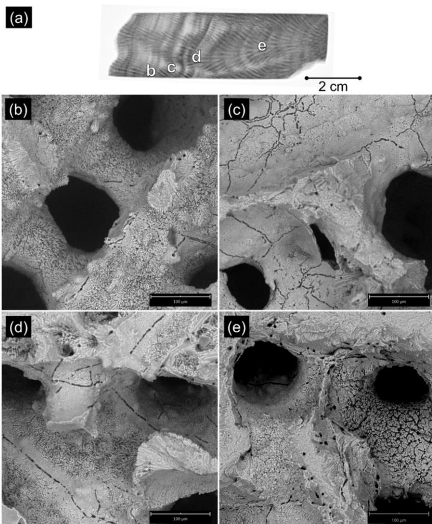
Figure C8. OTI 1-3 (AR24OTI02) SEM images. (a) Approximate locations of SEM images labelled b b - c c on coral X-radiograph. (b) to (e) Select SEM images from OTI 1-3; (b) low-level diagenetic alteration with 100% cover of secondary aragonite needles of 5–15 µm and evidence of micro-borers tracks , (c) No secondary aragonite needles, with evidence of dissolution and micro-borers tracks , (d) Evidence of micro-borers tracks and possibly dissolution. Secondary aragonite needles and calcite crystals (0–10 µm), (e) 90% surface covered by secondary aragonite needles, left side of coral needles are ≤ 5 µm and right side of coral needles are ~5–15 µm. Evidence of micro-borers visible. Scale bar indicates 100 µm (b–e).
