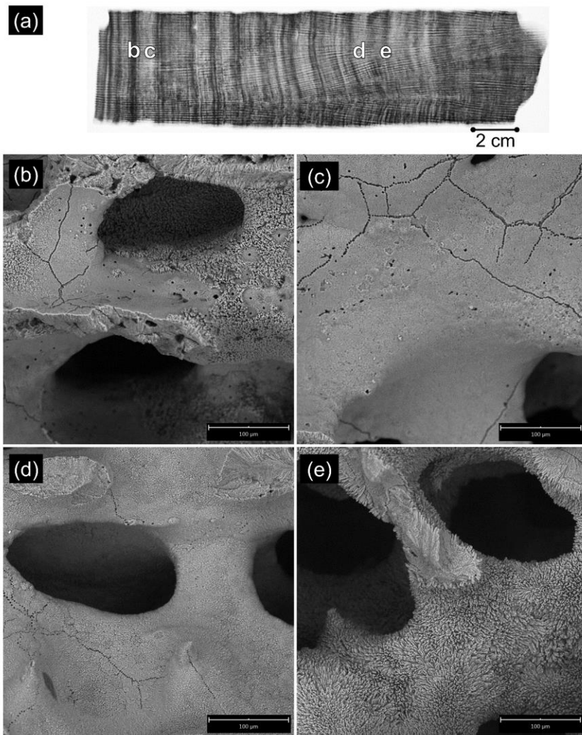
Figure C5. GUT12 (AR24OTI01) SEM images (a) Approximate locations of SEM images labelled b – e on coral X-radiograph. (b) to (e) Select SEM images from GUT12; (b) Secondary aragonite needles \leq 5 \mu\text{m} patchy cover of coral surface (~50%) and evidence of micro-borers, (c) No secondary aragonite needles. Evidence of micro-borers, (d) low-level diagenetic alteration with 100% cover of secondary aragonite needles < 5 \mu\text{m} , (e) low-level diagenetic alteration with 100% cover of secondary aragonite needles of 5-15 \mu\text{m} . Scale bar indicates 100 \mu\text{m} (b-e).
