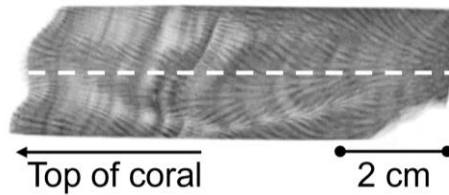
785 Figure C6. X-radiograph (positive) of alternate slice of OTI 1-3 (AR24OTI02) coral. Dashed white line indicates the estimated track analysed by LA-ICP-MS for the record included in AR24OTI02. X-radiographs by PRP Diagnostic Imaging Wollongong.
