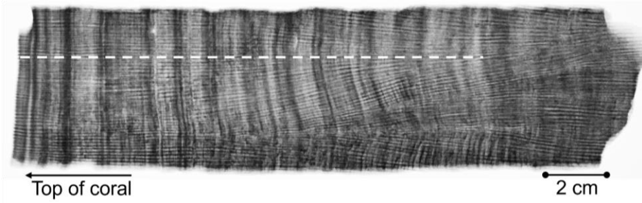
Figure C4. X-radiograph (positive) of GUT12 (AR24OTI01) coral. Dashed white line indicates the track analysed by ICP-AES for the record included in AR24OTI01. X-radiographs by PRP Diagnostic Imaging Wollongong.
