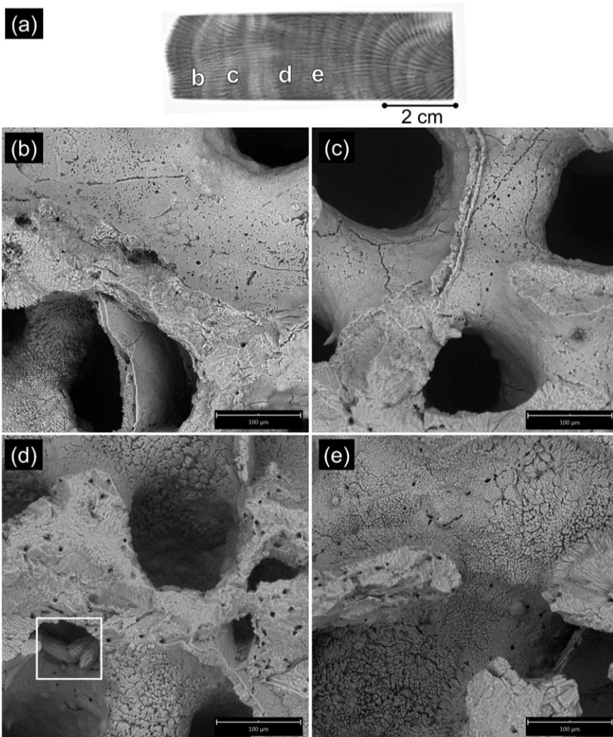
Figure C9. OTI 3-1 (AR24OTI03) SEM images. (a) Approximate locations of SEM images labelled b – e on coral X-ray. (b) to (e) Select SEM images from OTI 3-1; (b) Secondary aragonite needles (0–10 μm) in lower left of image and possible low Mg-calcite cement on coral surface in upper right of image. Evidence of micro-borers, (c) No secondary aragonite. Evidence of micro-borers and possible minor dissolution of coral surface, (d) 100% cover with secondary aragonite needles (0–15 μm) with evidence of micro-borers. High Mg-calcite splays occur in pore space; (marked by white box), (e) 100% cover with secondary aragonite needles (~5–15 μm) with evidence of micro-borers. Scale bar indicates 100 μm (b–e).
