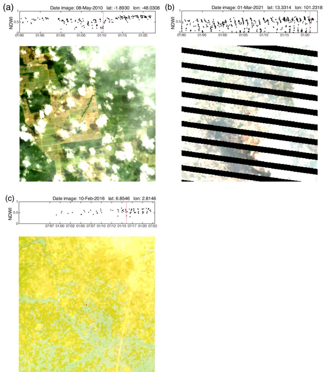
585 Figure A3: Example of the Landsat NDWI time series and the Landsat image that corresponds to the last date of land preparation for three validation points. The NDWI time series corresponds to the pixel located at the center of the image. The images correspond to the last Landsat images classified as bare land using a Random Forest classification. (a) The NDWI time series shows the typical patterns of oil palm development, and the Landsat image corresponds to the land preparation for oil palm. (b) The NDWI time series presents a pronounced seasonality, and the Random Forest classified the low NDWI values as bare land. (c) The NDWI time series presents persistent gaps, and the last observation classified as bare land corresponds to an image largely impacted by cloud 590 cover.
