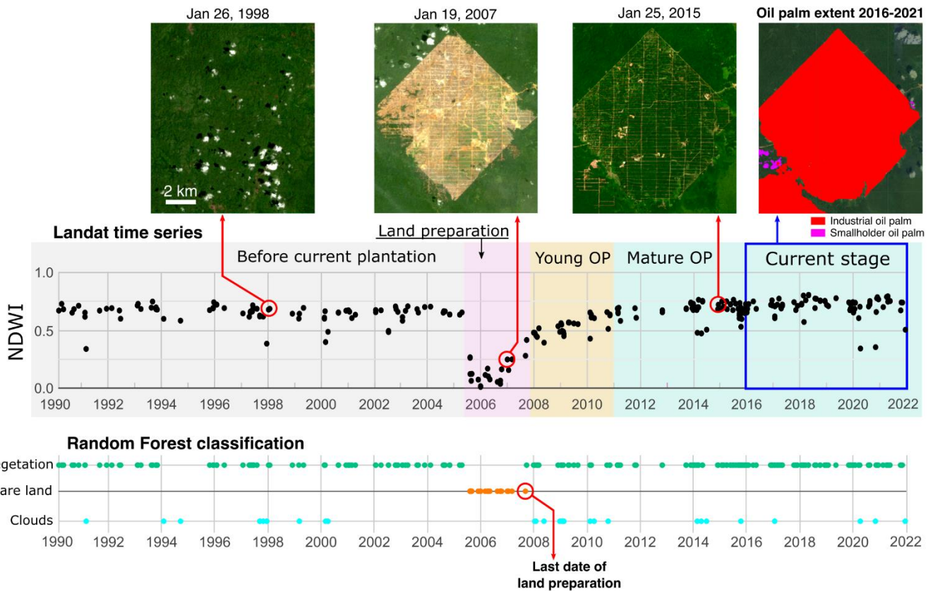
200 Figure 2: Normalized difference water index (NDWI) and classification time series obtained from Landsat-5, -7, and -8 for an industrial oil palm plantation in South Papua, Indonesia. The time series was extracted for a pixel located at the center of the plantation. The upper images illustrate Landsat images for specific dates of the period 1990–2021. The current extent of oil palm was detected using Sentinel-1 data for the period 2016–2021. The Random Forest classified Landsat images into three classes: vegetation, bare land, and clouds.
