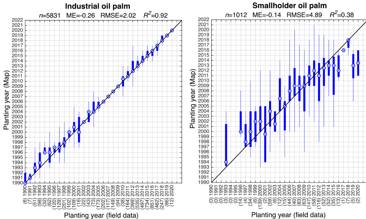
335 Figure 6: Comparison between the planting year obtained from Landsat and the true planting year obtained from field data in a) industrial and b) smallholder oil palm plantations. The title shows the number of observations ( n ), mean error (ME; field data - satellite estimate), root-mean-squared error (RMSE), and coefficient of correlation ( R^2 ). The number of observations from field data for each year appears in parenthesis in the x-axis.
