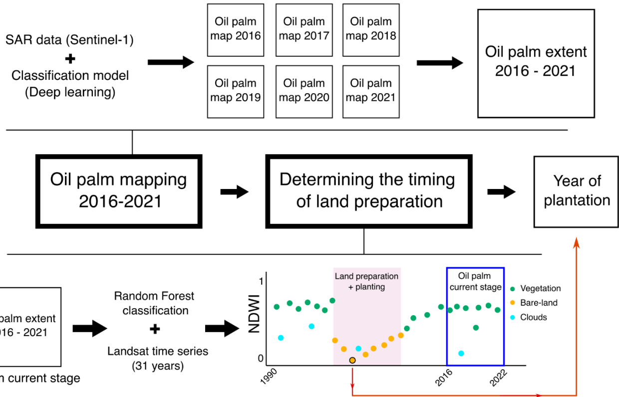
Figure 1: Overview of the three main parts of the methodology for mapping the extent and planting year of oil palm.
