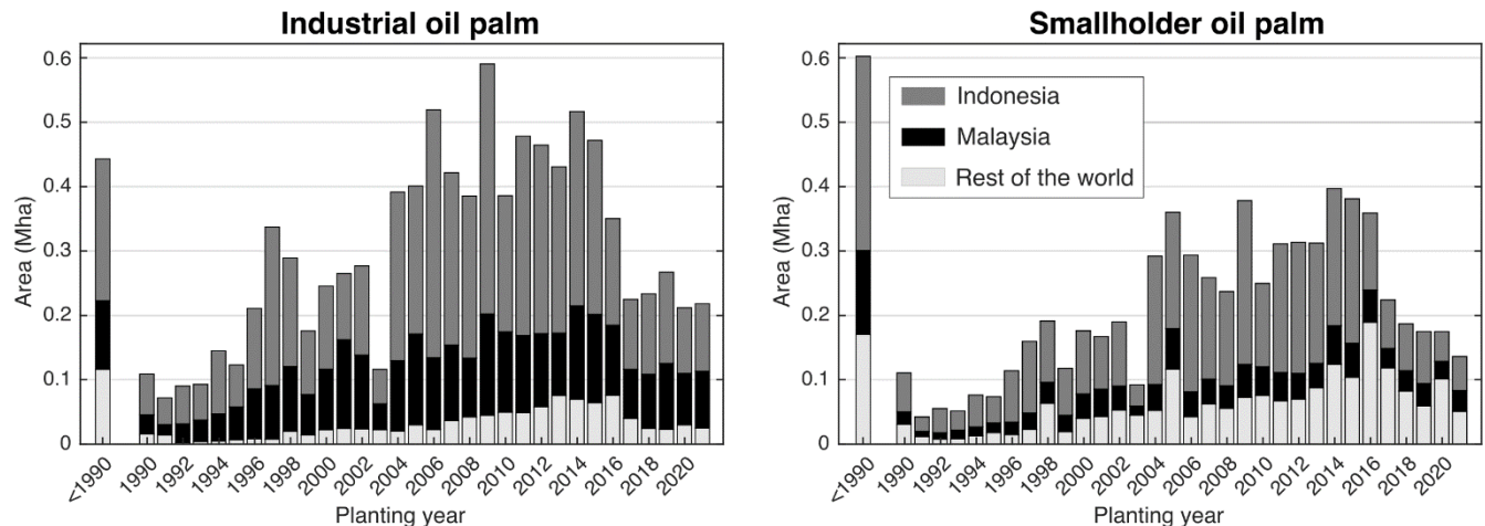
350 Figure 7: Oil palm planting year in industrial and smallholder oil palm for the period 1990–2021 in Indonesia, Malaysia, and the rest of the world. The planting year denotes the time when oil palm was established, either as a new plantation, or through the process of replanting, where old oil palm trees are cleared and replaced by young ones to maintain productivity.
