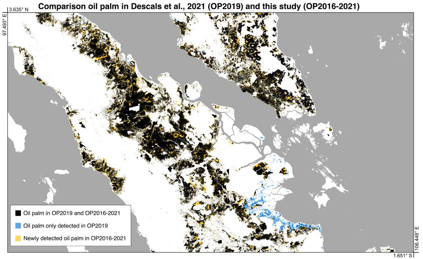
610 Figure A6: Comparison between the oil palm dataset developed by Descals et al. (2021) for 2019 and the oil palm extent layer developed in this study for 2016-2021. Black pixels indicate oil palm detected in both datasets, orange pixels represent newly detected oil palm in this study, and blue pixels correspond to areas detected in 2019 but not included in this study. The orange pixels primarily correspond to young oil palm omitted in the previous version, while the blue pixels mostly consist of false positives in coconut-growing regions.
