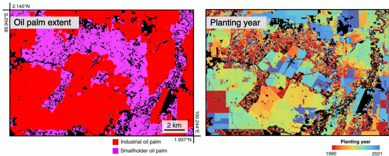
280 Figure 4: Oil palm extent and planting year in a region in North Sumatra, Indonesia. The oil palm extent was obtained from the classification of annual Sentinel-1 composites for 2016–2021. The oil palm age was estimated from the Landsat time series for the period 1990–2021.
