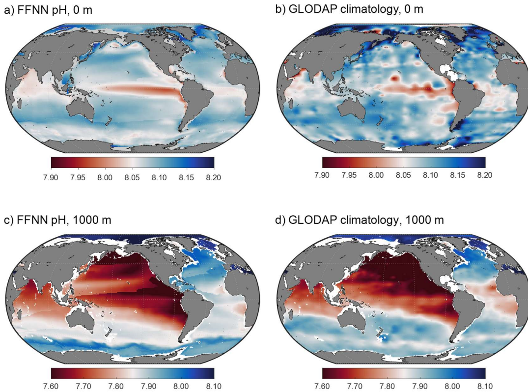
405 Figure 9: Average pH distribution from FFNN pH product and GLODAP climatology normalized to the year 2002. The GLODAP climatology data is from Lauvset et al., 2016.
