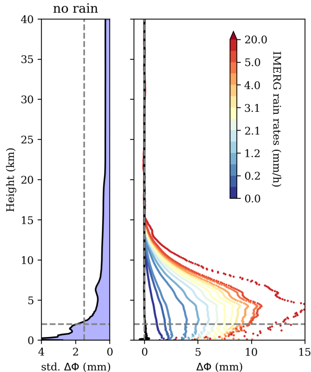
Figure 6. Statistics for the \Delta\Phi profiles. Left panel shows the standard deviation as function of tangent height of the group of \Delta\Phi obtained when P_{\text{IMERG}} = 0 mm/h, representing the free-of-rain cases. Right panel shows the average as function of height of the \Delta\Phi grouped by P_{\text{IMERG}} , when exceeding a certain value indicated in the colorbar. The black line is the average for P_{\text{IMERG}} = 0 mm/h. The horizontal dashed line indicates the 2 km height, and the vertical dashed line indicates the 1.5mm \Delta\Phi standard deviation, which has been taken as reference in previous works (e.g. Cardellach et al., 2014).
