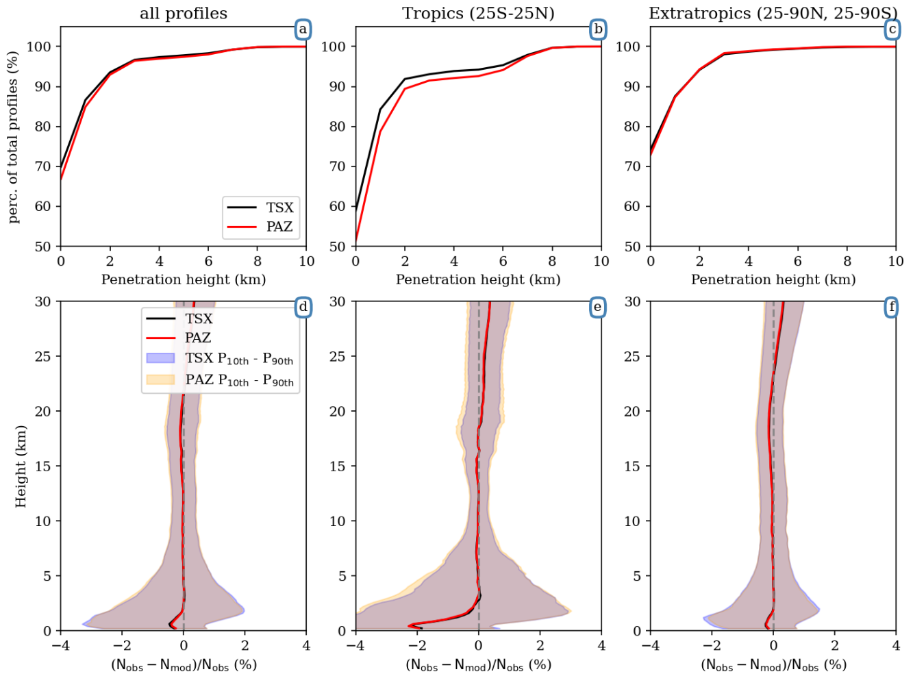
Figure 5. Penetration depth and O-B comparison between TSX and PAZ refractivity retrievals, N , with respect to ECMWF model, for all data between 2019-01-01 and 2019-06-30. Panel (a) corresponds to the percentage of total profiles (y-axis) reaching a certain penetration height (x-axis), for all retrieved data. Panel (b) shows the same as panel (a), but for observations obtained in the Tropics (25S-25N) and panel (c) shows the corresponding results for extratropical cases (25S-90S, 25N-90N). Panel (d) corresponds to the fractional differences (x-axis) as a function of height (y-axis), for all retrieved data. Panel (e) shows the same as panel (d), but for observations obtained in the Tropics (25S-25N) and panel (f) shows the corresponding results for extratropical cases (25S-90S, 25N-90N). The shaded area represent the 10th to 90th percentile of the distribution of fractional differences as function of height.
