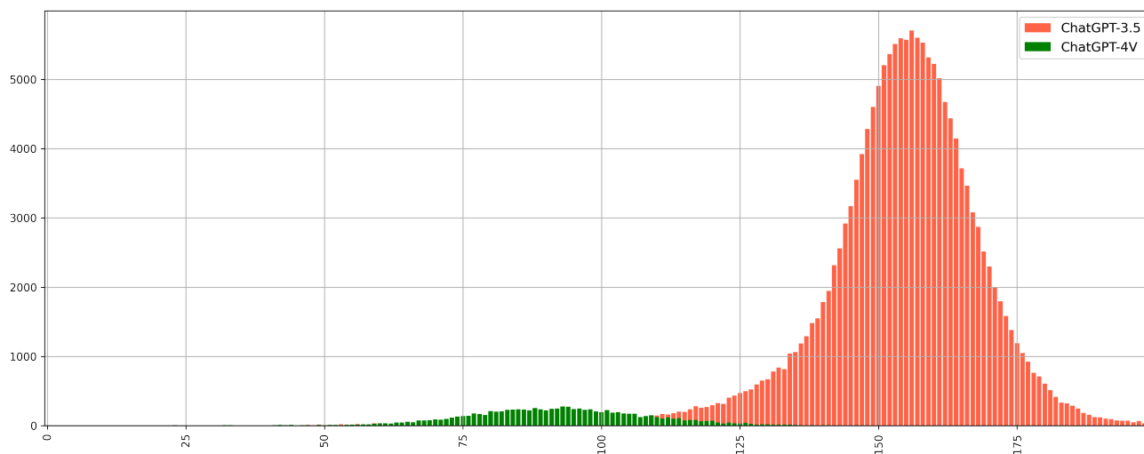
Figure 15. Histogram comparing caption lengths generated by ChatGPT-3.5 and ChatGPT-4V.
