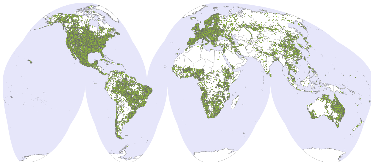
Figure 2. Distribution of sites represented in the 2023 snapshot of WoSIS (Good homolosine equal-area projection).
