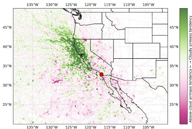
365 Figure 6: ARMTRAJ-ARSCl cloudy (in-cloud deck) and free-tropospheric (above cloud deck) airmass source origin tendency qualitatively demonstrated by the difference between 3-5 day ensemble mean trajectory PDFs. The red marker denotes the EPCAPE main deployment site.
