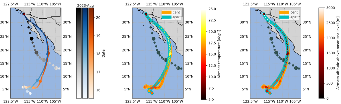
Figure 2: ARMTRAJ-CLD 5-day back trajectory properties of a cloudy layer detected on August 20, 2023, using the 13 UTC sounding measurements (see yellow rectangle in Figure 1). (Left) Airmass trajectory using the ARM deployment coordinates (orange tints), ensemble-mean trajectory (blue shades), and 6-hourly markers of Hurricane Hilary's track (transitioned to a tropical storm on August 20; grey tints). (Middle) The same trajectories overlaid with hourly airmass temperature and (right) altitude AMSL. Larger markers denote 24-hour increments from the trajectory initialization time. The red marker designates the ARM ECAPE deployment site.
