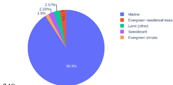
Figure 5: ARMTRAJ-PBL bulk analysis of average surface and vegetation properties overpassed by ECAPE PBL airmasses (see text).
