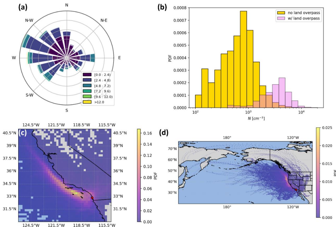
Figure 4: ARMTRAJ-SFC bulk analysis: (a) Wind rose based on hourly-mean data from the ARM Surface Meteorology System (legend values are in m/s), (b) sub-micron total number concentration histogram (logarithmic bin width of 0.121) using SMPS data partitioned based on whether 12-36 hour surface back trajectories had any land overpass (see text), (c) probability density function of 12-36 hour back-trajectory samples (bin dimensions of 0.25×0.25 degrees), and (d) same, but for 48-96 hour back-trajectories.
