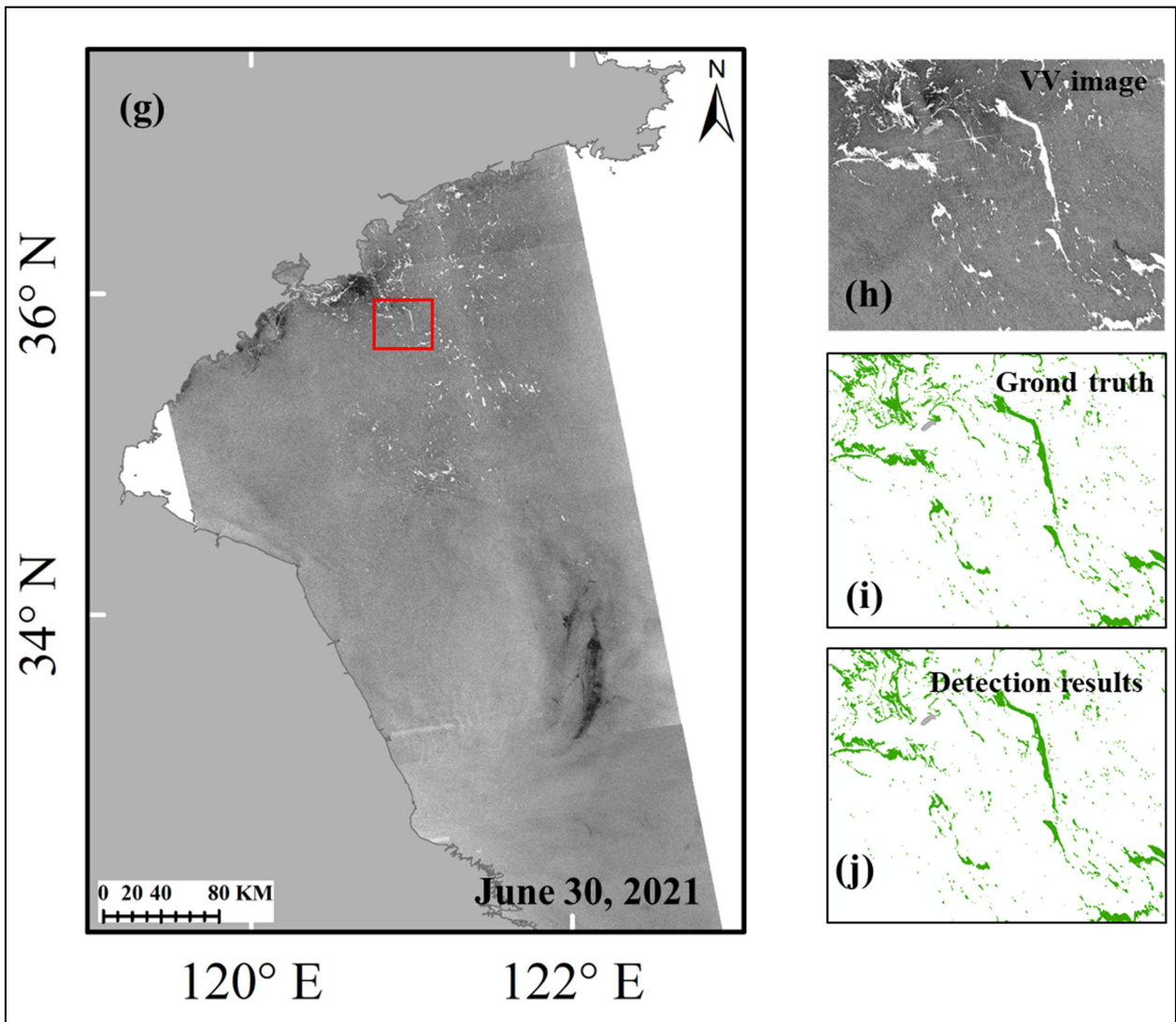
375 Figure 12. Randomly selected SAR image detection results for the Subei Shoal (a-f) and the entire Yellow Sea (g-j) regions on June 22, 2018, and June 30, 2021.
