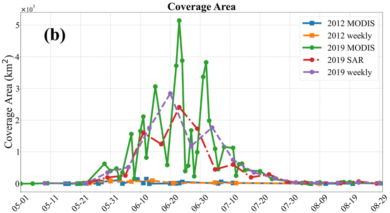
445 Figure 15. (a) Time series of the green tide's maximum daily and weekly coverage area from 2008 to 2022. The numbers on the subfigure represent the corresponding observation cycle date and the week to which the fusion product belongs. (b) Daily and weekly green algae coverage throughout the entire life cycle in 2012 and 2019.
