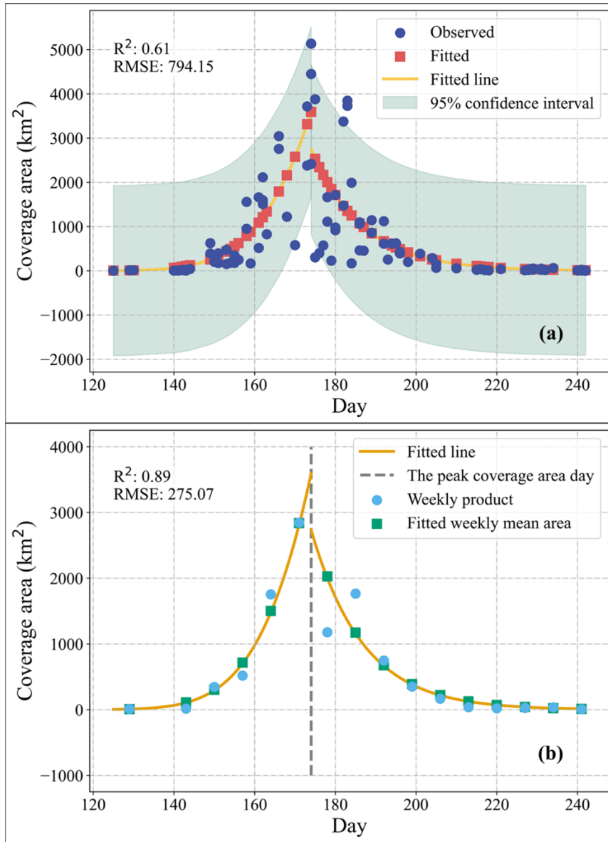
410 Figure 13. Uncertainty assessment of green tide products based on green tide outbreak pattern (2019). (a) Uncertainty in daily product and (b) Uncertainty in weekly product.
