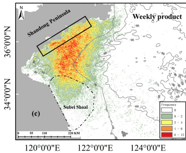
420 Figure 14. Green tide distribution hotspot map obtained from daily optical (a) and SAR (b) products, and weekly products (c).
