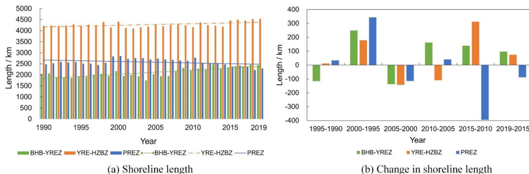
Figure 6: Regional shoreline length and change from 1990 to 2019.
