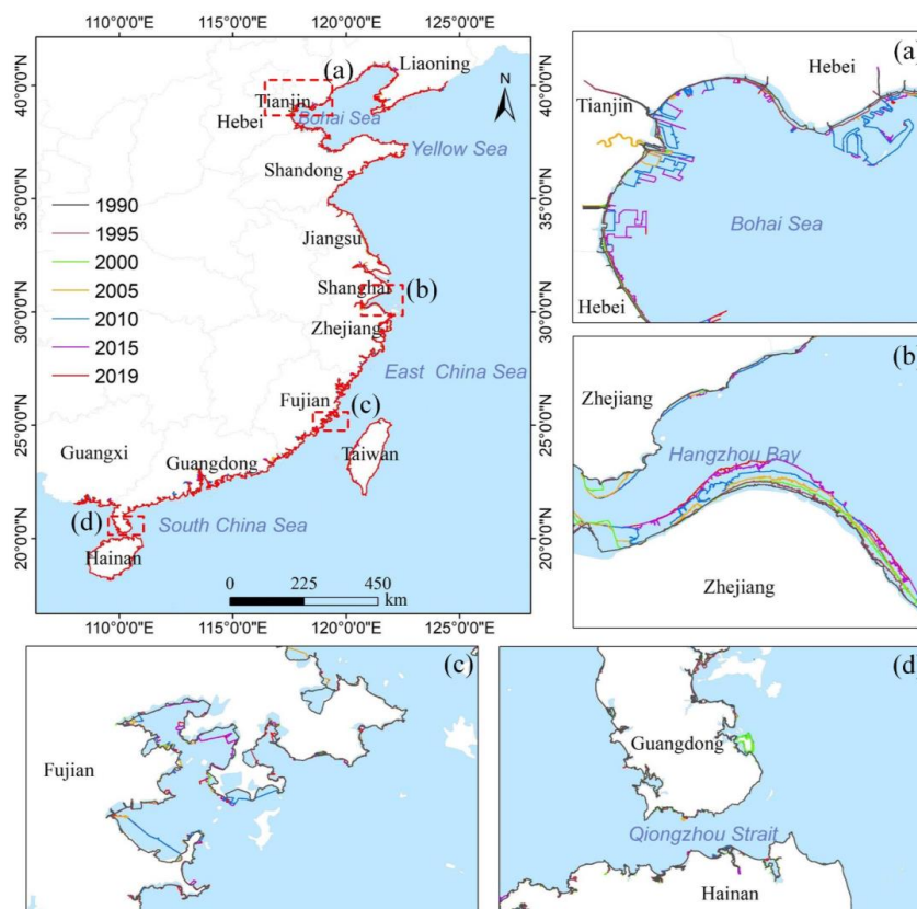
225 Figure 4: Spatial distribution of the shoreline during the study period from 1990 to 2019.
