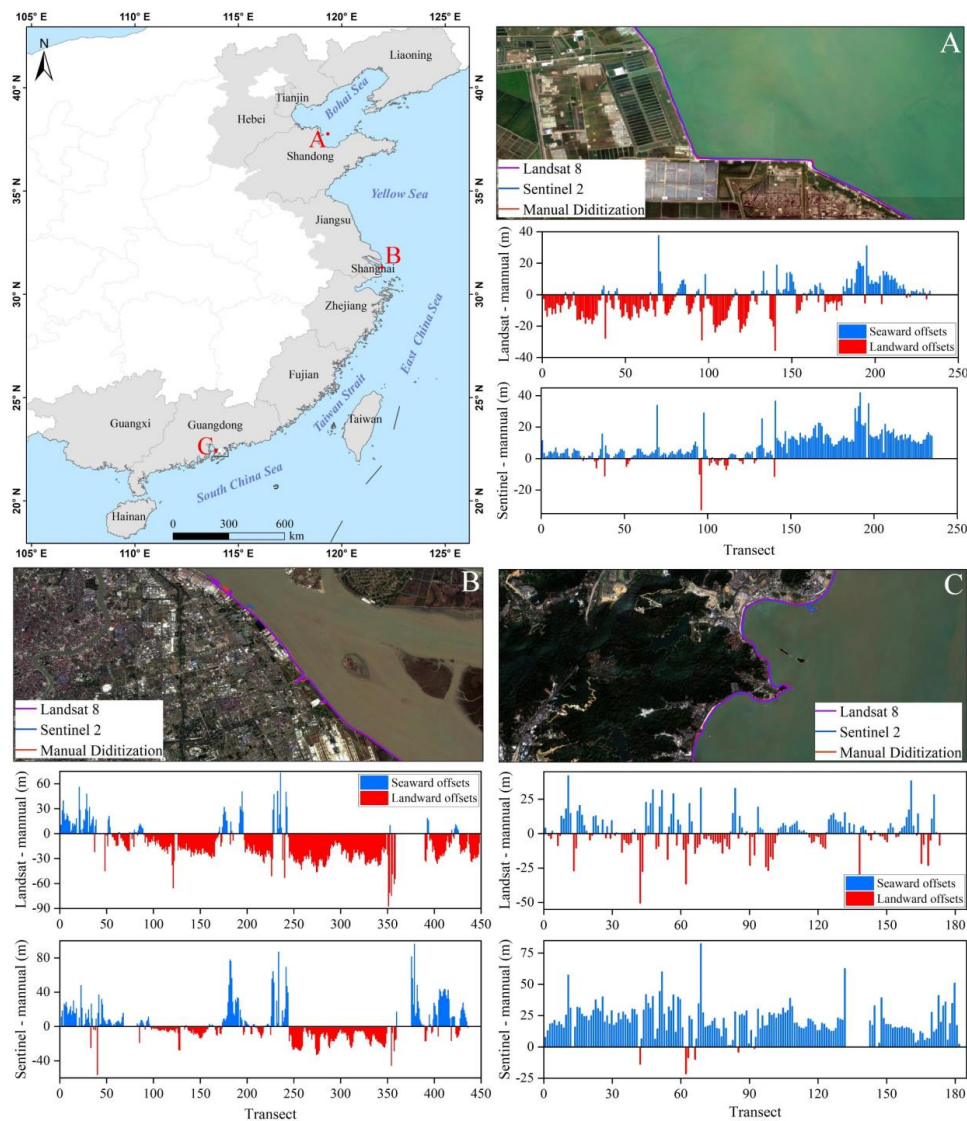
440 Figure 14: Comparison between the L8, S2, and the corresponding results of manual digitization. (A), (B), and (C) are the difference between L8, S2, and manual digitization. ME and MAE are mean error and mean absolute error respectively.
