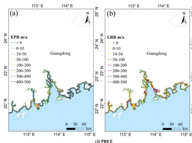
Figure 8: Map of shoreline change rate in three regions from 1990 to 2019: (1) BHB-YREZ; (2) YRE-HZBZ; (3) PREZ. (a) EPR, (b) LRR.
