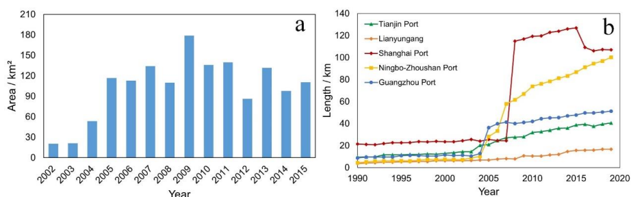
340 Figure 10: (a) Reclamation in China from 2002 to 2015; (b) Length of main coastal ports above the designated size from 1990 to 2019.
