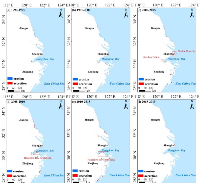
Figure 12: Area and locations of land erosion and accretion in the YRE-HZBZ.
