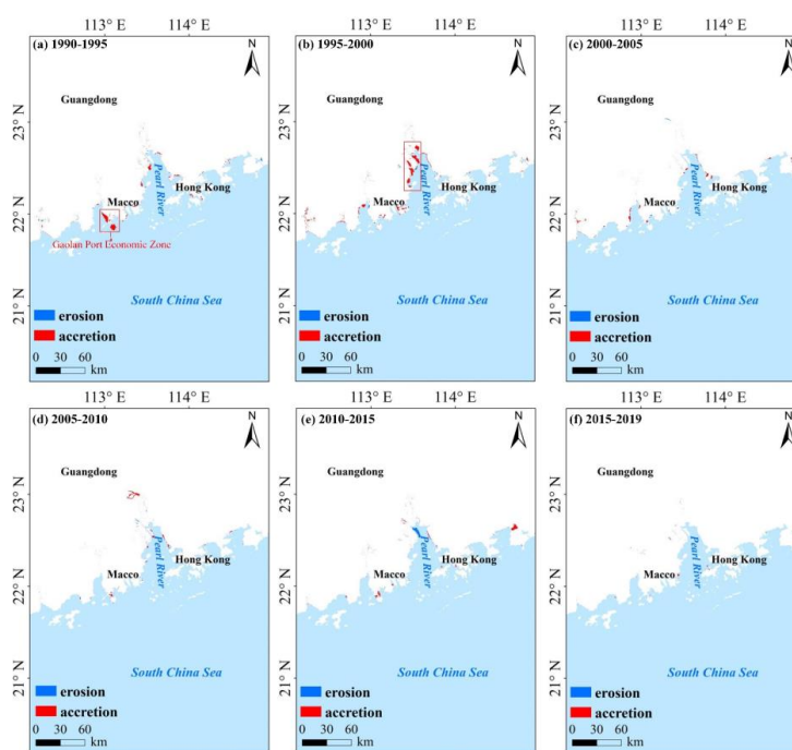
395 Figure 13: Area and locations of land erosion and accretion in PREZ.
