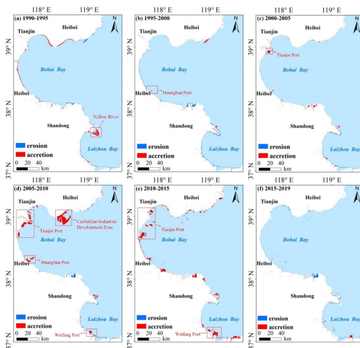
Figure 11: Area and locations of land erosion and accretion in the BHB-YREZ.
