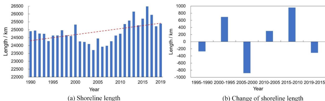
Figure 5: Length and change of China's shoreline from 1990 to 2019.
