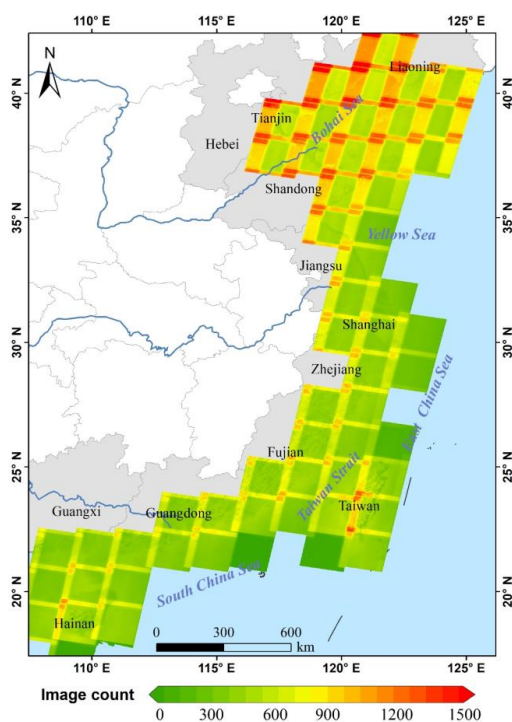
Figure 2: Landsat TM/ETM+/OLI images coverage of good-quality observations from 1990 to 2019.
