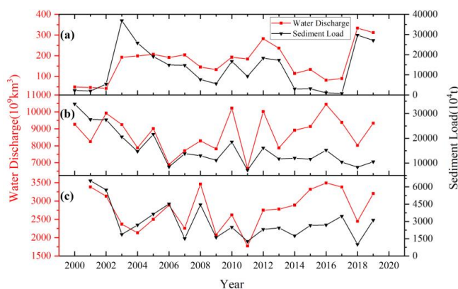
310 Figure 9: Annual water discharge and annual sediment load. (a) Lijin Hydrometric Station from 2000 to 2019; (b) Datong Hydrometric Station from 2000 to 2019; (c) Gaoyao, Shijiao, and Boluo Hydrometric Stations from 2001 to 2019.
