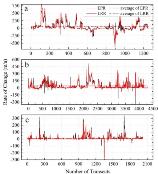
Figure 7: Change rate of shorelines over BHB-YREZ (a), YRE-HZBZ (b), and PREZ (c) from 1990 to 2019.
