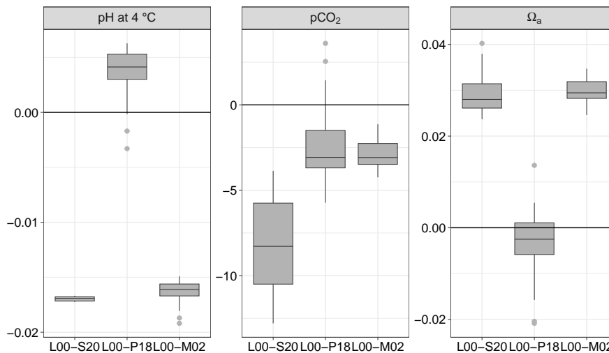
Figure 4. pH normalised at 4 °C, partial pressure of CO 2 and saturation state of aragonite \Omega_a calculated from A_T and A_T - C_T (115 data pairs): differences between the formulations for K_1 and K_2 of Lueker et al. (2000, L00) and those of Sulpis et al. (2020, S20), Papadimitriou et al. (2018, P18) and Millero et al. (2002, M02). Units for pCO 2 is \mu\text{atm} .
