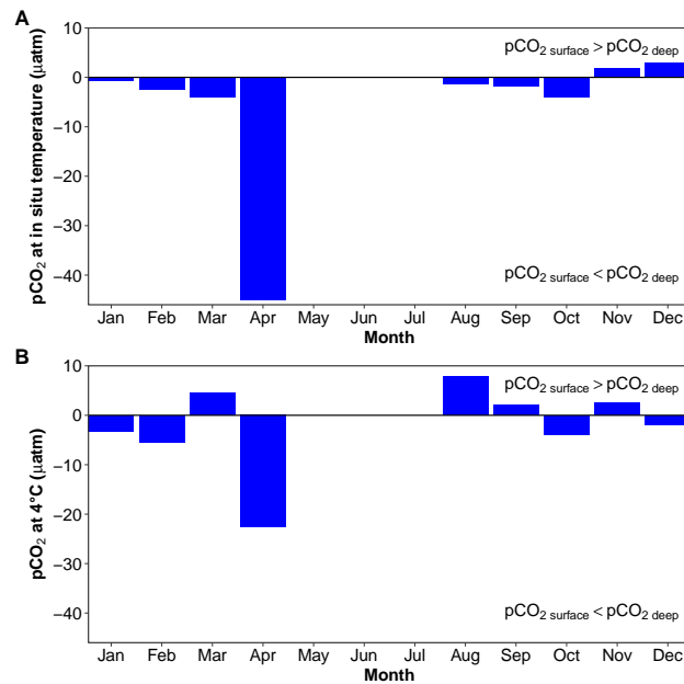
Figure 9. Vertical gradients estimated using the median monthly values of pCO 2 at in situ hydrostatic pressure, calculated from A_T (using the A_T vs S relationship) and SeaFET pH _{T-T} using the R package seacarb (?) (Gattuso et al., 2023b). A: CO 2 at in situ temperature; B: pCO 2 normalised at 4 °C. “Surface” is 0 to 4 m while “deep” is 8 to 12 m. Data are missing in May to July because no surface pH data is available during this period.
