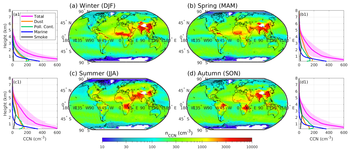
Figure 4. Seasonal climatology of n_{CCN} at a supersaturation of 0.20% and at altitudes below 2 km for winter (a), spring (b), summer (c) and autumn (d). The vertical variations in seasonal n_{CCN} is depicted in the adjacent sub-panels for dust (orange line), polluted continental (green line), marine (blue line), and smoke (black line) aerosol types. Magenta profile in the sub-panels represent the total n_{CCN} and the semi-transparent patch highlights the associated standard deviation scaled to half of its original value for better visualization.
