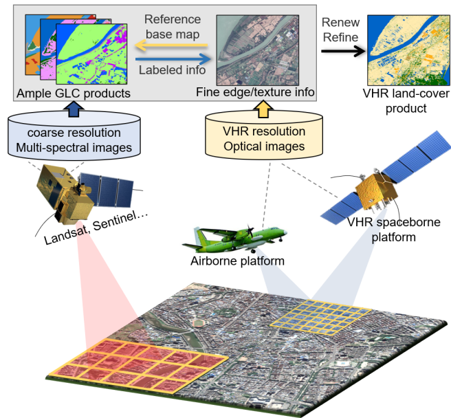
Figure 1. Demonstration of using the fine edge and texture information from VHR images to renew and refine the current ample coarse-resolution GLC products. The VHR remote sensing images in the figure are from © Google Earth 2021.
