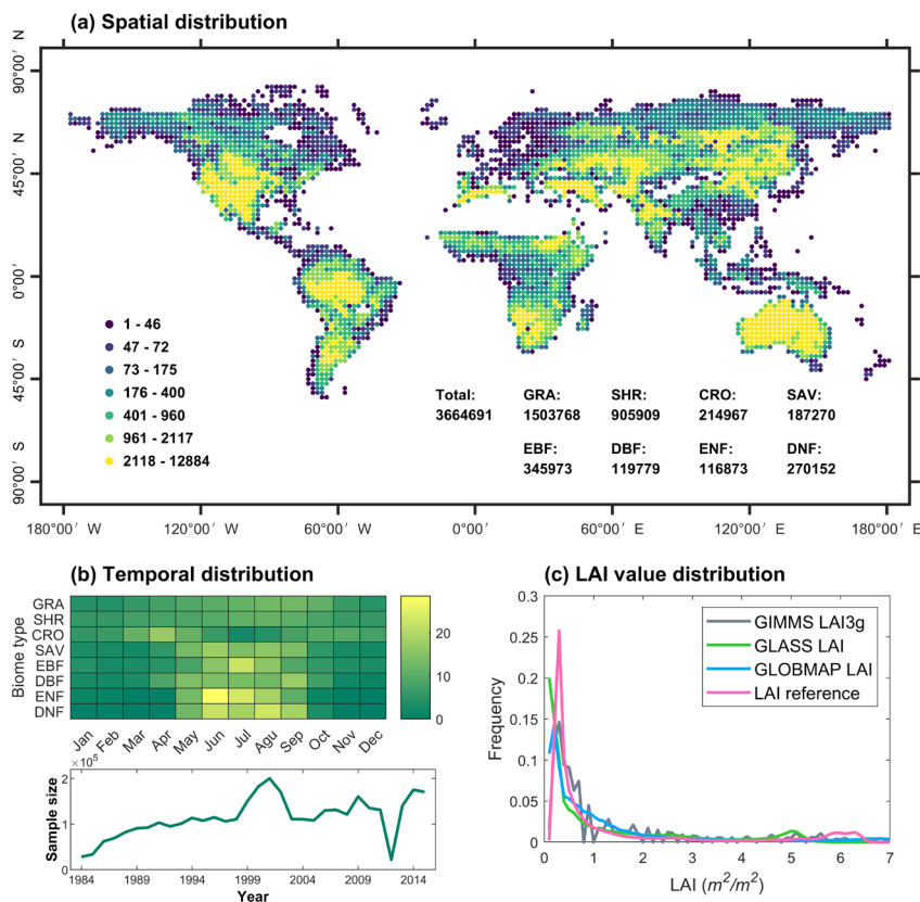
Figure 2. Spatial and temporal distribution of the LAI reference data. (a) The global distribution of LAI samples in 2° grids. The LAI sample size for each vegetation is listed. (b) The temporal distribution of LAI samples for the eight vegetation biome types and the annual variation of LAI sample size. (c) The distribution of LAI values in percentage (bin width = 0.1) for Landsat LAI samples, GIMMS LAI3g, GLASS LAI, and GLOBMAP LAI. For GIMMS LAI3g, GLASS LAI, and GLOBMAP LAI, the value distribution was calculated based on all terrestrial vegetation pixels. It should be noted that 40,000 Reprocessed MODIS LAI samples were introduced at locations and months when Landsat LAI samples were scarce.
