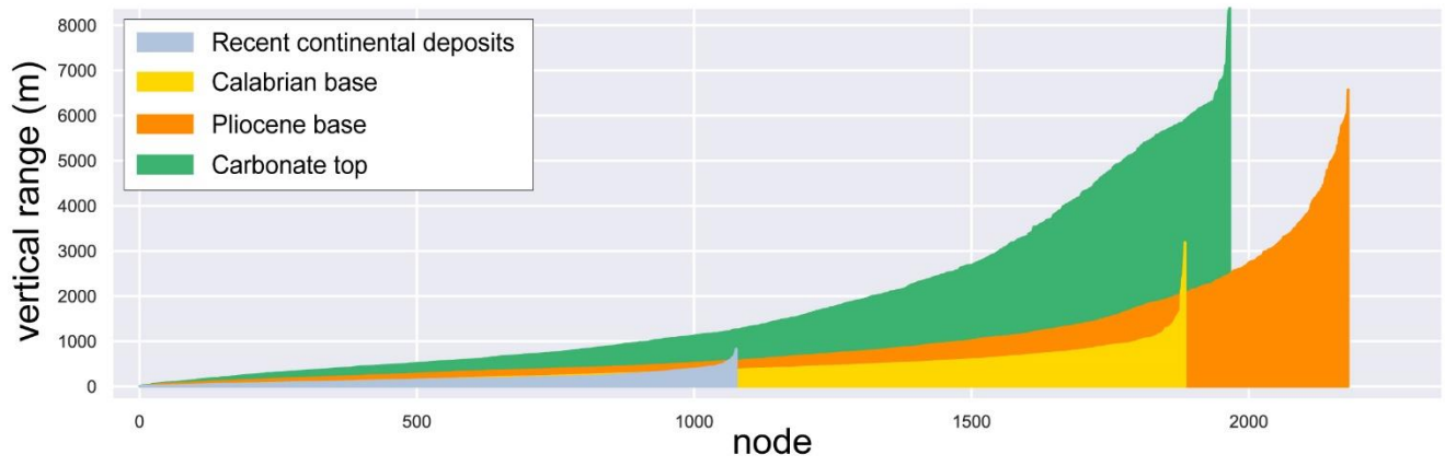
535 Figure 12: Range of depths variation interpolated at each point of the evaluation grid based on the different datasets available for the four surfaces.
