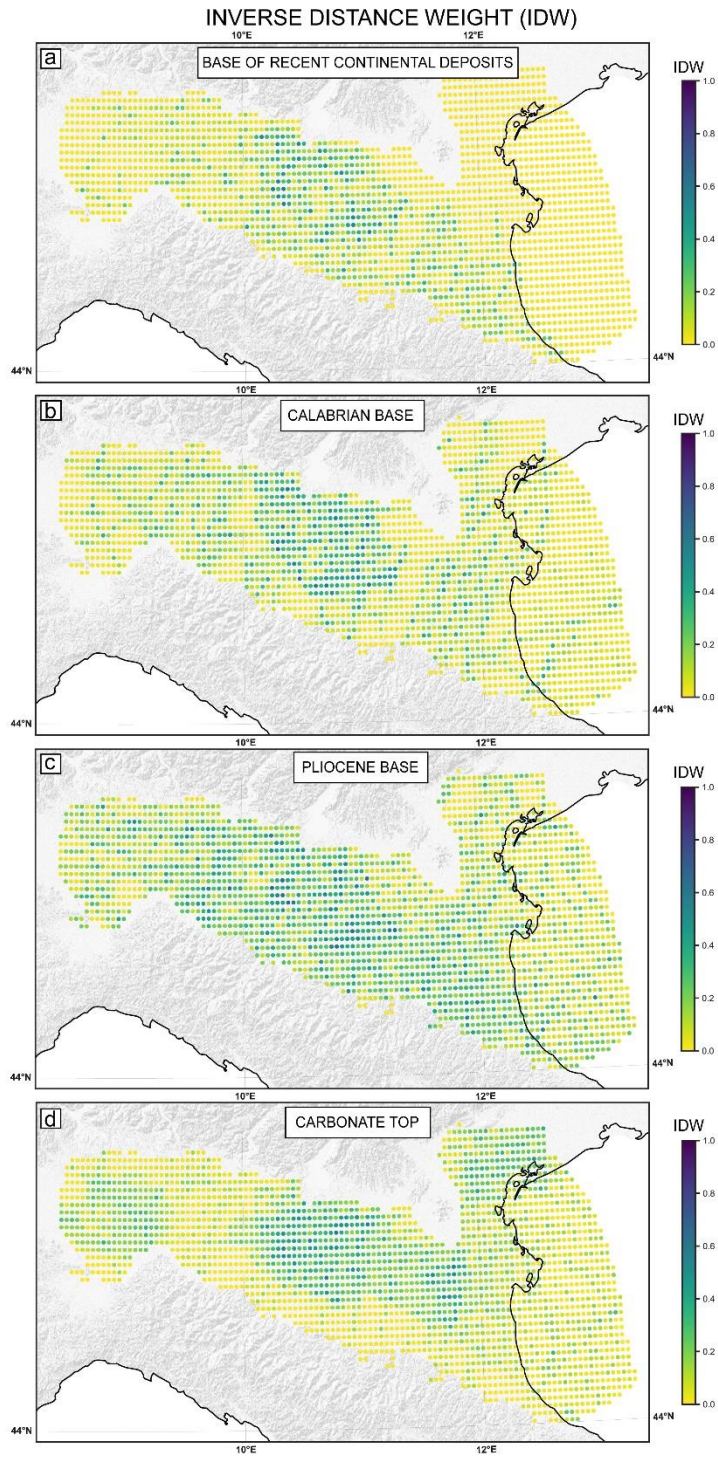
Figure 11: The spatial distribution of the IDW for the four analysed surfaces. The IDW values represent the confidence on the variable of interest (level depth) at each node of the grid (1 = max confidence).
