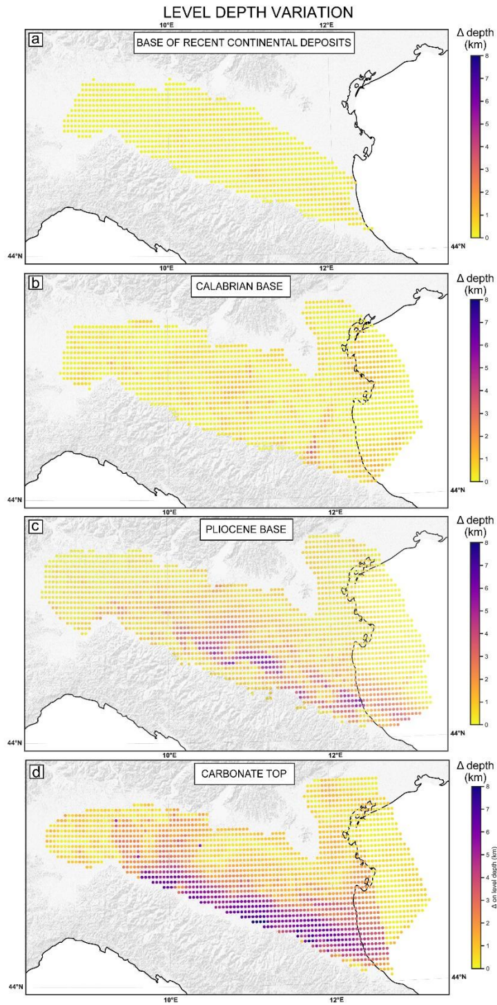
Figure 13: Geographic distribution of the range of depths variation for the four analysed surfaces
