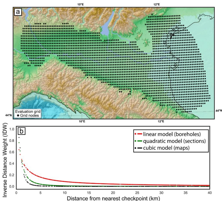
475 Figure 9: a) Grid-nodes used to evaluate the data accuracy and uncertainties for geological surfaces presented for the study area. At each node, based on spatial autocorrelation, we calculated the Inverse Distance Weight (IDW) with respect to points observation (checkpoints). b) The model adopted for the IDW describes how uncertainties increase moving away from the best guess at checkpoints (i.e., at well, along geologic cross-sections or on depth maps); at the same distance from a checkpoint, well data gives higher IDWs (red points) with respect to data derived from geological cross-sections or interpolated maps (green and black points).
