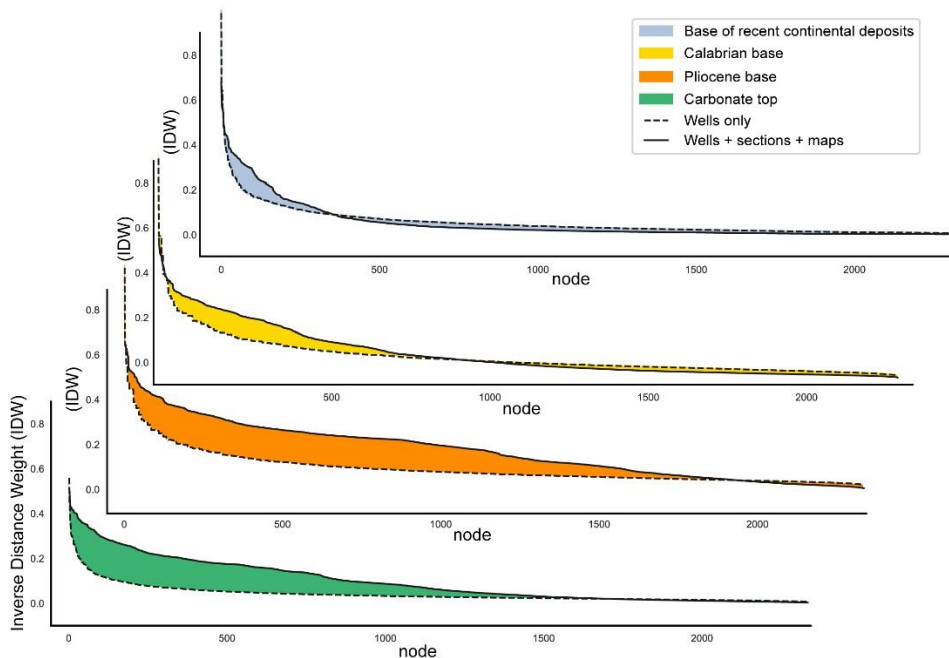
510 Figure 10: IDW values at grid nodes calculated for each surface considering distances from well data only (dashed lines) or integrating distances from well data plus geological cross-section plus geological maps (solid lines). The area between the two lines for each proposed surface is larger for greater uncertainties. Note that the uncertainties increase with the depth of the surfaces and that the total number of checkpoints does not always increase the confidence level of the data (as for example in the recent continental deposits).
