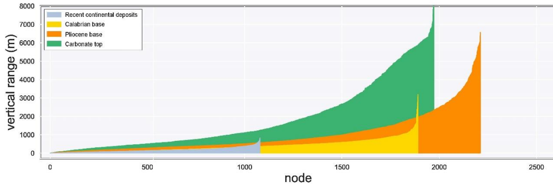
535 Figure 12: Range of depths variation interpolated at each point of the evaluation grid based on the different datasets available for the four surfaces.
