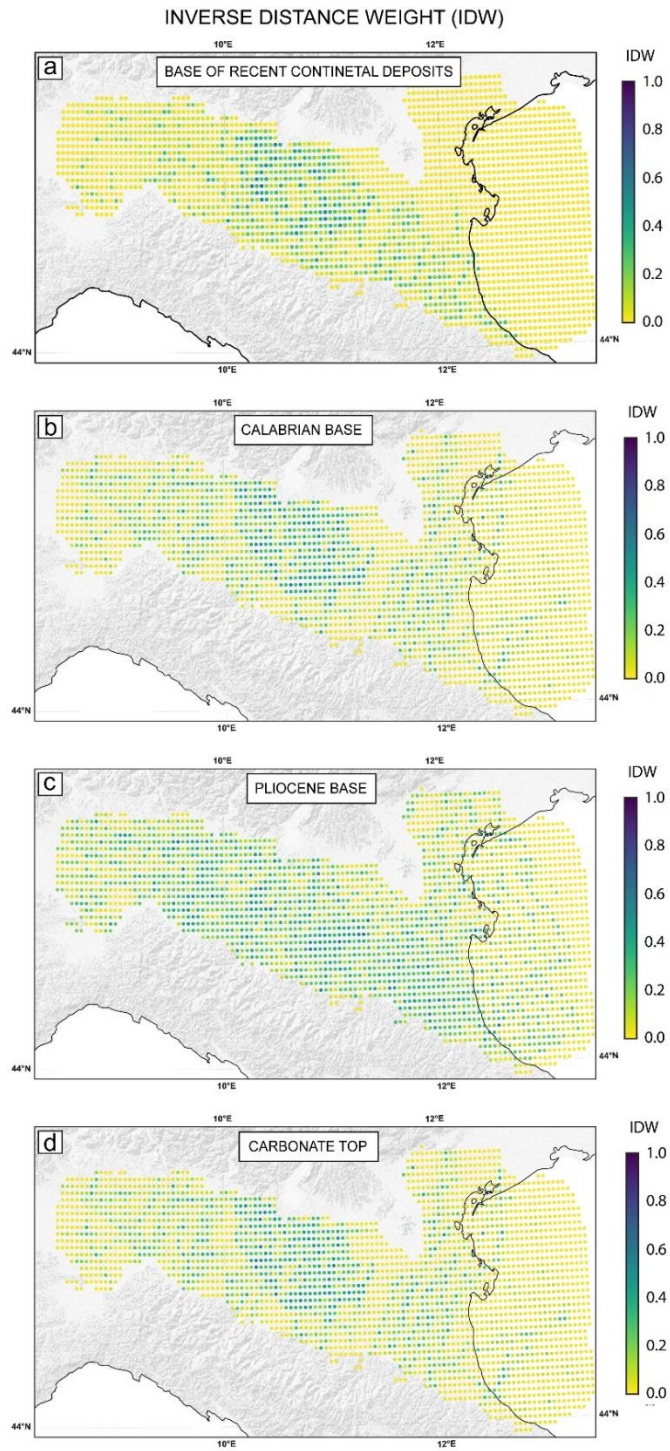
530 Figure 11: The spatial distribution of the IDW for the four analysed surfaces. The IDW values represent the confidence on the variable of interest (level depth) at each node of the grid (1 = max confidence).
