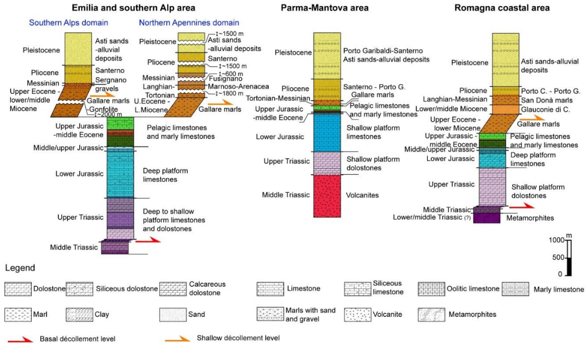
185 Figure 3: Synthetic stratigraphic columns of the Po Plain. From left to right: the stratigraphy of Emilia and Southern Alps, Parma-Mantova, and Romagna coastal areas is shown (see Fig. 2a). The carbonate passive margin (from violet to green colours) and silicoclastic active margin (from brown to light yellow colours) sequences are distinguished. The main décollement levels are highlighted (red for basal décollement and orange for shallow décollement). The stratigraphic column to the left shows the different filling and the different formation thickness of the Southern Alps and the northern Apennines foredeep. 190
