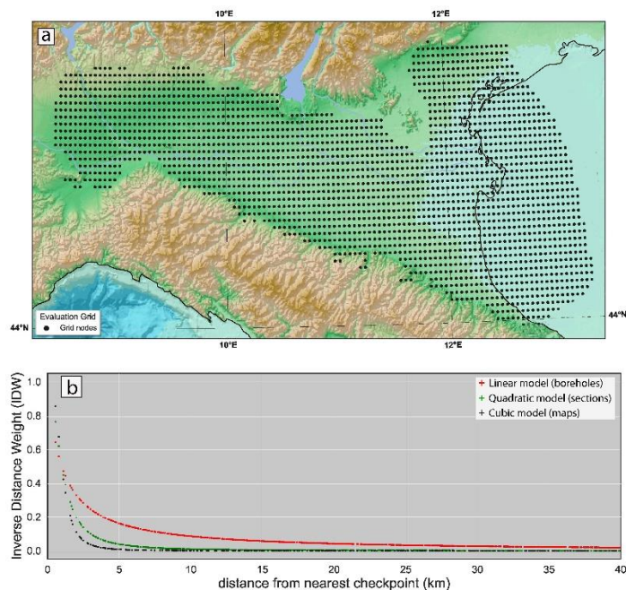
475 Figure 9: a) Grid-nodes used to evaluate the data accuracy and uncertainties for geological surfaces presented for the study area. At each node, based on spatial autocorrelation, we calculated the Inverse Distance Weight ( IDW ) with respect to points observation (checkpoints). b) The model adopted for the IDW describes how uncertainties increase moving away from the best guess at checkpoints (i.e., at well, along geologic cross-sections or on depth maps); at the same distance from a checkpoint, well data gives higher IDW s (red points) with respect to data derived from geological cross-sections or interpolated maps (green and black points).
